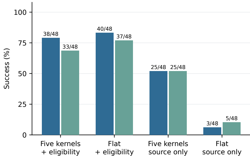
Counterfactual pair success
