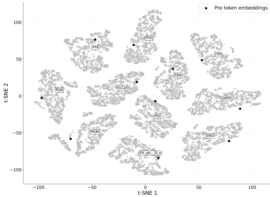
Figure 4.7: t-SNE projection of glycolysis reaction embeddings in the E. coli core model. Gray points show final layer embeddings across sampled nutrient compositions. Black points show the learned initial reaction embeddings before Transformer processing.
