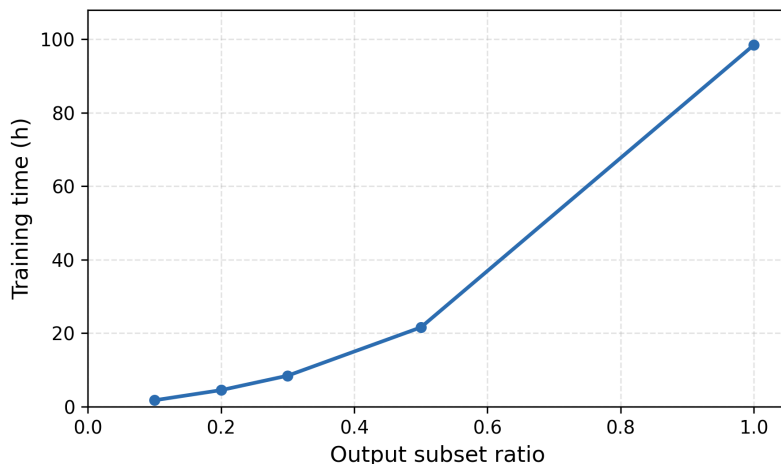
Figure 4.12: FluxTransformer training time for Yeast9 at different output subset ratios using 250,000 simulated samples.
