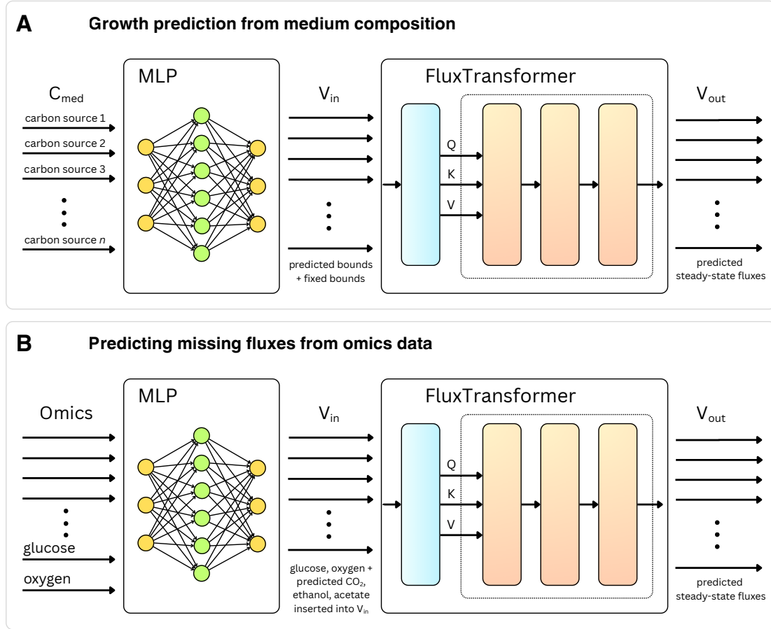
Figure 3.4: Experimental prediction pipelines using a pretrained FluxTransformer. (A) In growth prediction, the medium-composition vector C_{med} is mapped by a multilayer perceptron (MLP) to V_{in} , the uptake-bound input vector for the FluxTransformer. The model predicts V_{out} , and the biomass reaction in this flux vector is compared with measured growth. (B) In missing-flux prediction, transcriptomic and proteomic measurements are combined with glucose and oxygen uptake. The MLP predicts missing exchange constraints for CO_2 , ethanol, and acetate, which are used as inputs to the frozen FluxTransformer and downstream pFBA evaluation.
