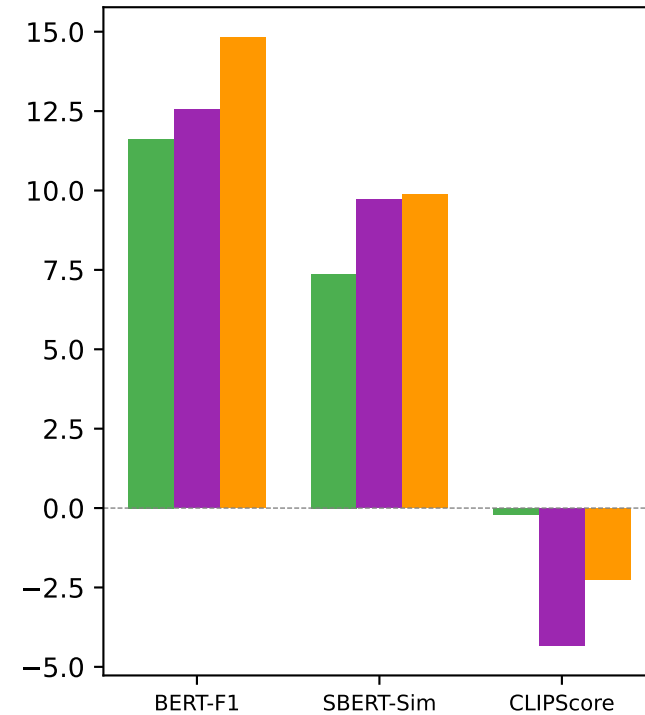
InternVL2.5-26B
