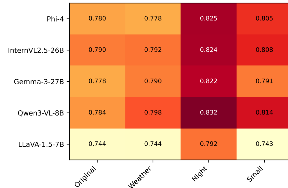
CLIPScore
