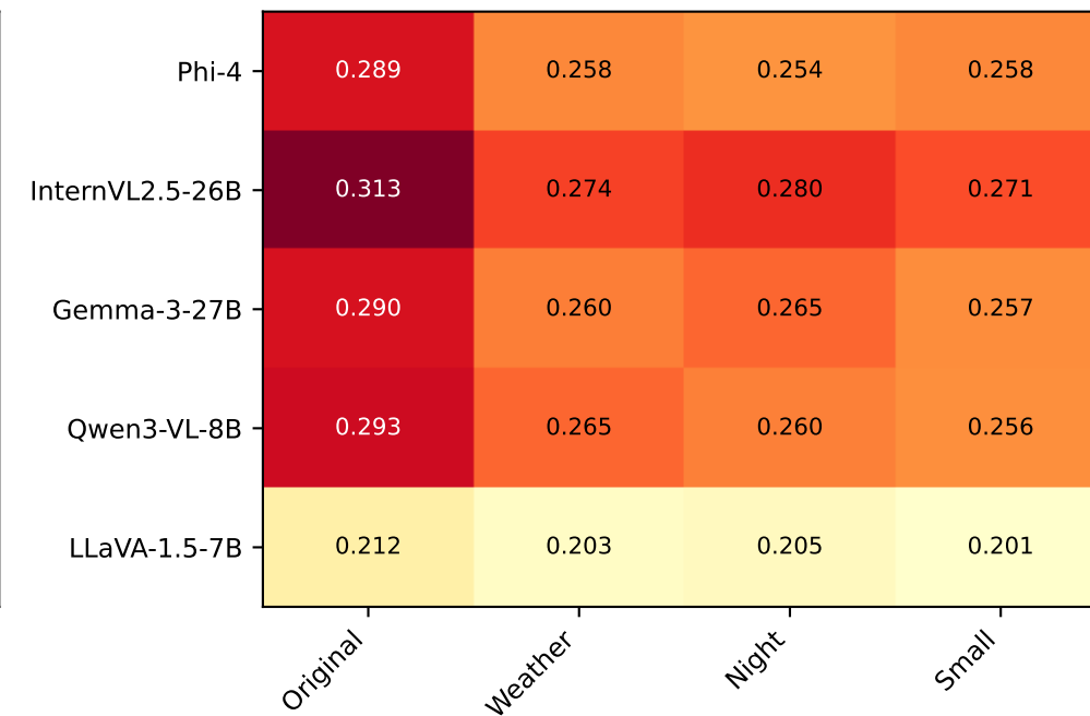
METEOR
