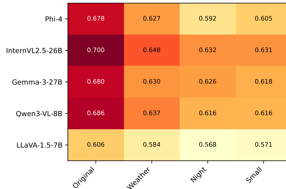
SBERT-Sim
