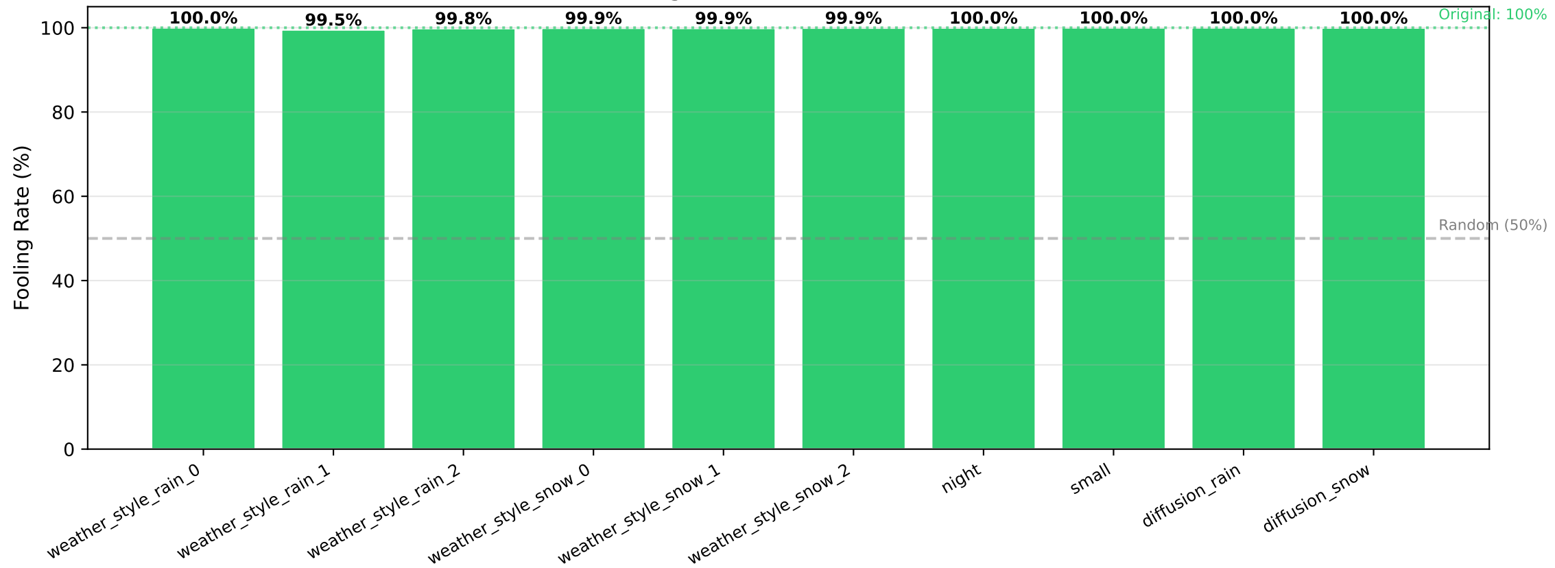
AI Detector Fooling Rate per Augmentation Condition (Higher = More Realistic)
