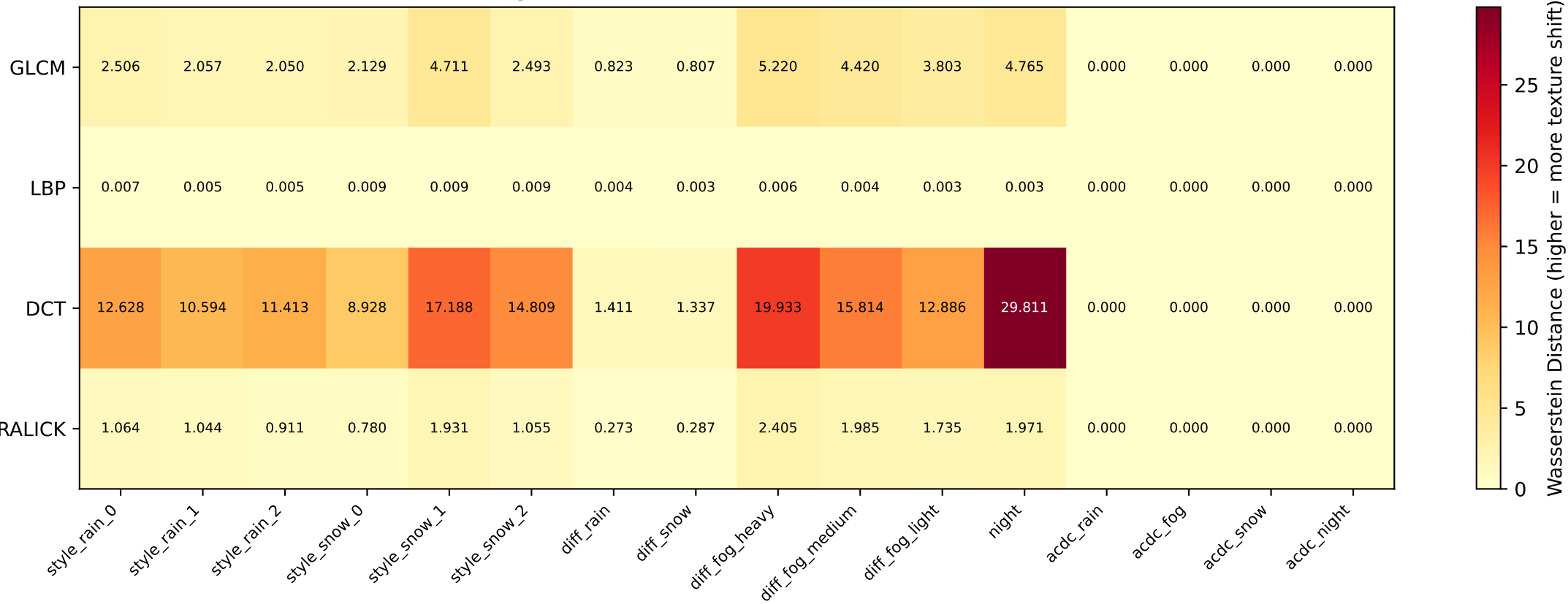
Texture Feature Distribution Shift: Augmented vs Original (per-feature Wasserstein distance)
