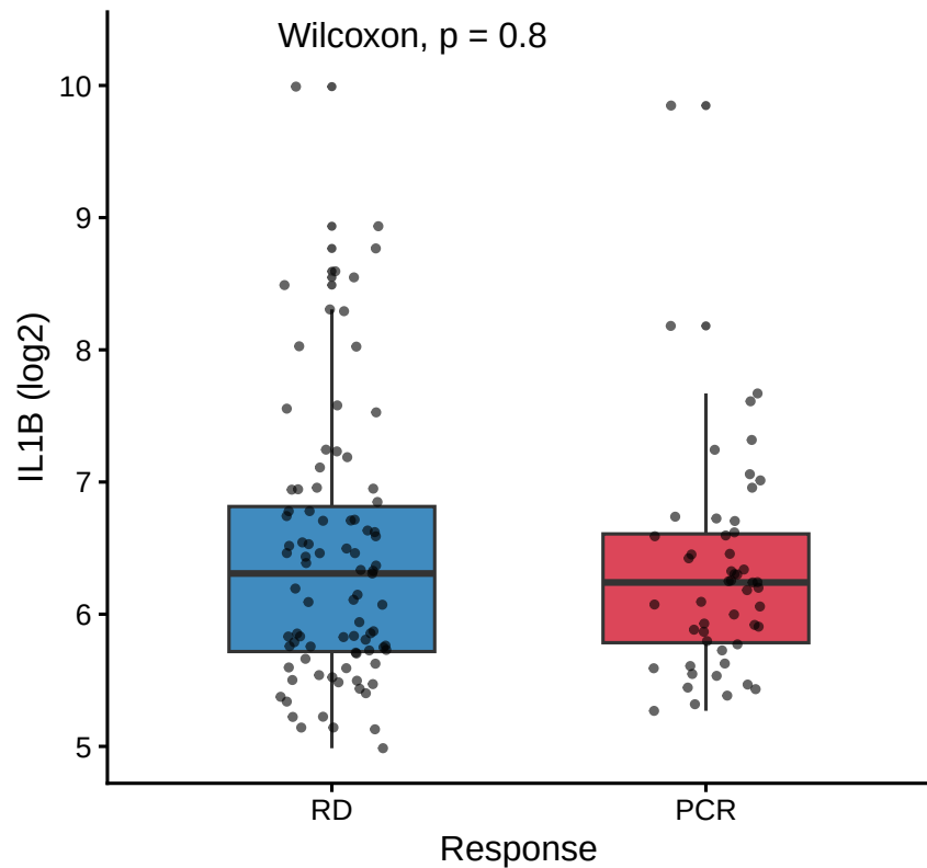
B IL1B in GSE41998 TNBC
