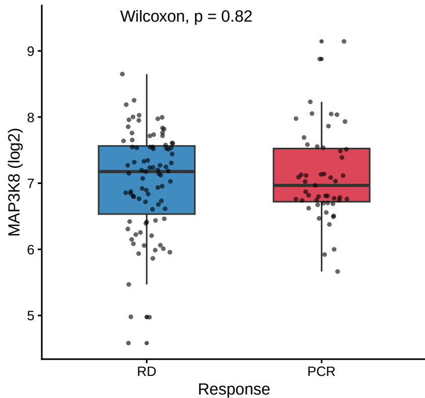
A MAP3K8 in GSE41998 TNBC
