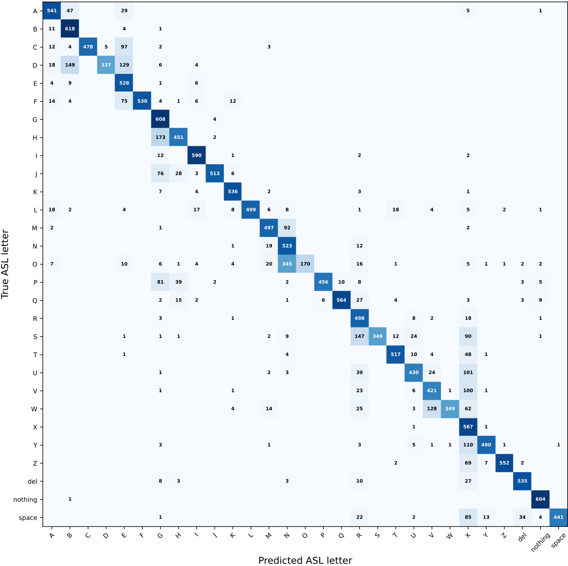
Final Validation Confusion Matrix
