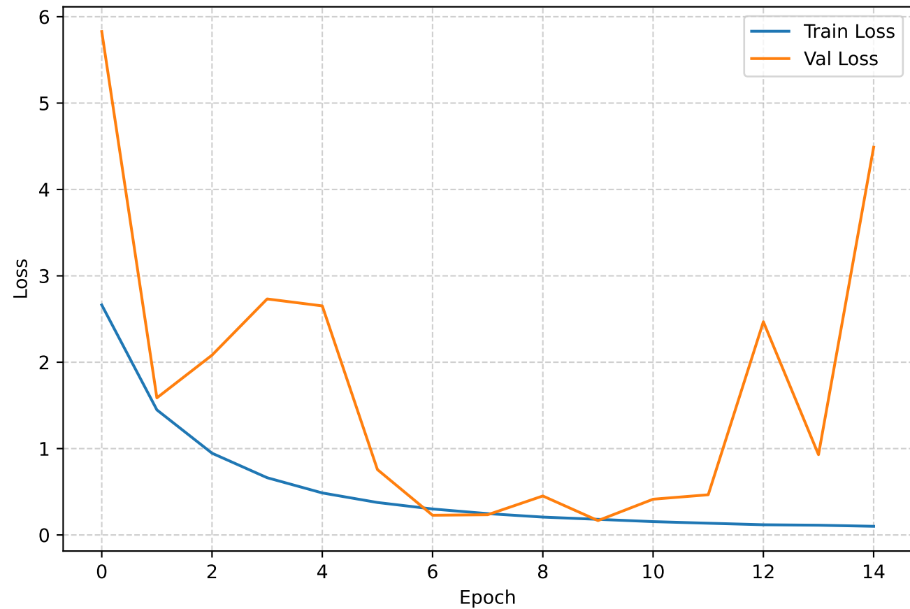
Model Loss
