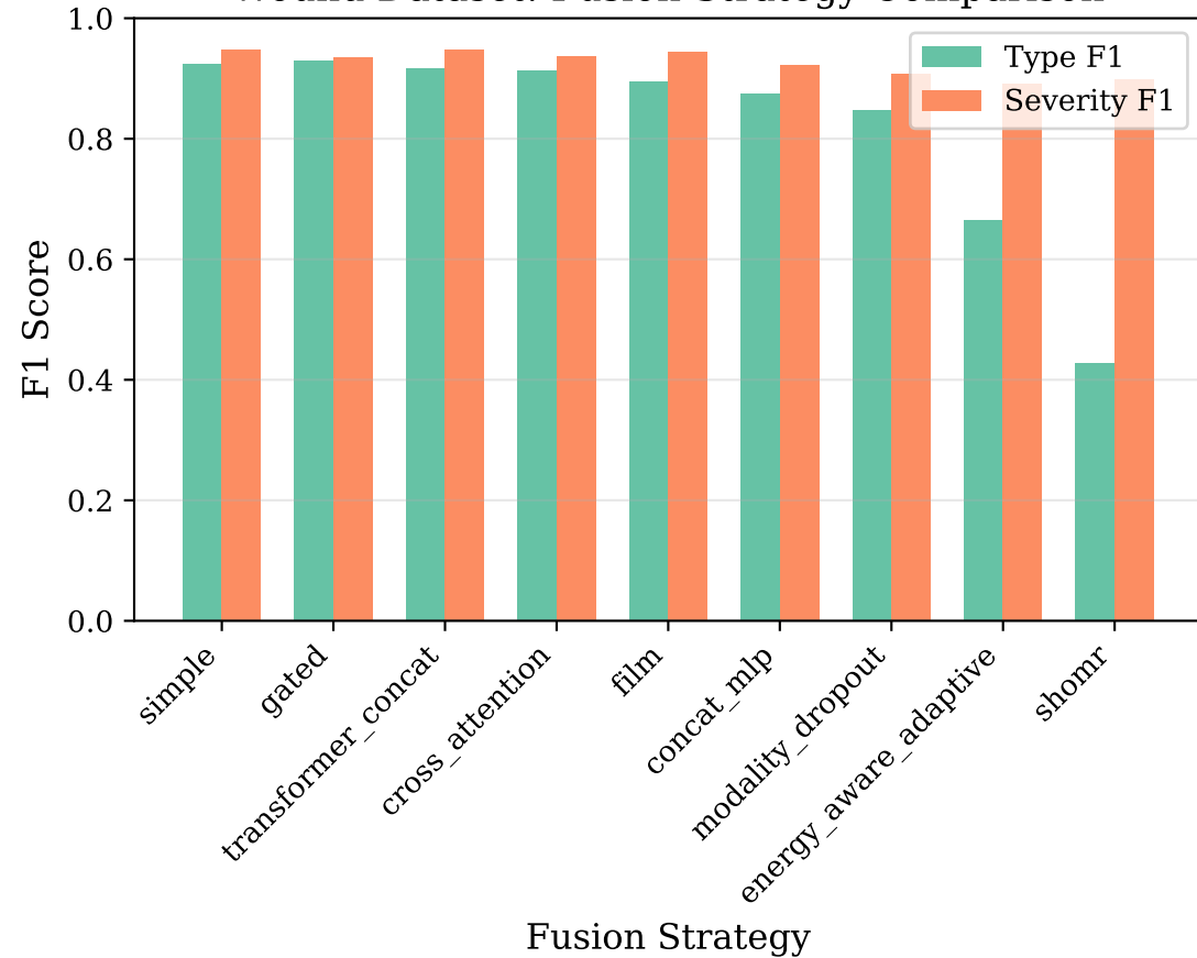
Wound Dataset: Fusion Strategy Comparison
