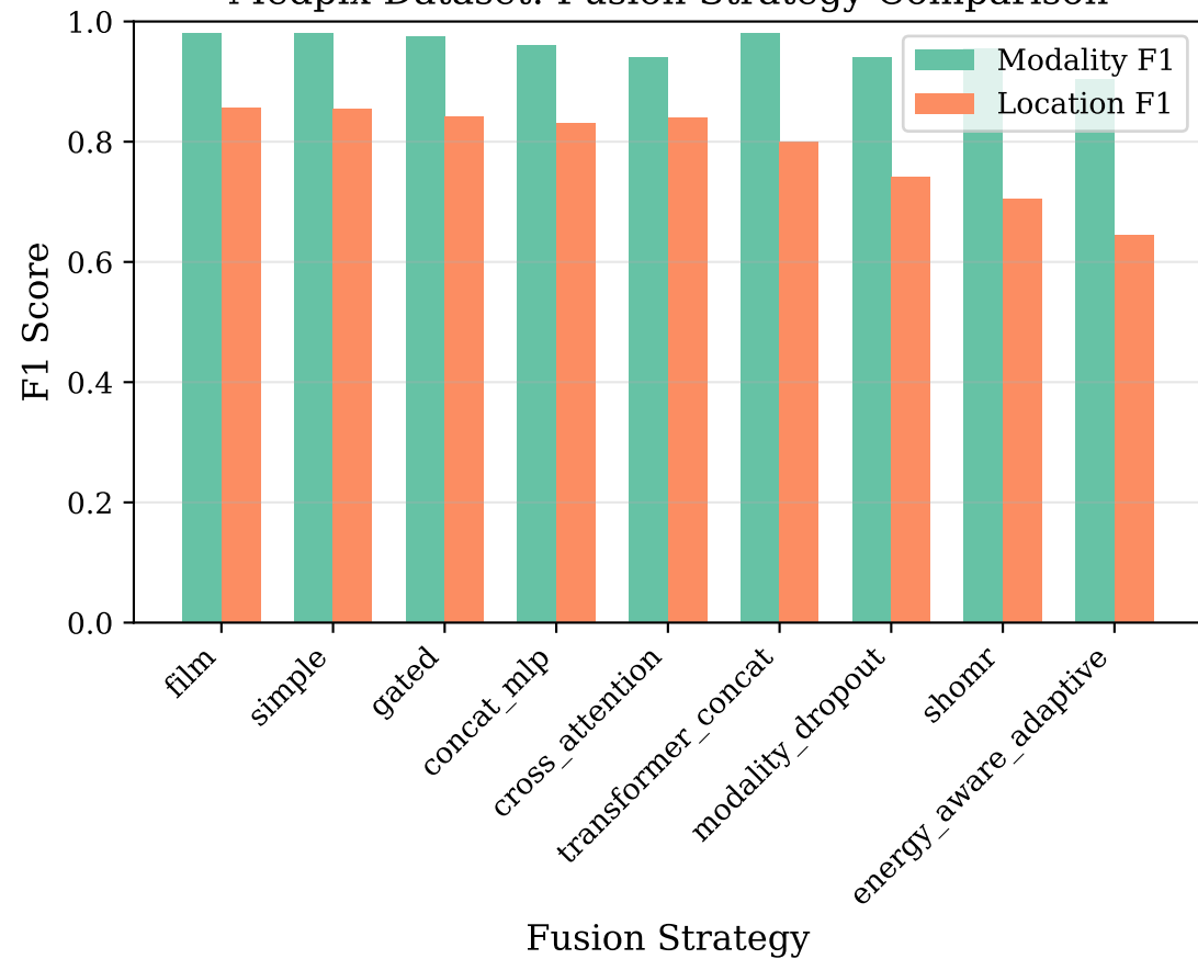
Medpix Dataset: Fusion Strategy Comparison
