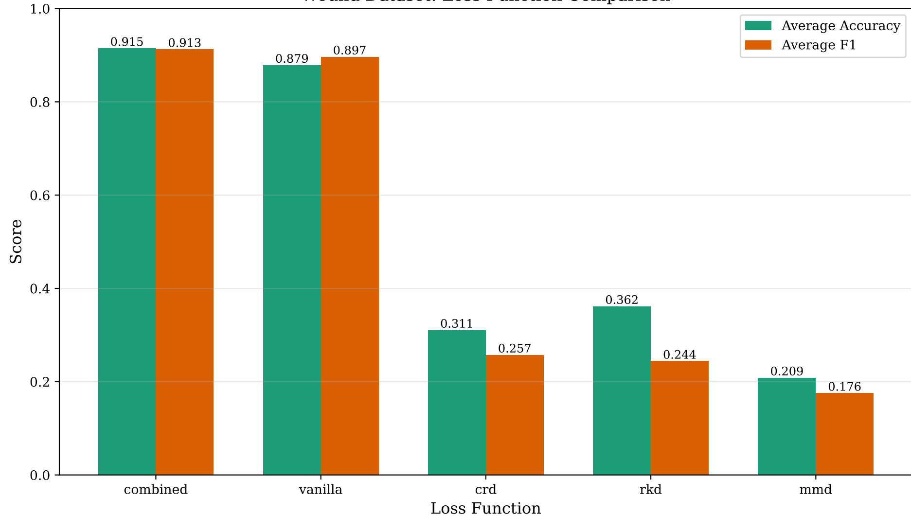
Wound Dataset: Loss Function Comparison
