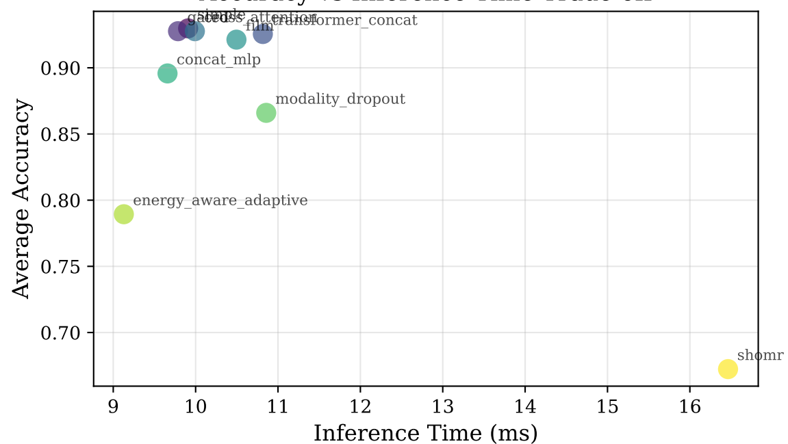
Accuracy vs Inference Time Trade-off
