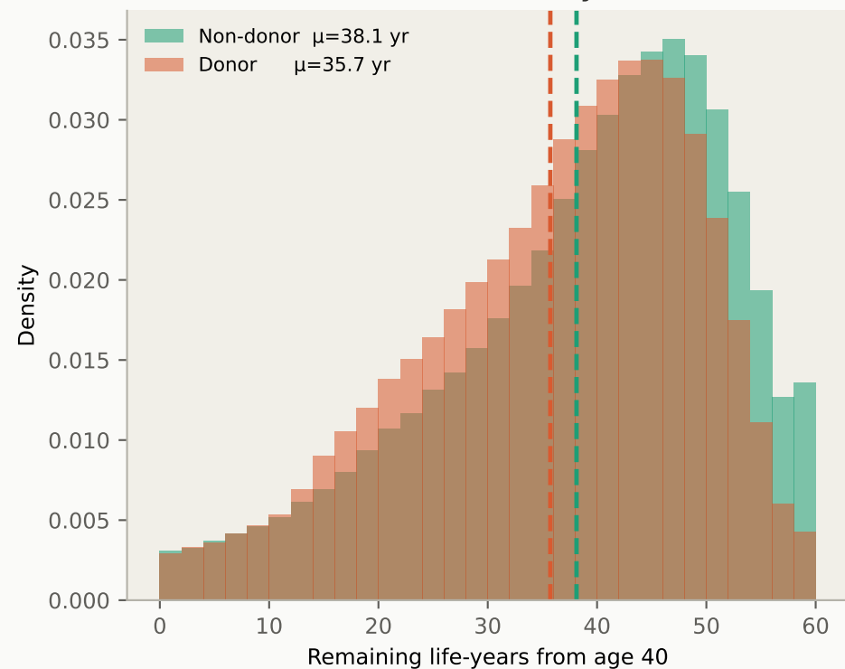
White donor \Delta LE = -877.0 days
