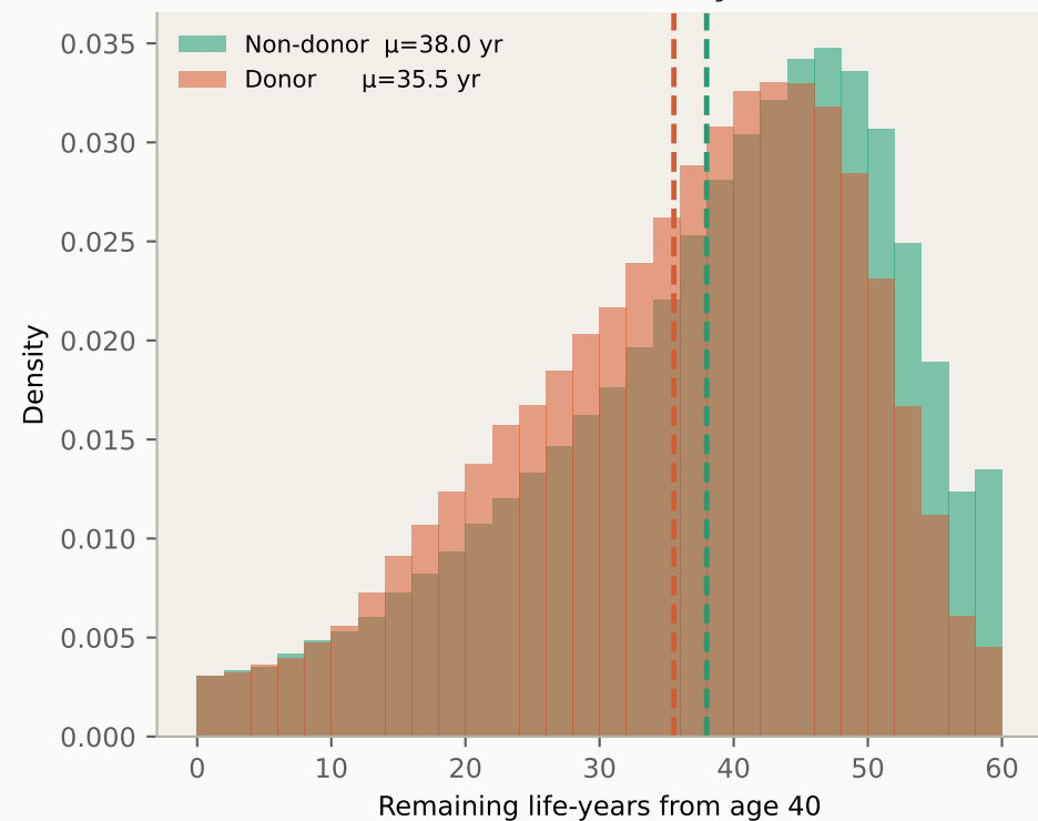
Black donor \Delta LE = -895.1 days
