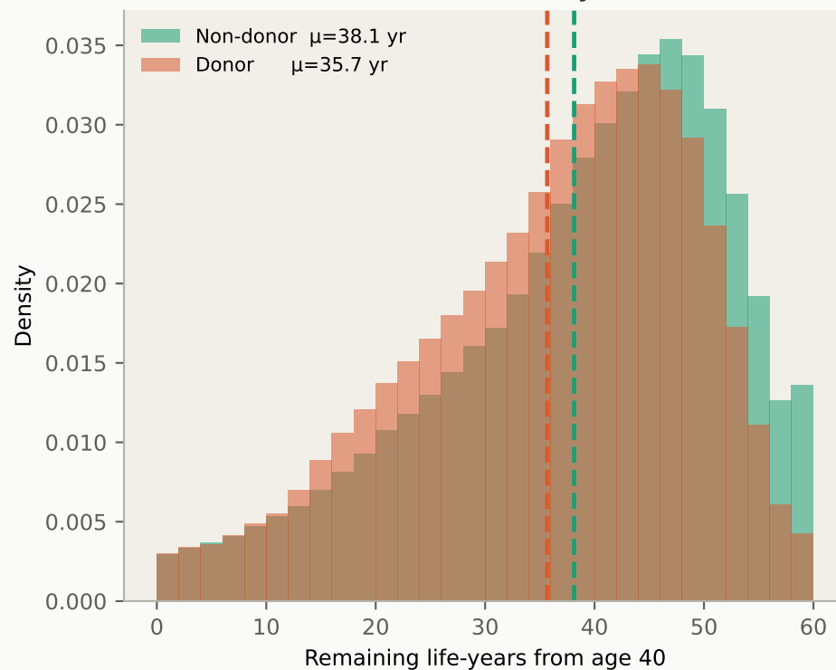
Overall (base) \Delta LE = -891.0 days
