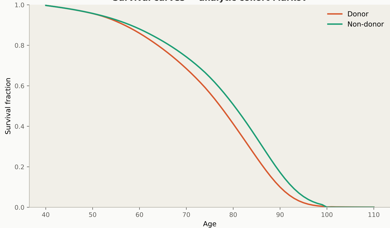
Survival curves — analytic cohort Markov
