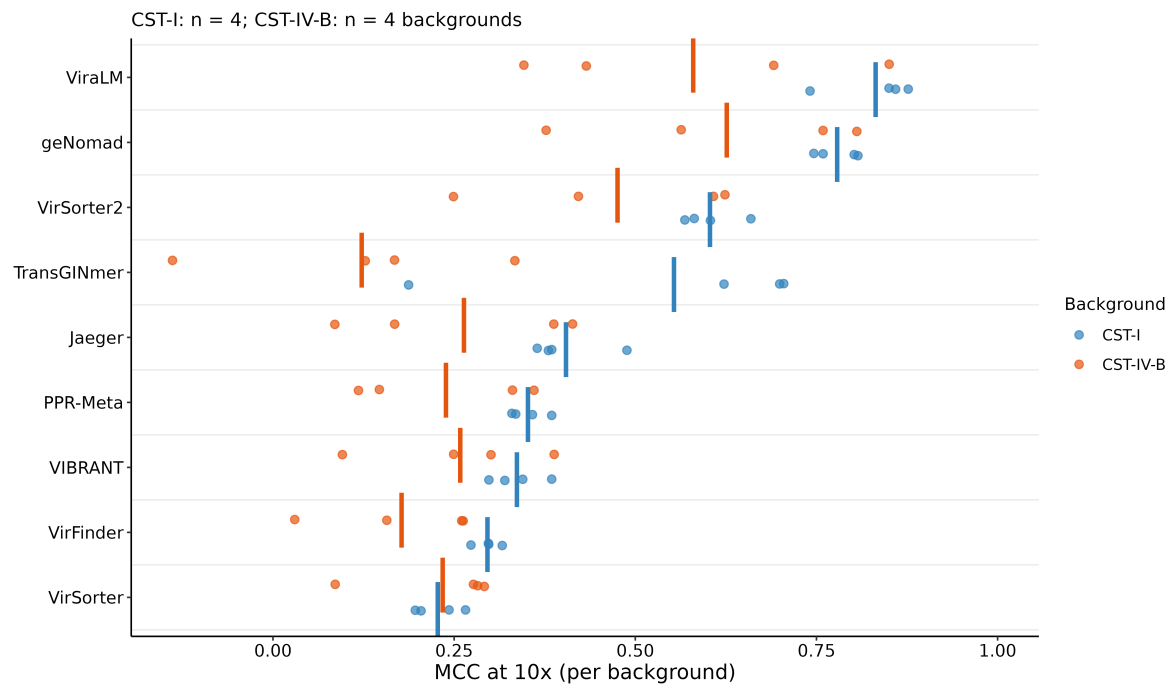
Figure S20. Per-background MCC underlying the CST-IV-B diversity contrast. MCC for the nine tools with the highest mean MCC in CST-I at 10× coverage across four CST-I and four CST-IV-B real backgrounds, with the CST groups distinguished by colour; each background is a point and the vertical bar is the arm mean. n = 4 backgrounds per arm.
