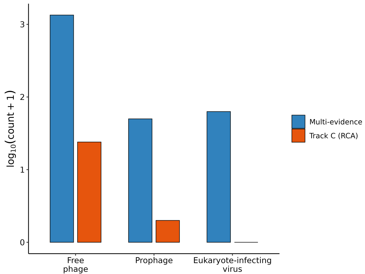
Figure S22. Viral-category composition of the multi-evidence and Track C positive sets. Viral-category composition of the multi-evidence Tier 1+2 viral-positive contigs and the Track C true-positive contigs ( n = 29 ), on a \log_{10}(\text{count} + 1) axis; free phage dominate both sets.
