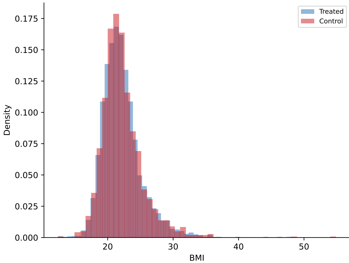
Figure 4: Outcome distributions by treatment group
