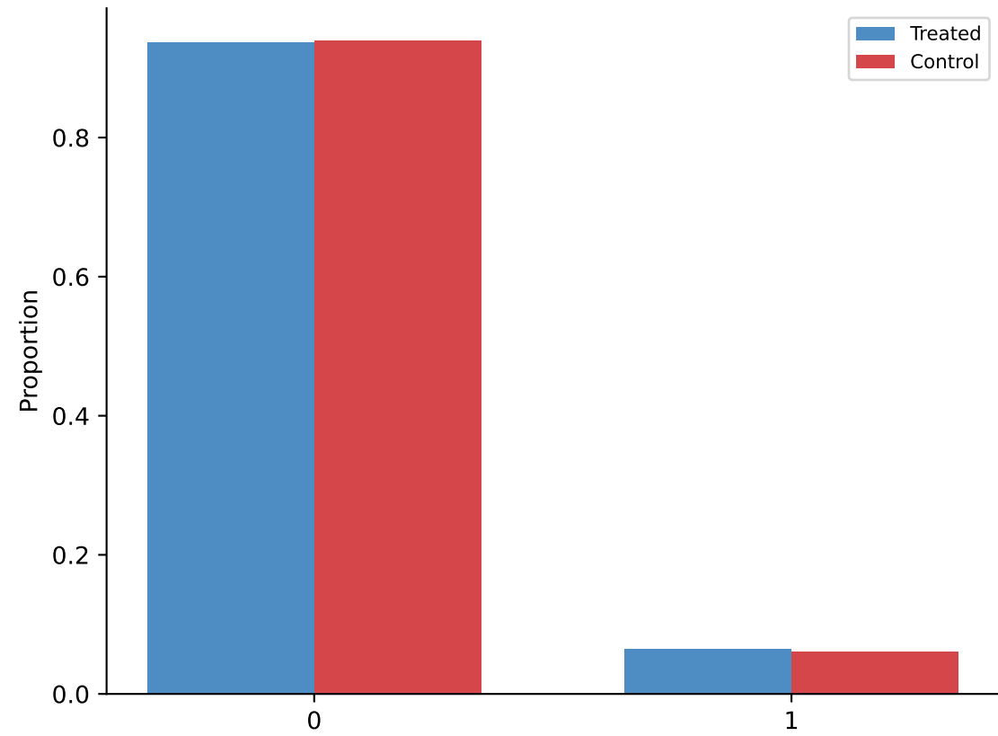
Figure 4: Outcome distributions by treatment group
