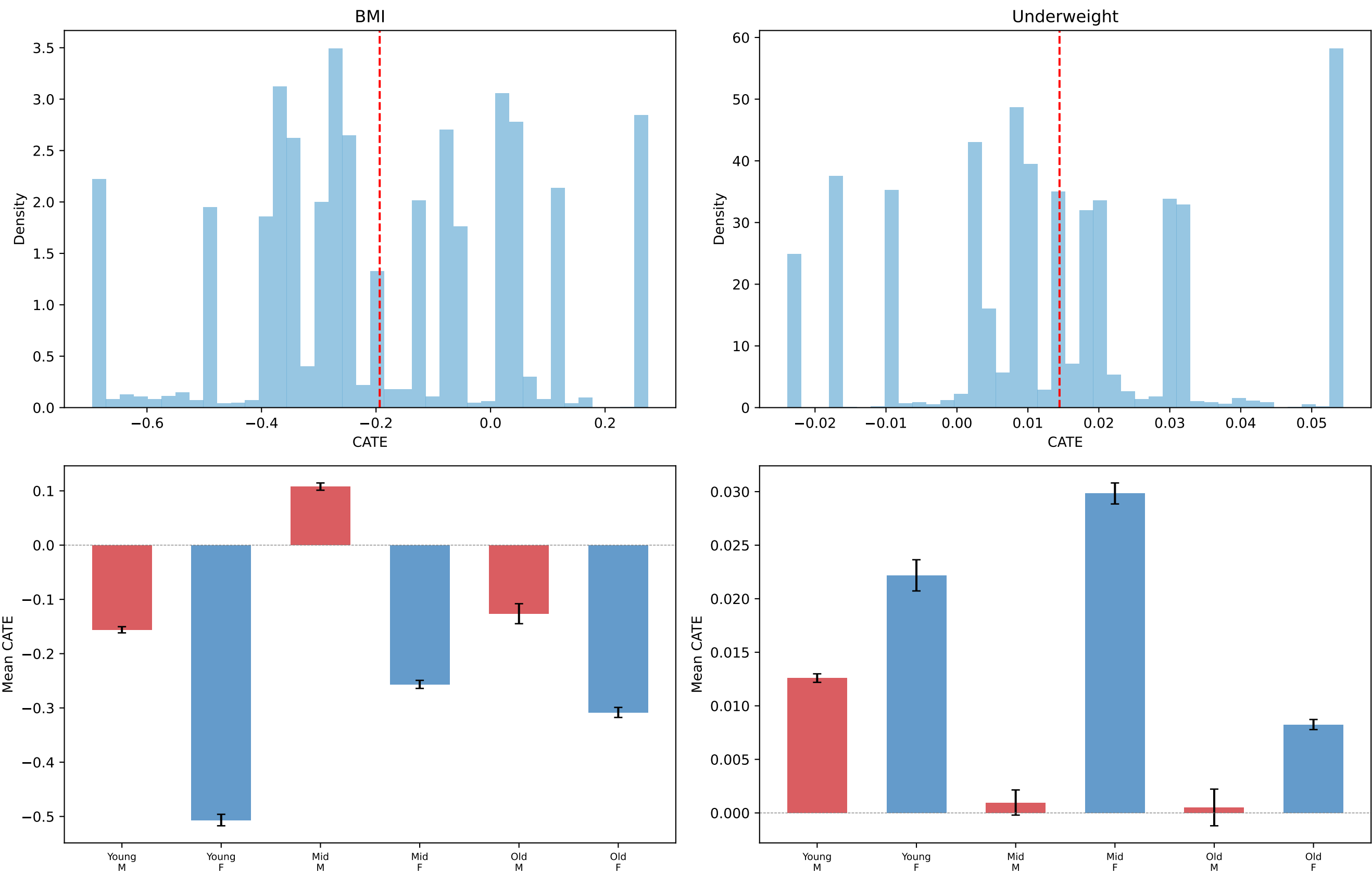
Figure 7a: CATE — BMI and underweight
