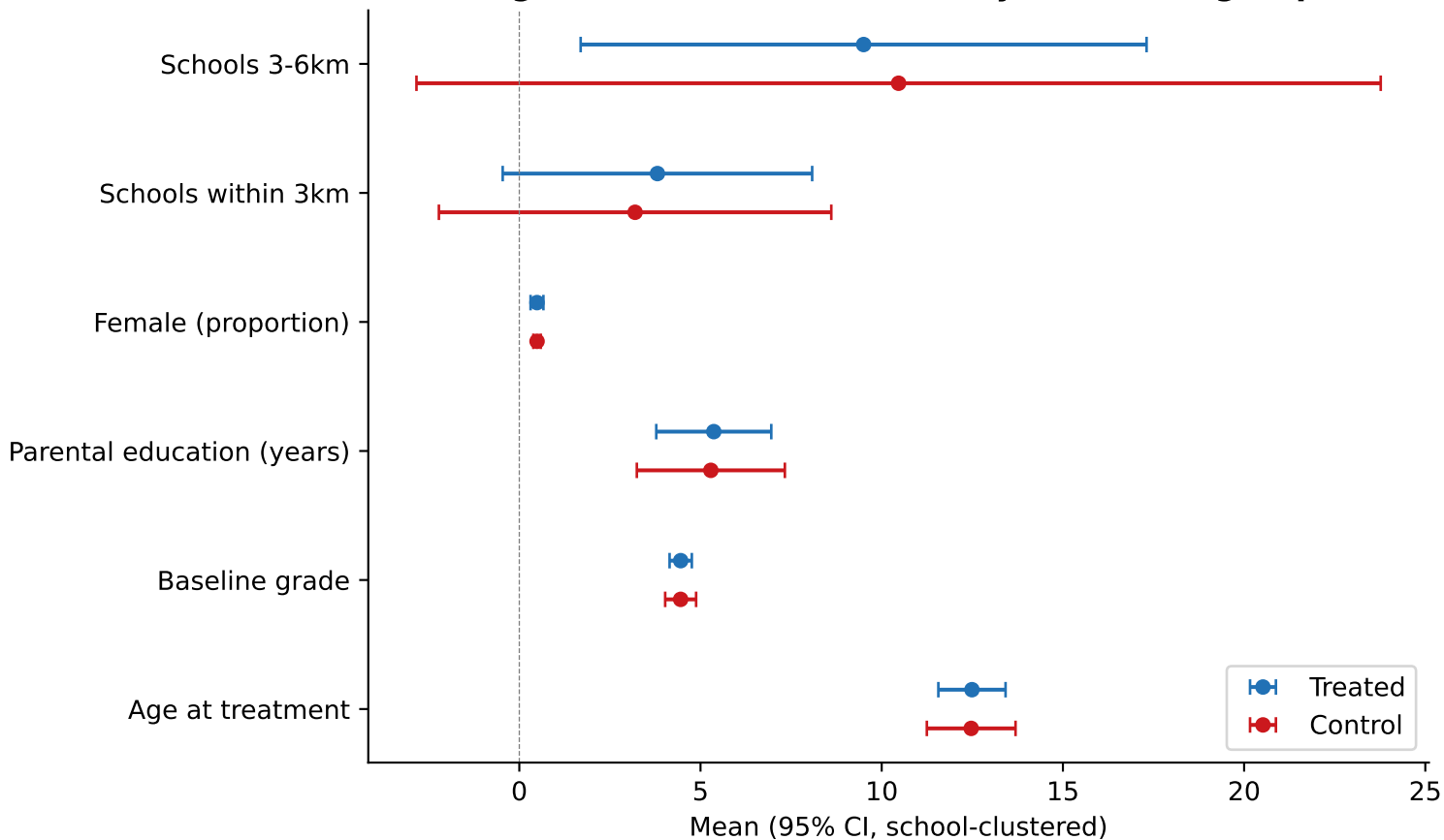
Figure 2: Covariate balance by treatment group
