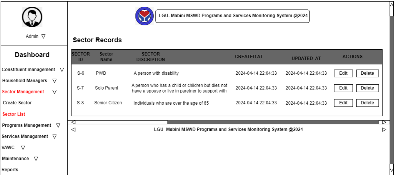
Figure 18.0 Sector List Prototype
