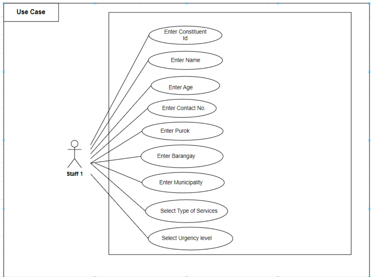
Figure 6.0 Service Request Form Use Case
