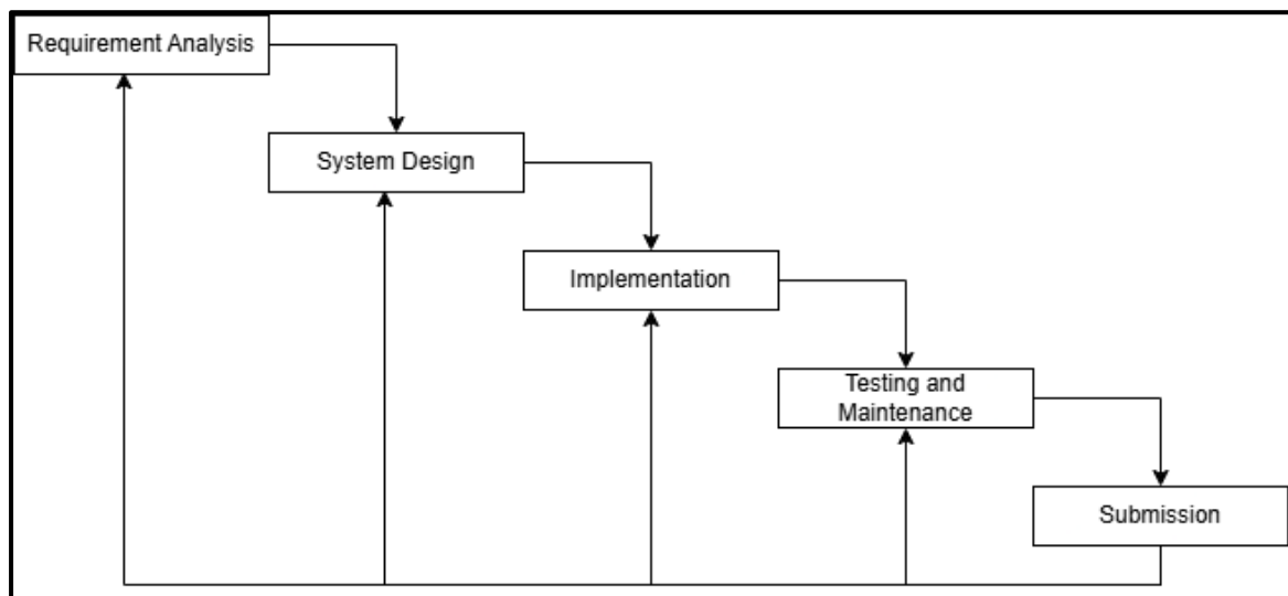
Figure 0.1: Waterfall Model
