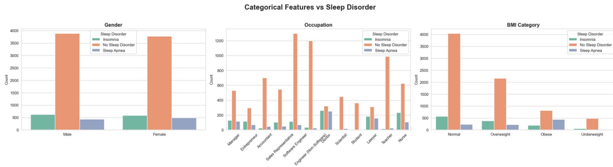
Figure 4.4b — Categorical Features vs. Sleep Disorder
