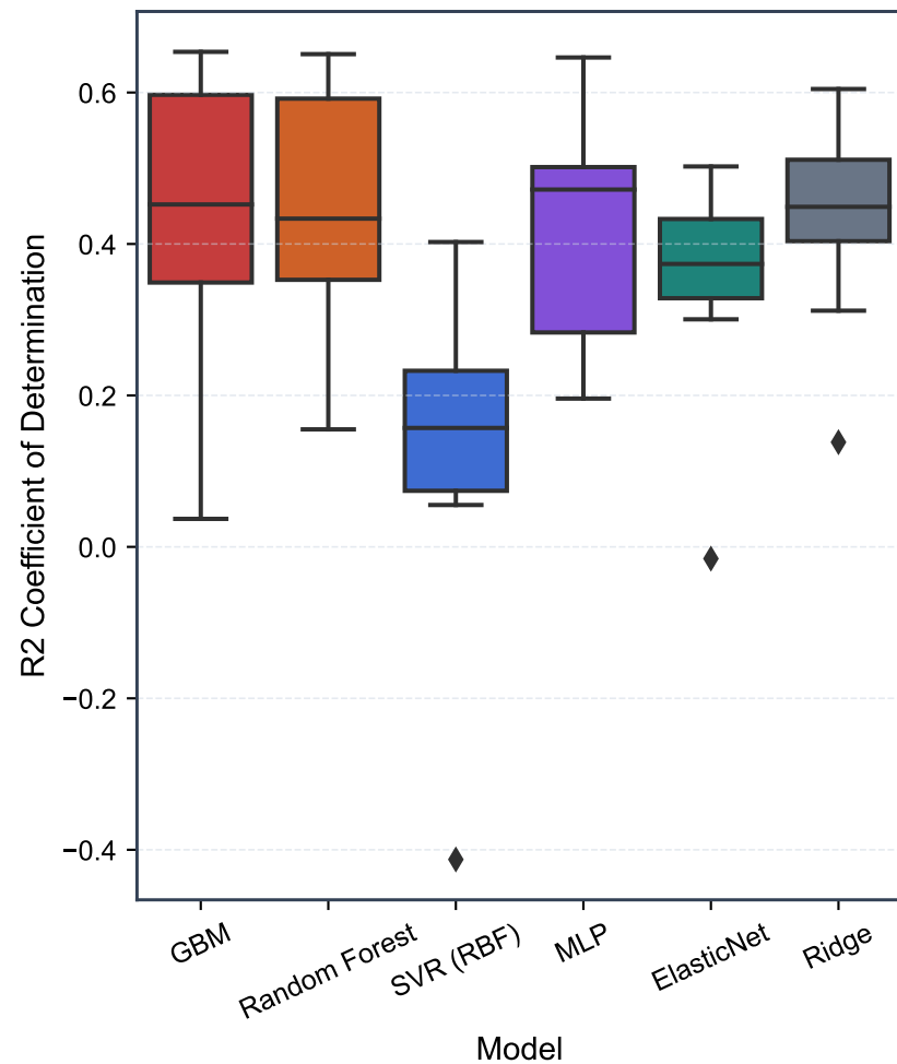
A. Cross-Validated R2 Score
