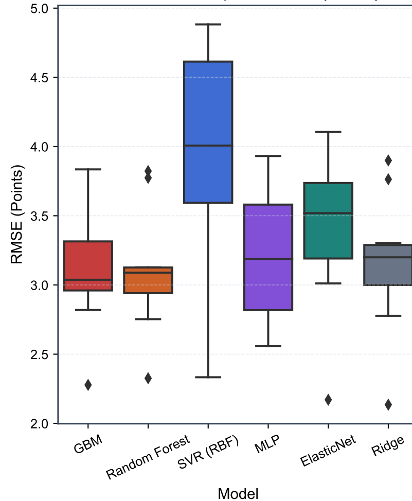
B. Root Mean Squared Error (RMSE)
