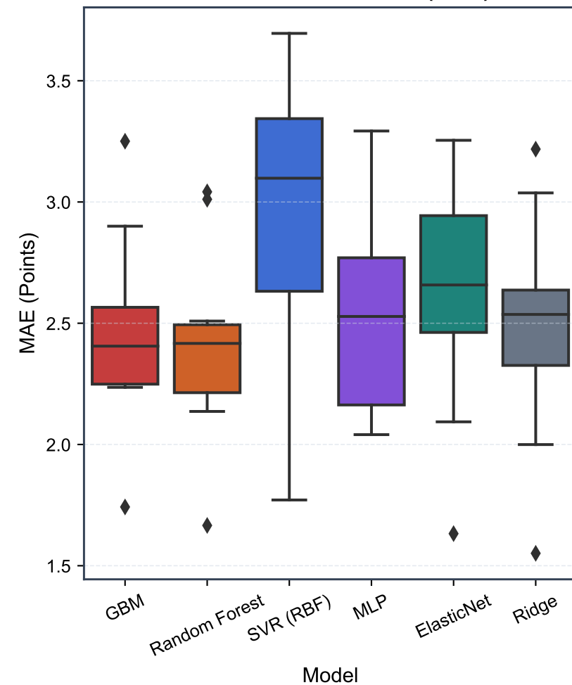
C. Mean Absolute Error (MAE)
