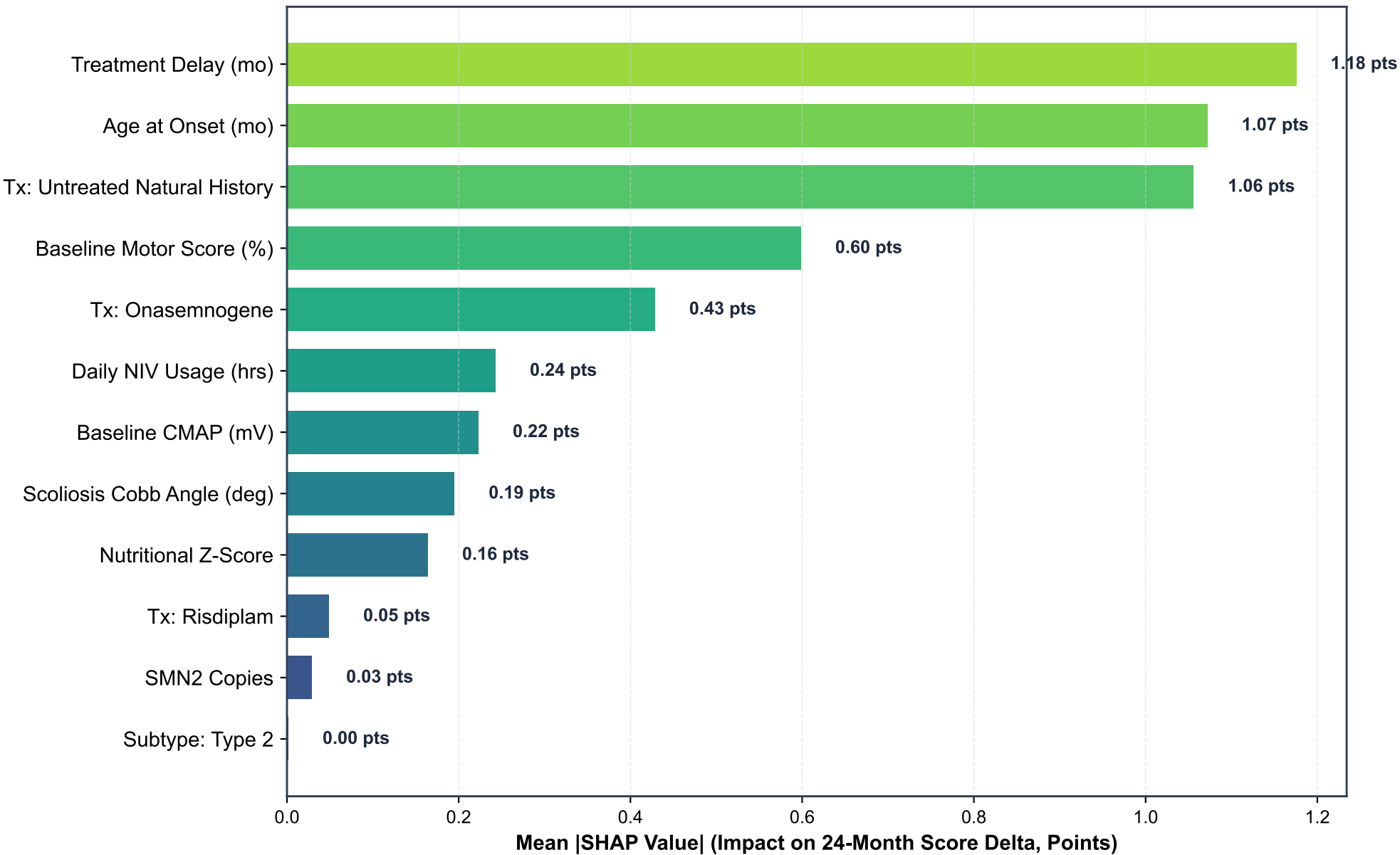
Global Feature Importance Ranking via SHAP TreeExplainer
