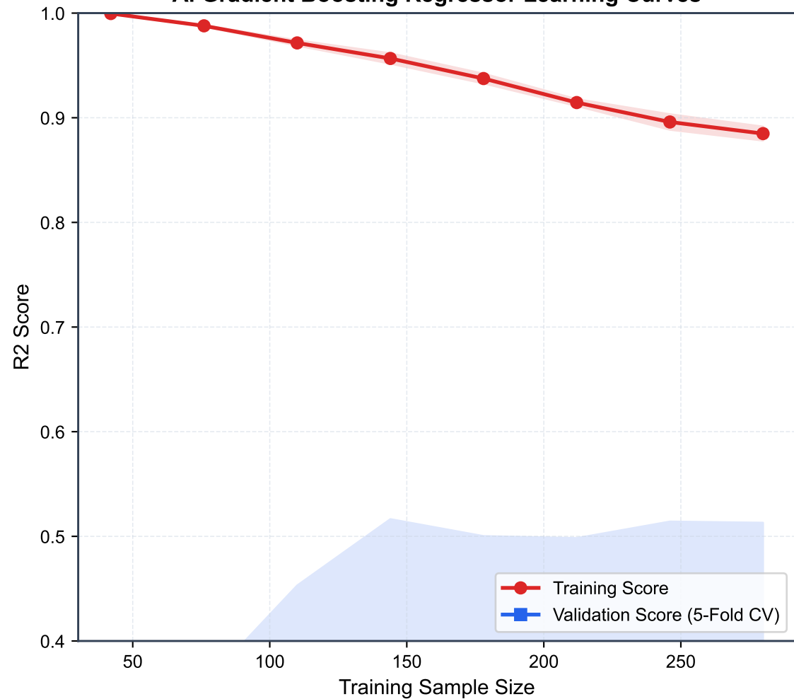
A. Gradient Boosting Regressor Learning Curves
