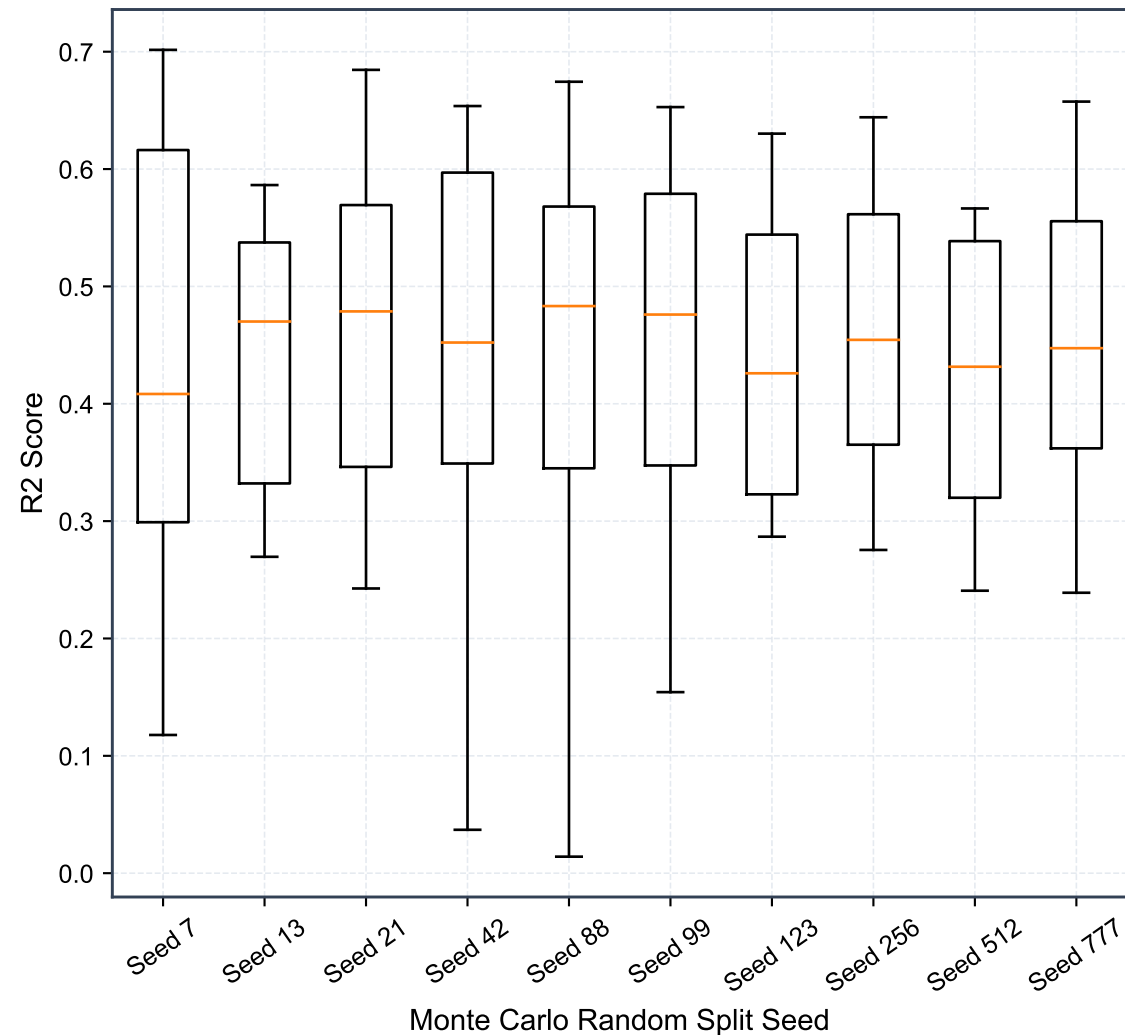
B. 10-Fold CV Score Distribution Across 10 Random Seeds
