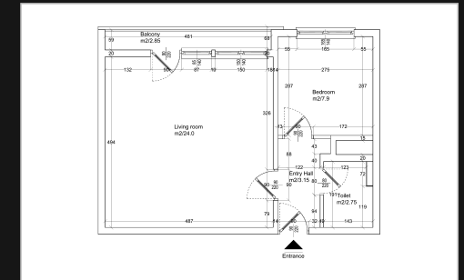
Dimensioned plan 1:20
