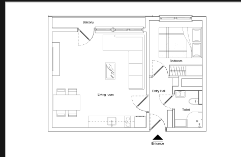
Floor plan 1:20
