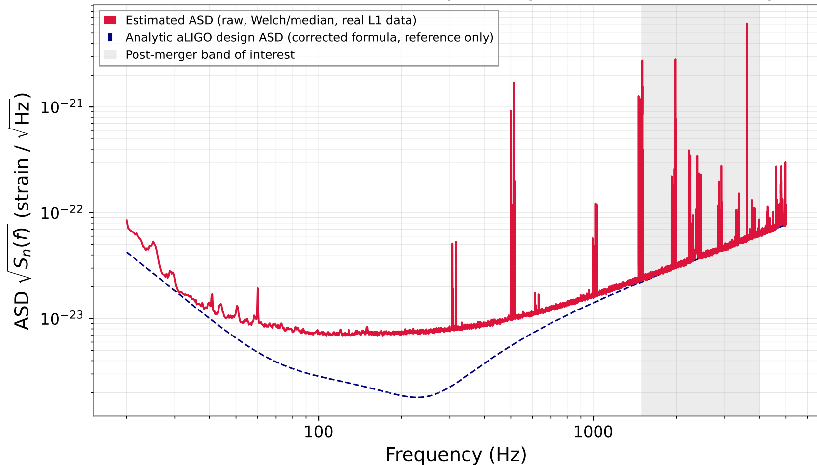
Estimated real-noise ASD vs. analytic design curve (cross-check only)
