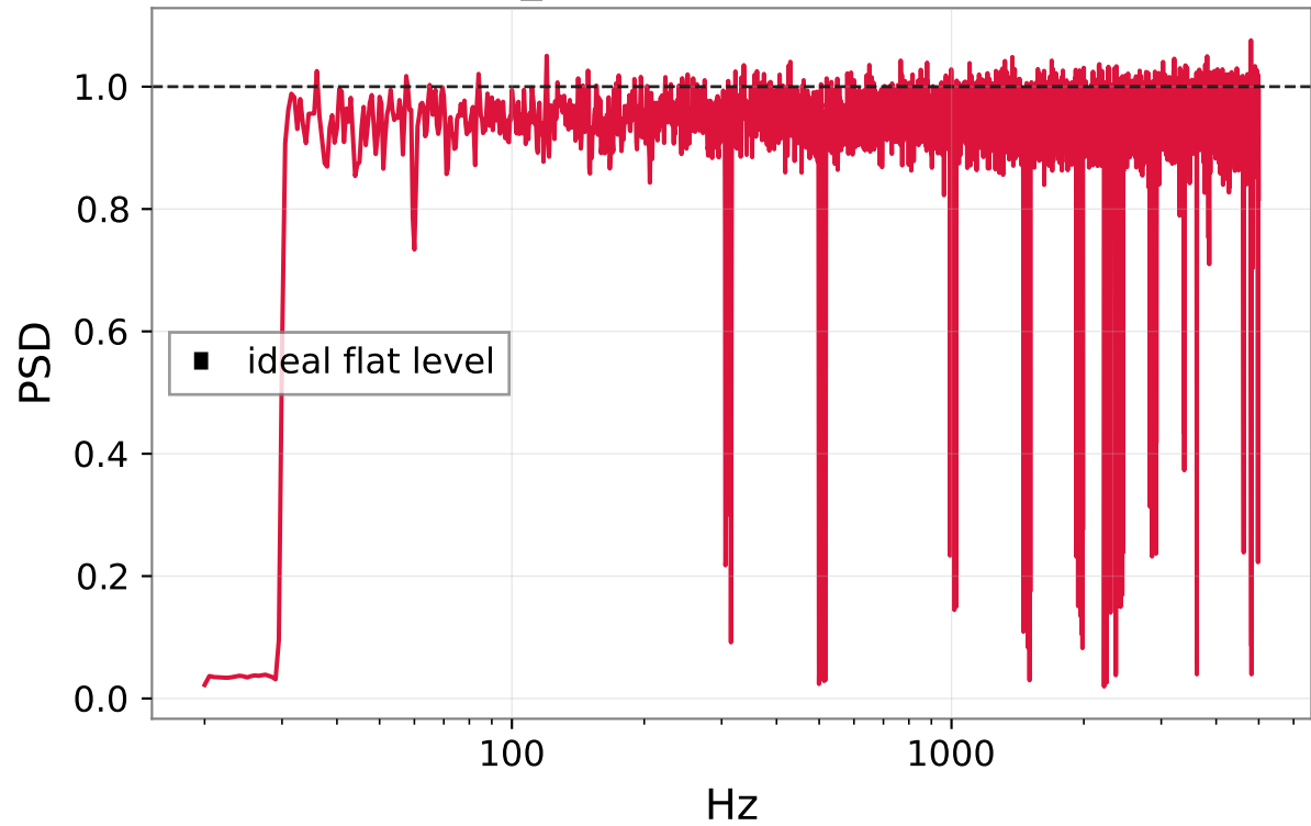
Whitened calib_block PSD (should be roughly flat)
