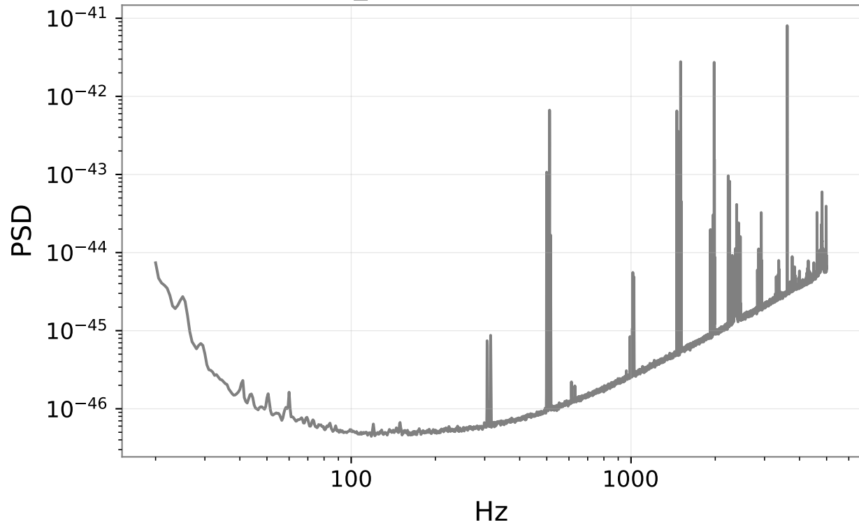
Raw calib_block PSD (before whitening)
