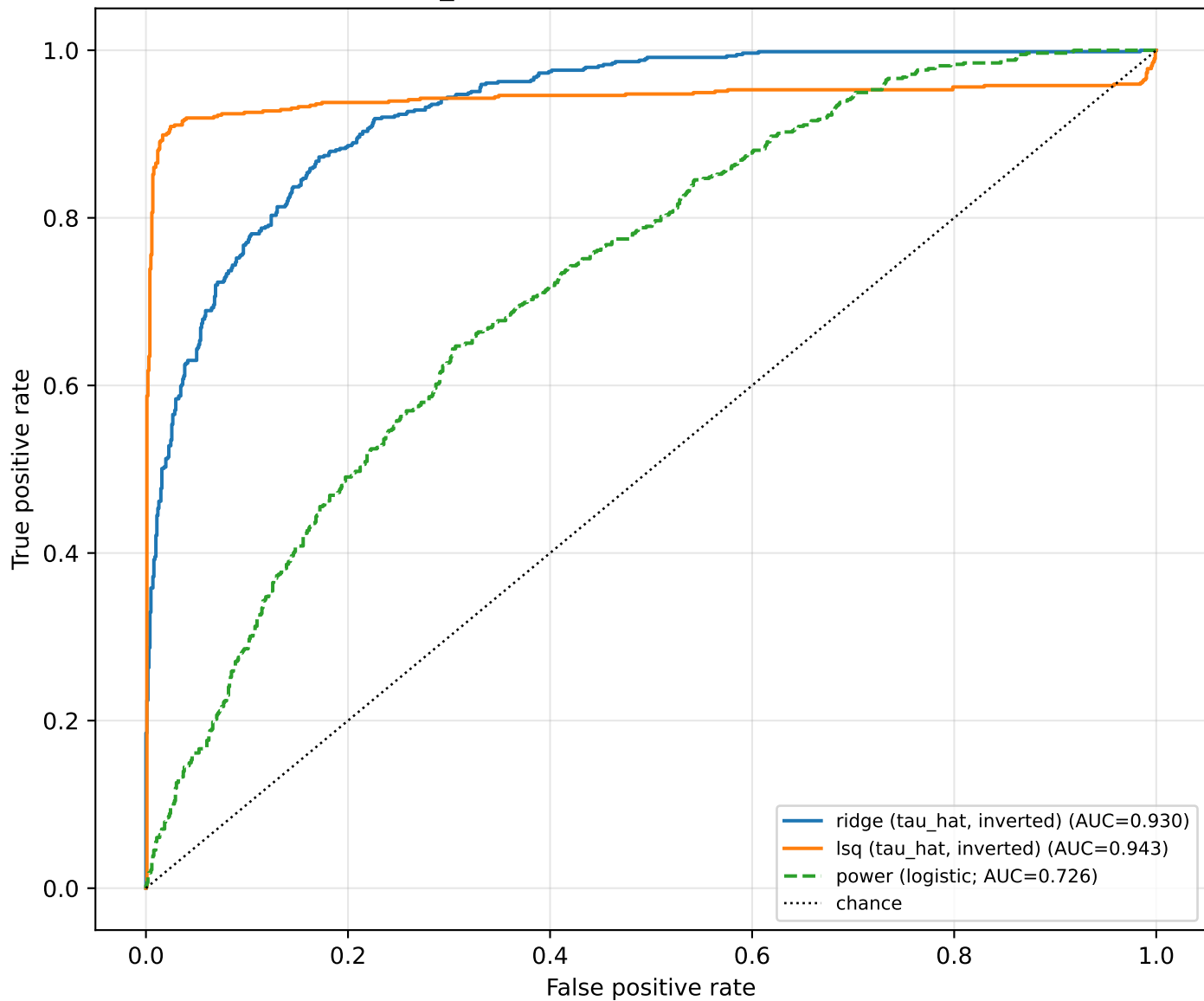
FINAL test_block discrimination (frozen thresholds)
