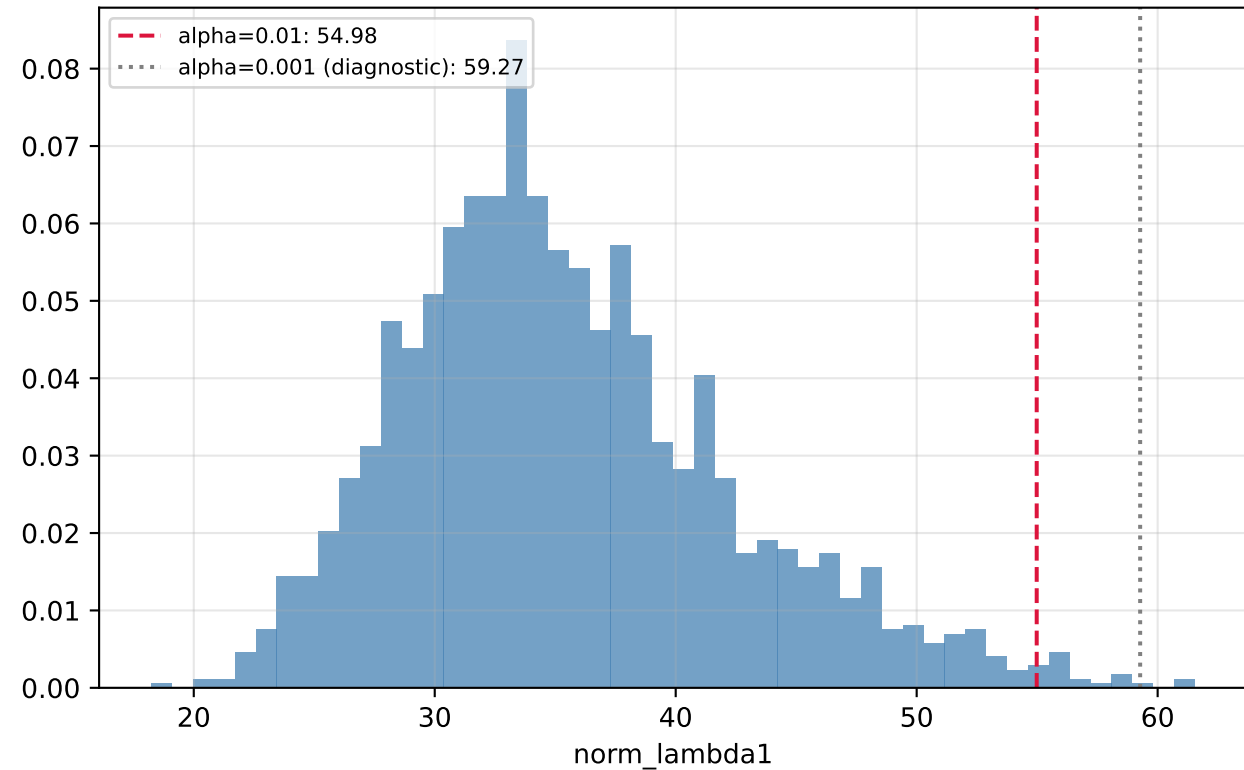
Null distribution: norm_lambda1
