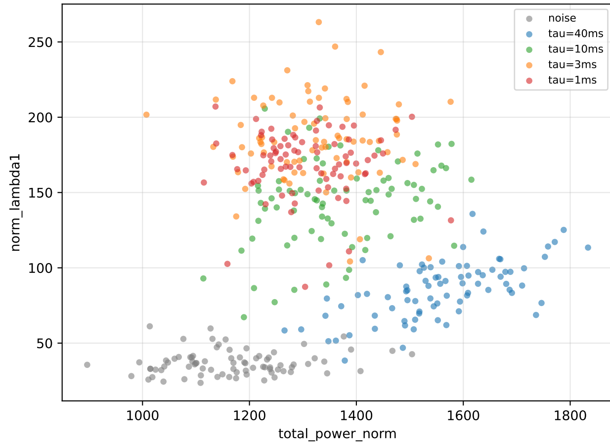
Normalized: power vs. lambda_1
