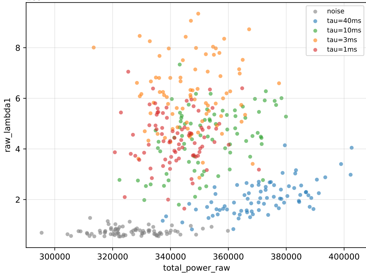
Raw: power vs. lambda_1
