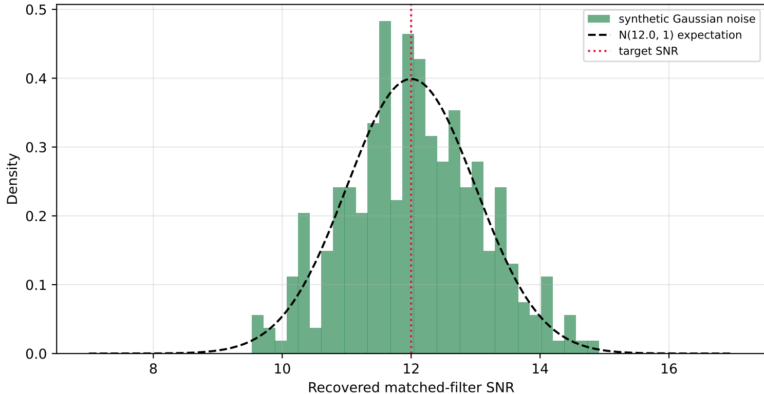
Test A: recovery on synthetic PSD-matched Gaussian noise
