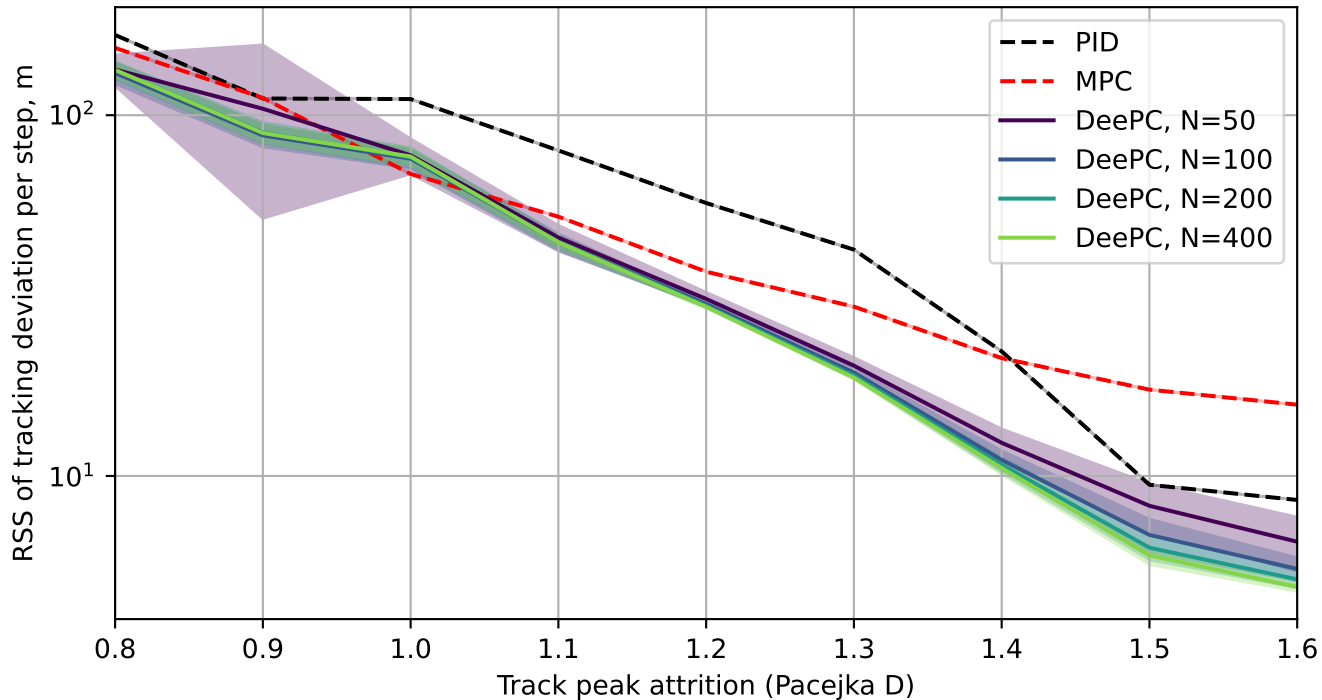
Tires friction variation on Abu Dhabi circuit
