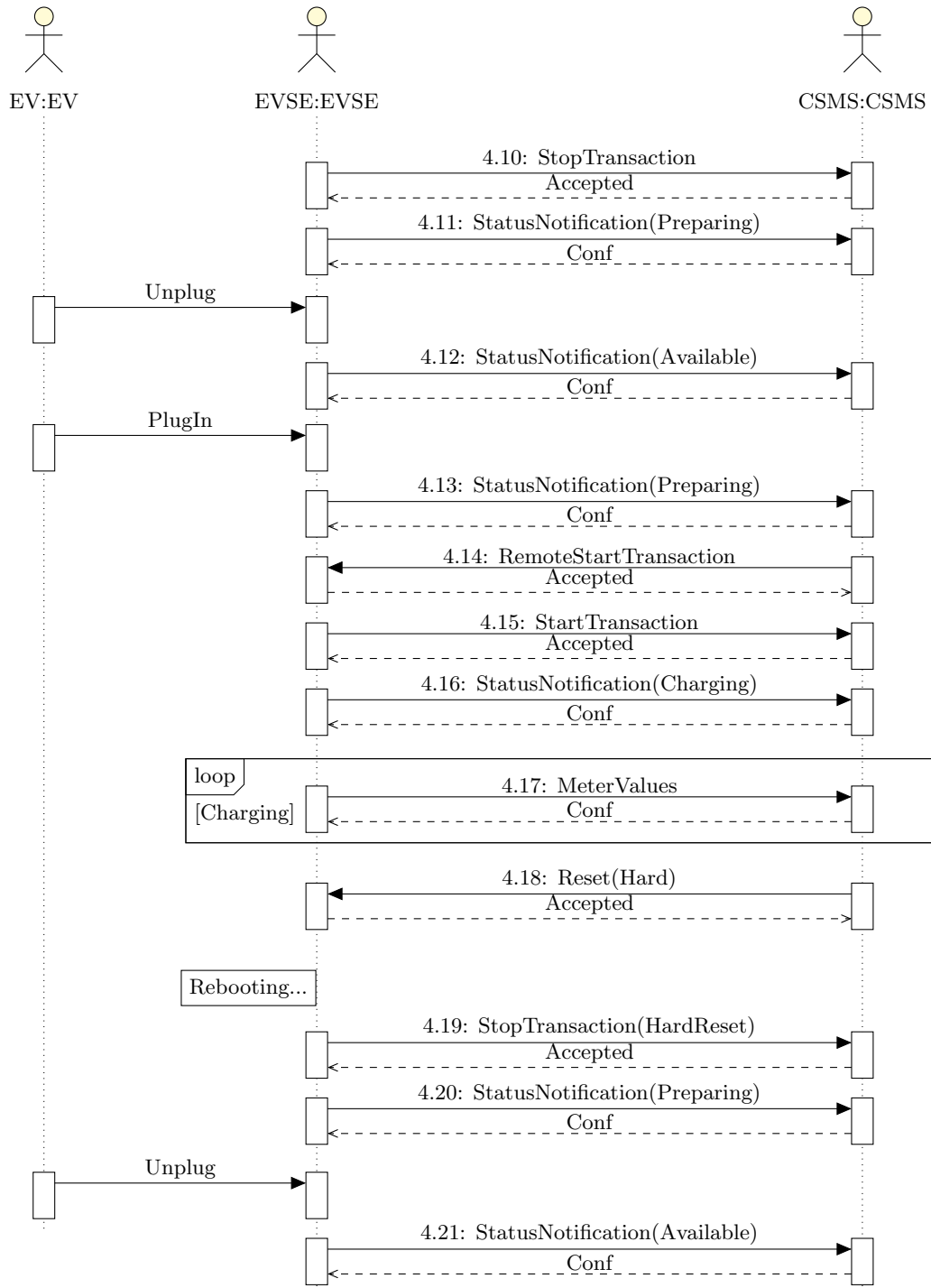
Figure 6.8: Reset Verification (Part 2)
