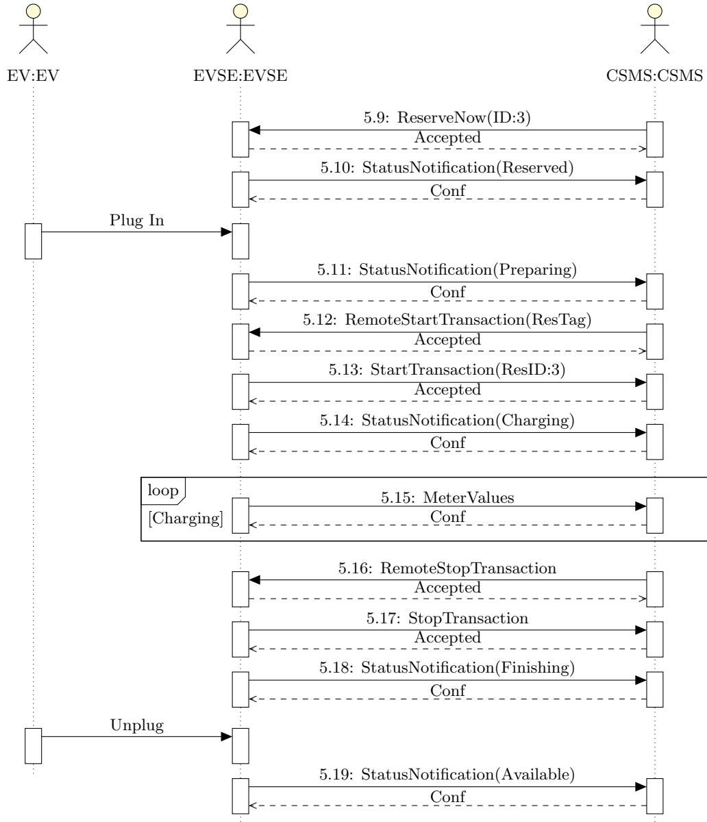
Figure 6.10: Reservation Verification (Part 2)
