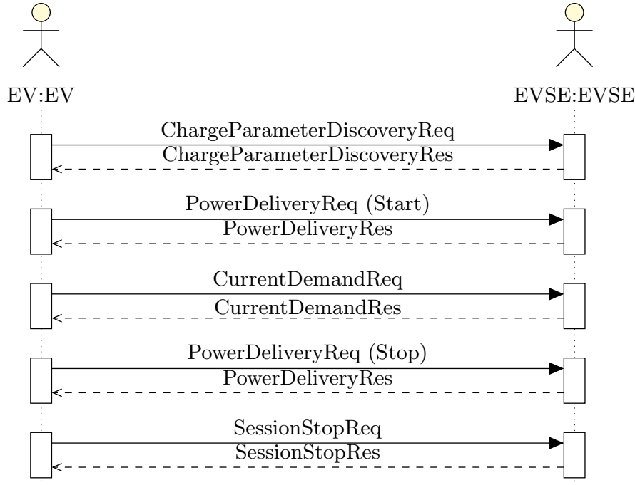
Figure 2.8: ISO 15118 Charging Loop Sequence
