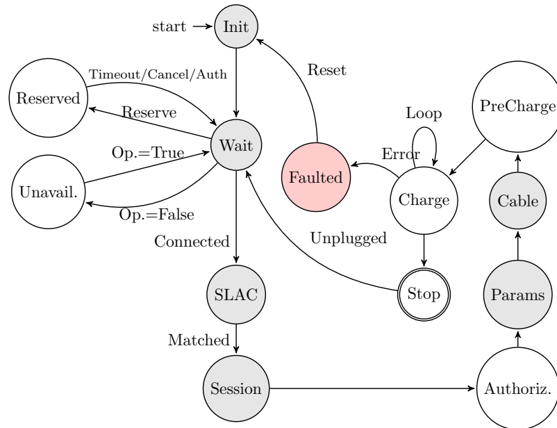
Figure 2.5: Low-Level EVSE State Machine (ISO 15118)
