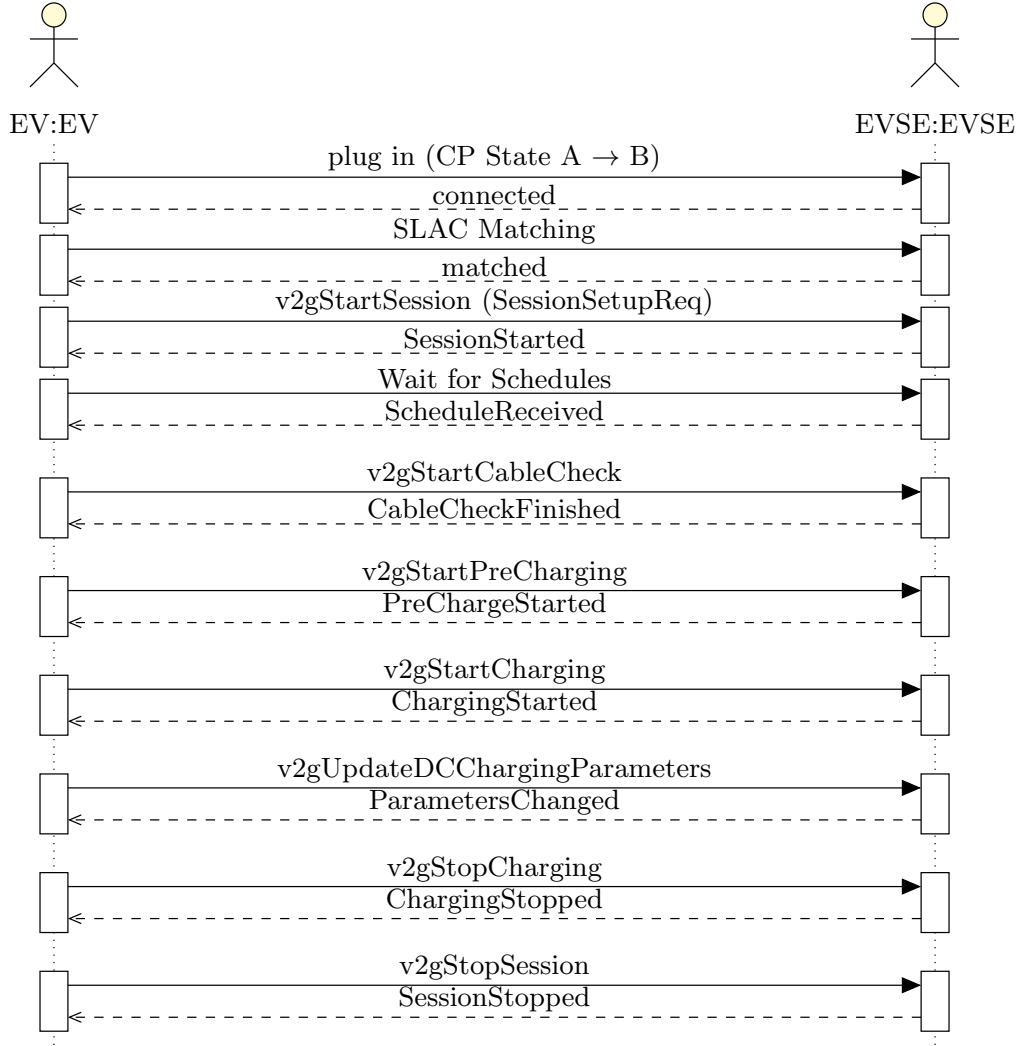
Figure 2.9: Detailed EV-EVSE Implementation Sequence
