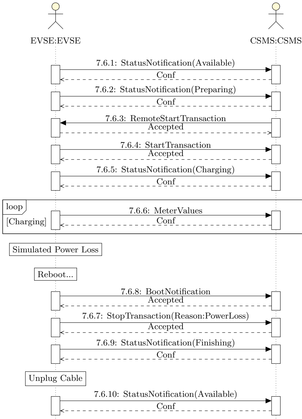
Figure 6.18: Power Loss Recovery Sequence
