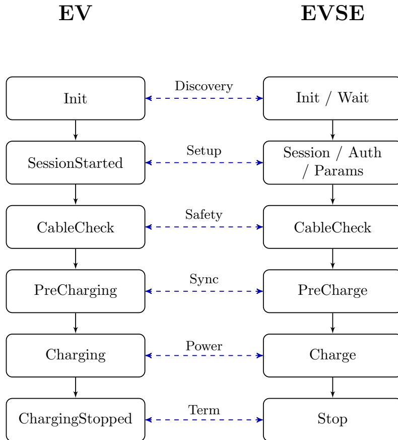
Figure 2.7: EV-EVSE State Synchronization
