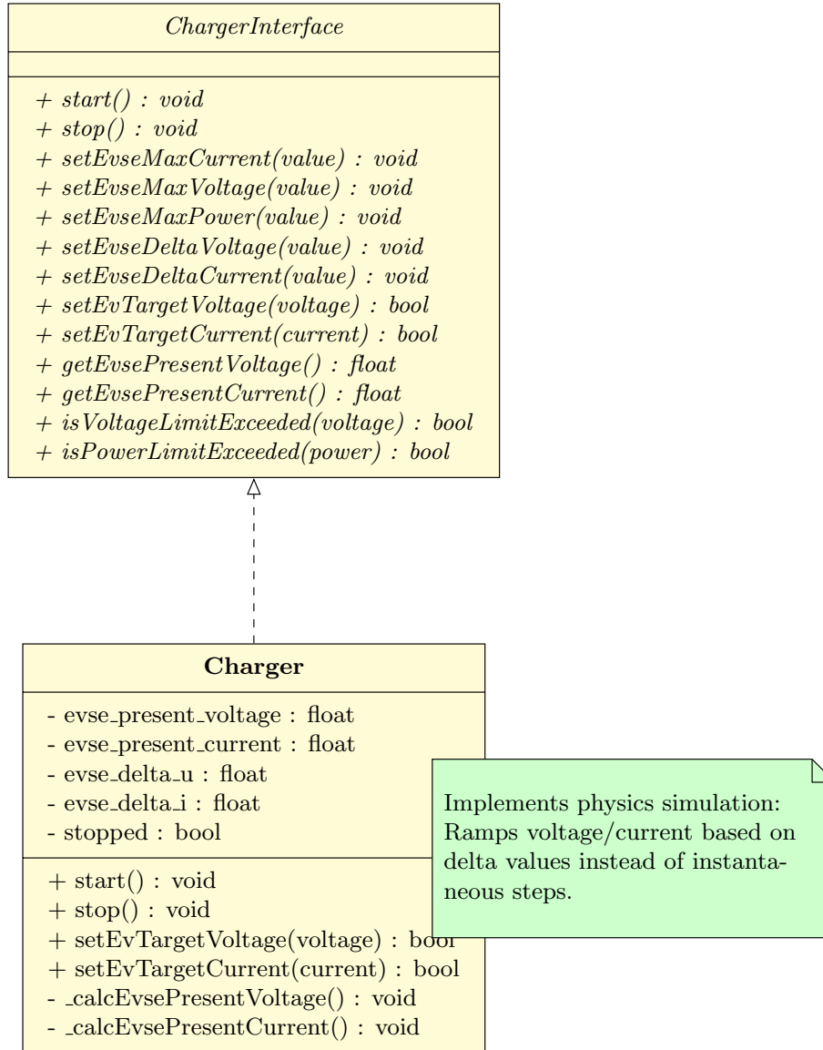
Figure 2.12: Charger Interface and Implementation
