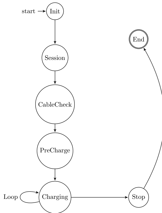
Figure 2.6: EV State Machine
