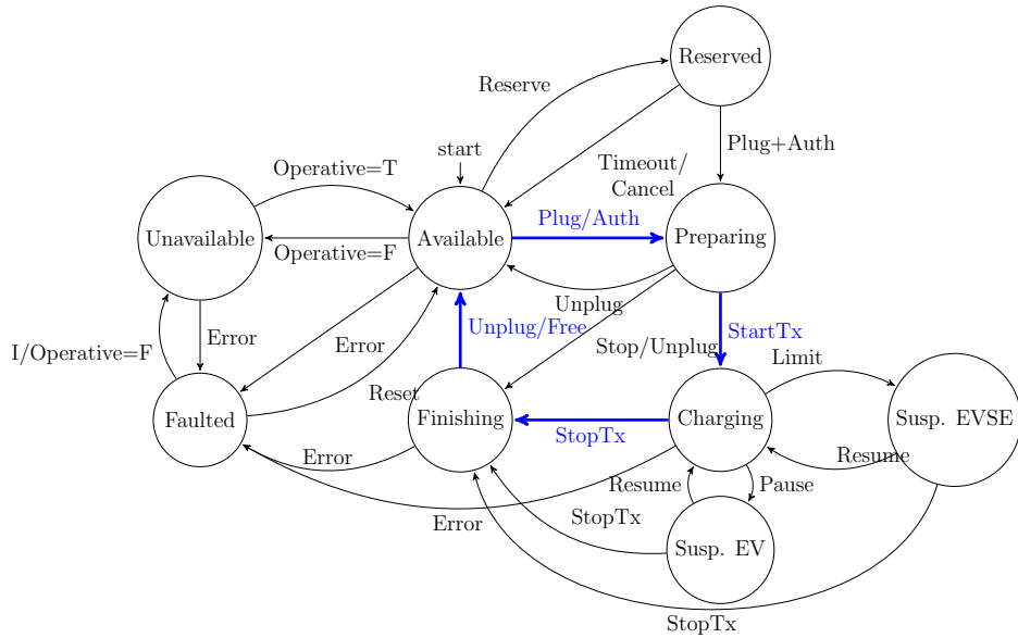
Figure 2.4: High-Level EVSE State Machine (OCPP)
