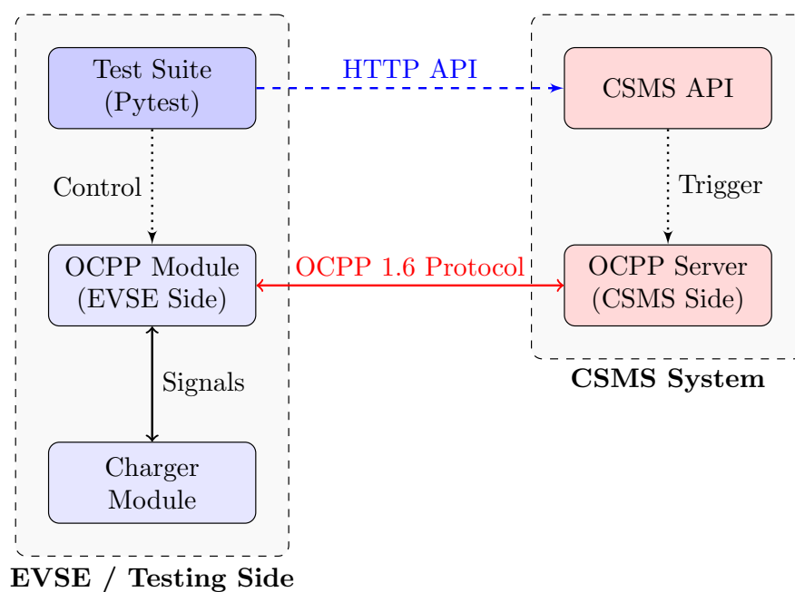
Figure 1: MEA OCPP 1.6 Compliance Testing Setup
