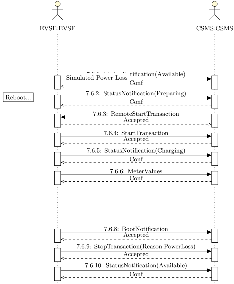
Figure 6.18: Power Loss Recovery Sequence
