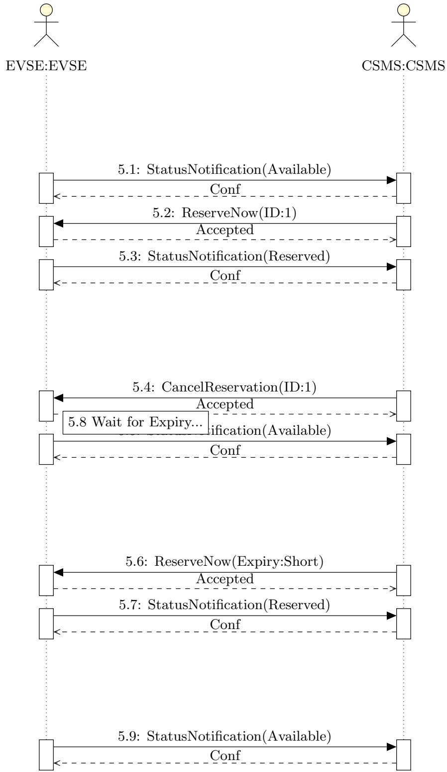
Figure 6.9: Reservation Verification (Part 1)
