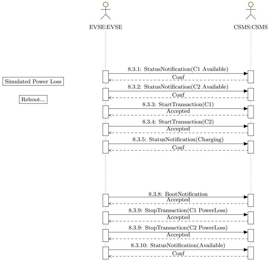
Figure 6.22: Dual Power Loss Sequence
