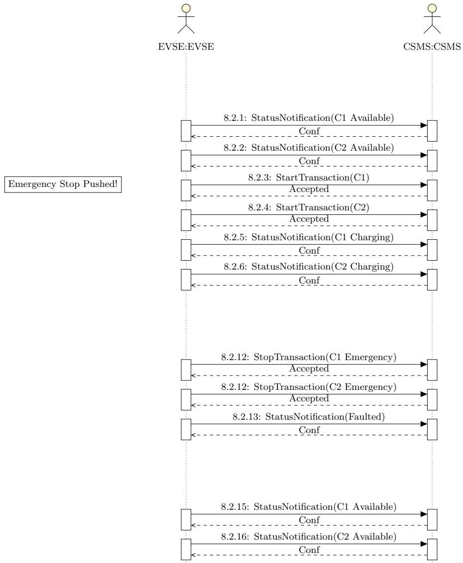
Figure 6.21: Dual Emergency Stop Sequence
