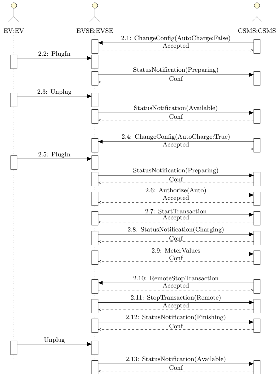
Figure 6.3: Auto Charge Verification (Part 1)
