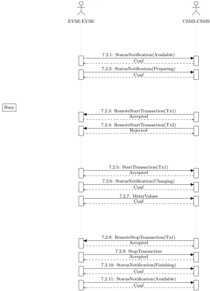
Figure 6.14: Concurrent Remote Start Sequence
