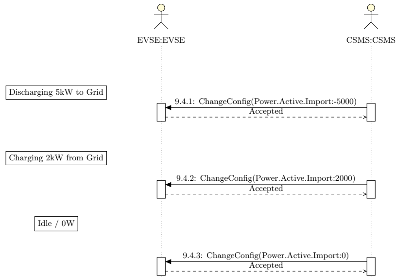
Figure 6.24: Power Demand Verification Sequence
