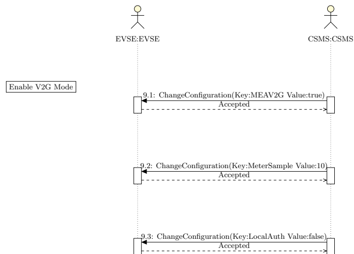
Figure 6.23: MEA General Configuration Sequence
