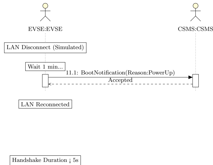
Figure 6.27: LAN Disconnect/Reconnect Sequence
