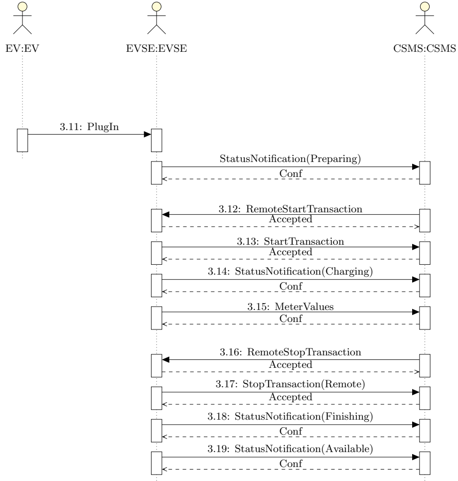
Figure 6.6: Normal Operation Verification (Part 2)
