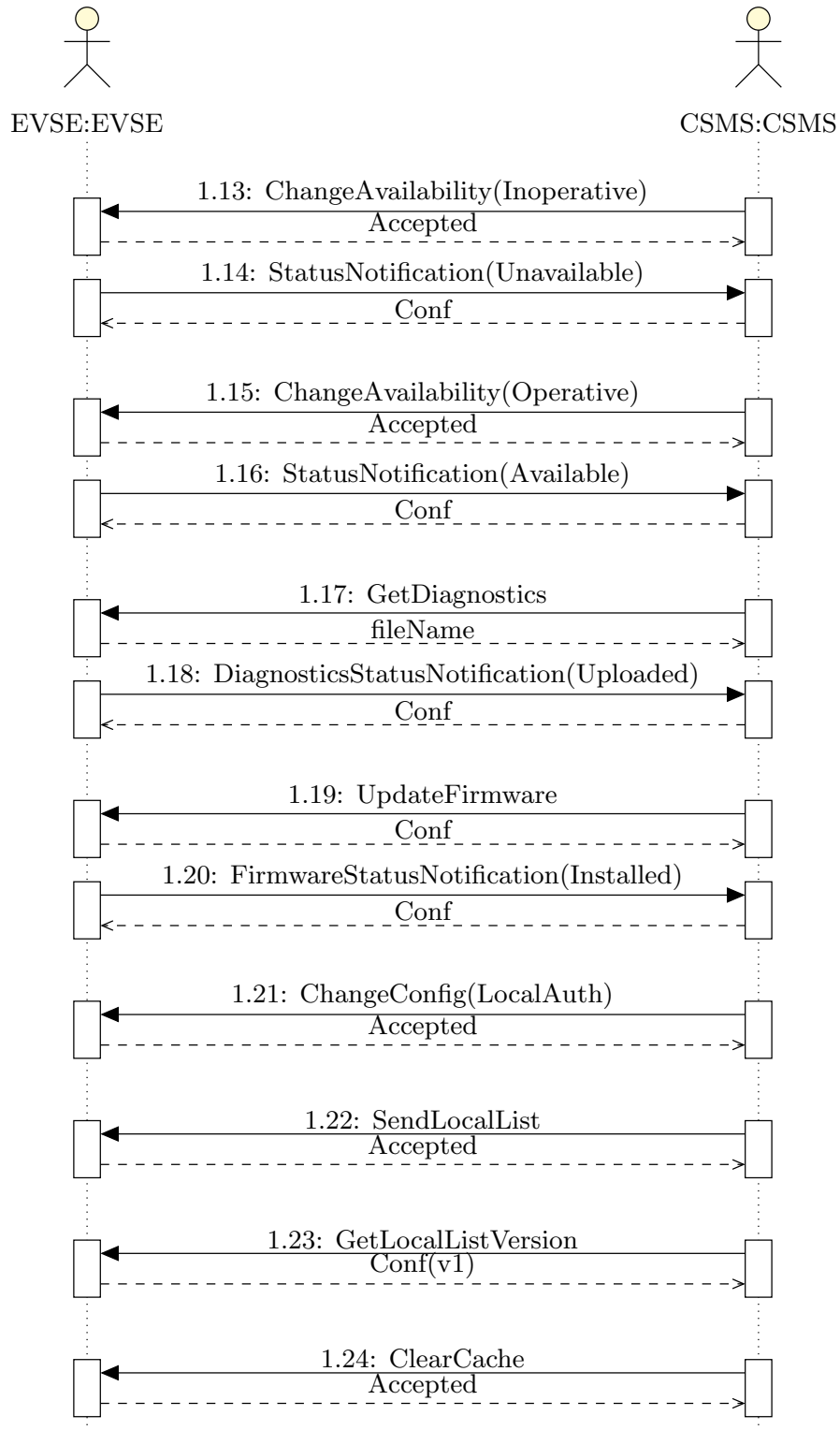
Figure 6.2: Configuration Verification (Part 2)
