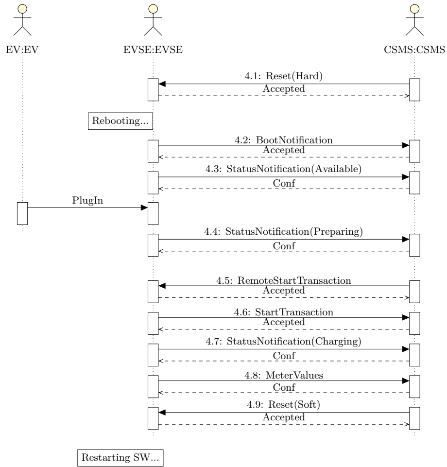
Figure 6.7: Reset Verification (Part 1)
