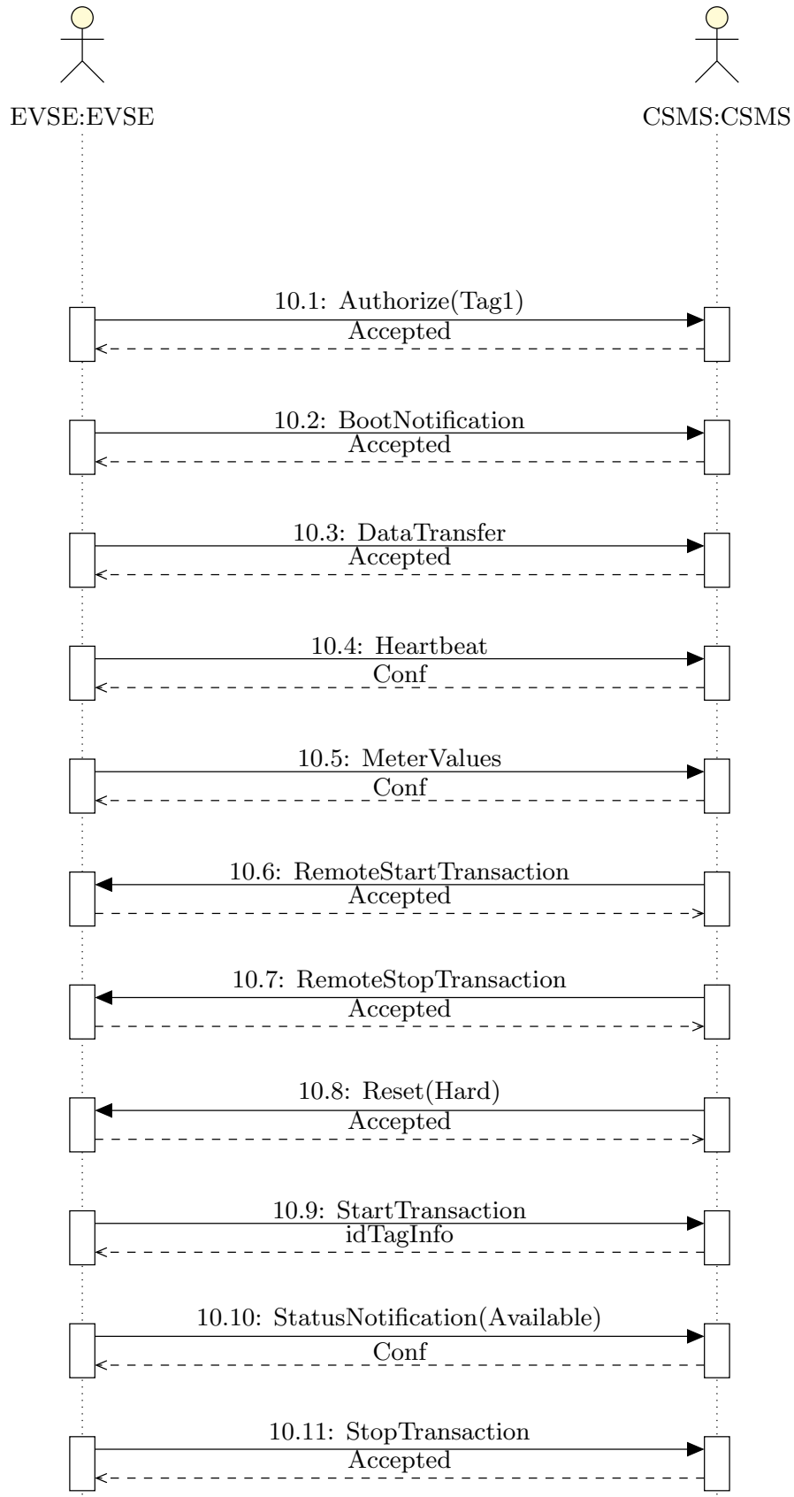
Figure 6.25: Summary Verification (Part 1)
