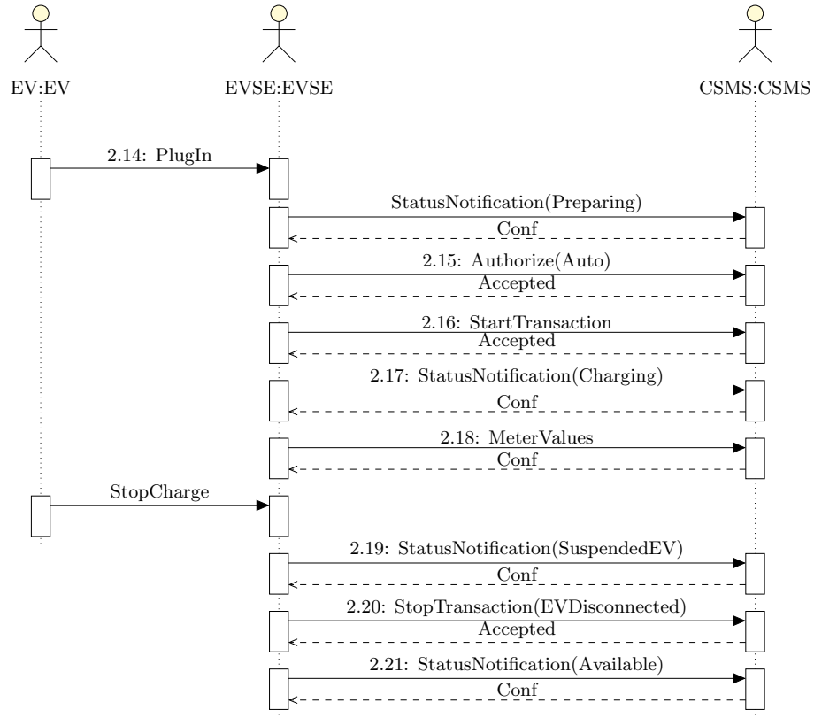
Figure 6.4: Auto Charge Verification (Part 2)
