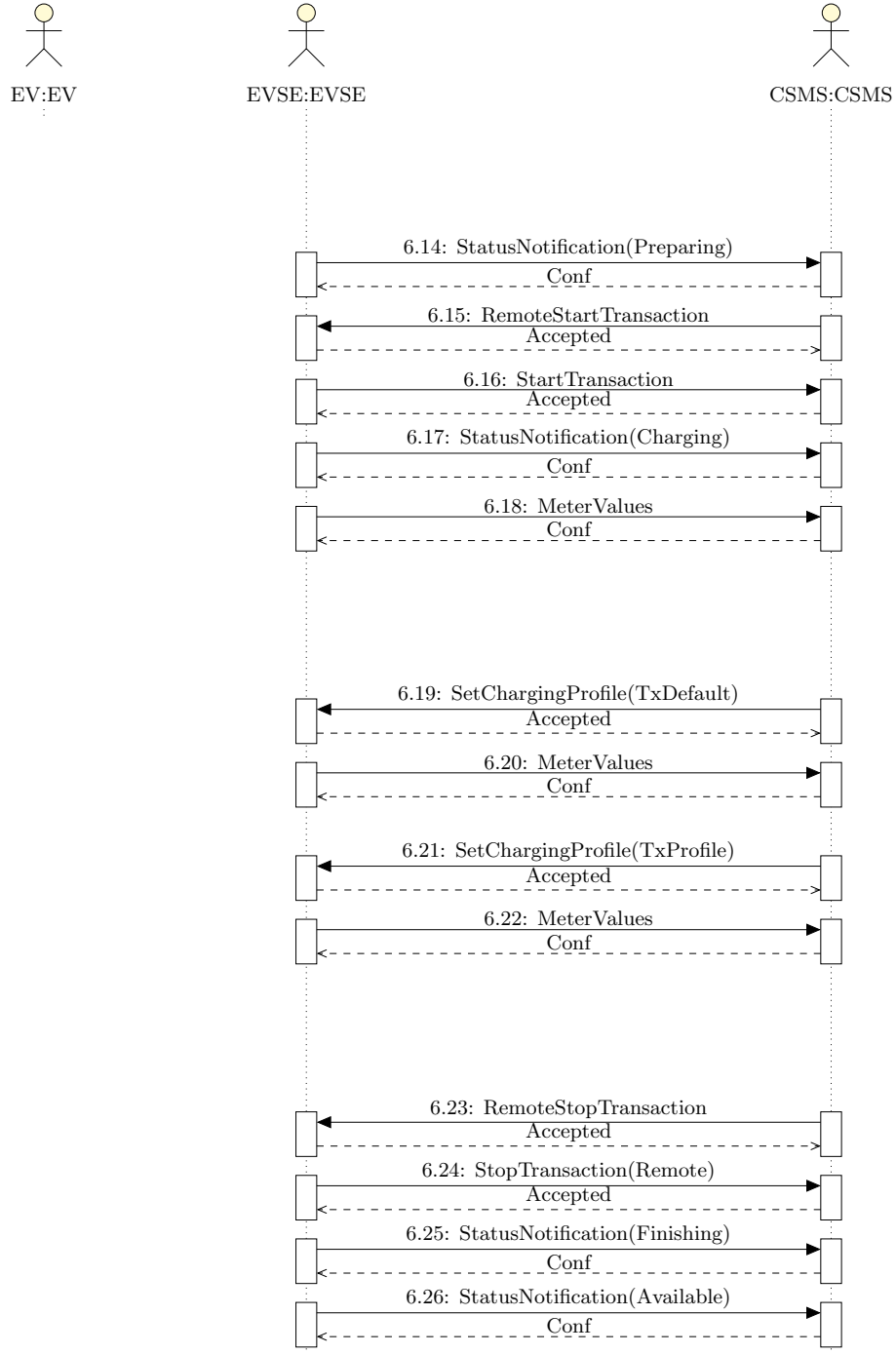
Figure 6.12: Charging Profile Verification (Part 2)
