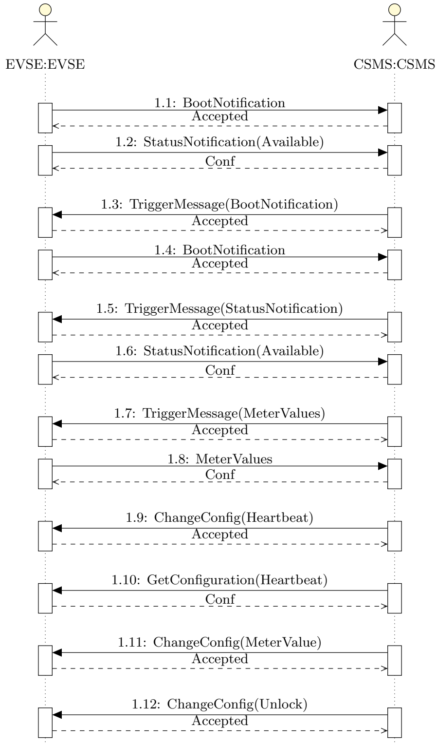
Figure 6.1: Configuration Verification (Part 1)
