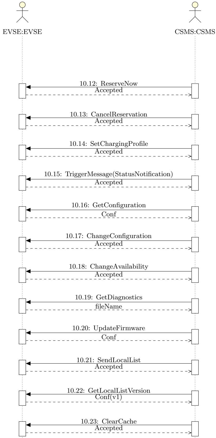
Figure 6.26: Summary Verification (Part 2)
