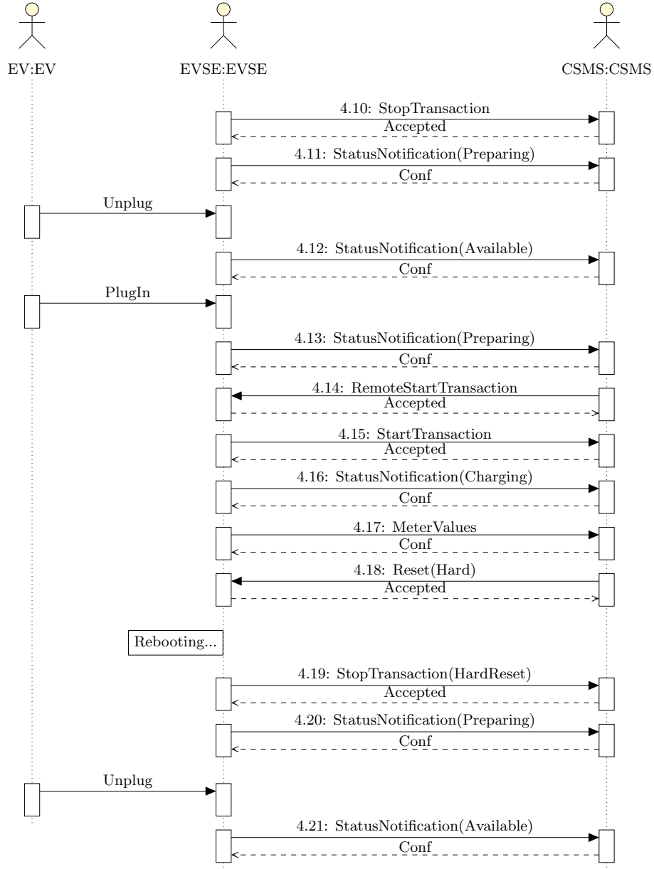
Figure 6.8: Reset Verification (Part 2)
