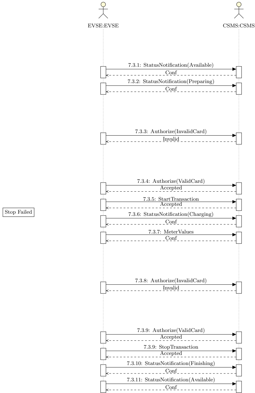
Figure 6.15: Swap Card Sequence
