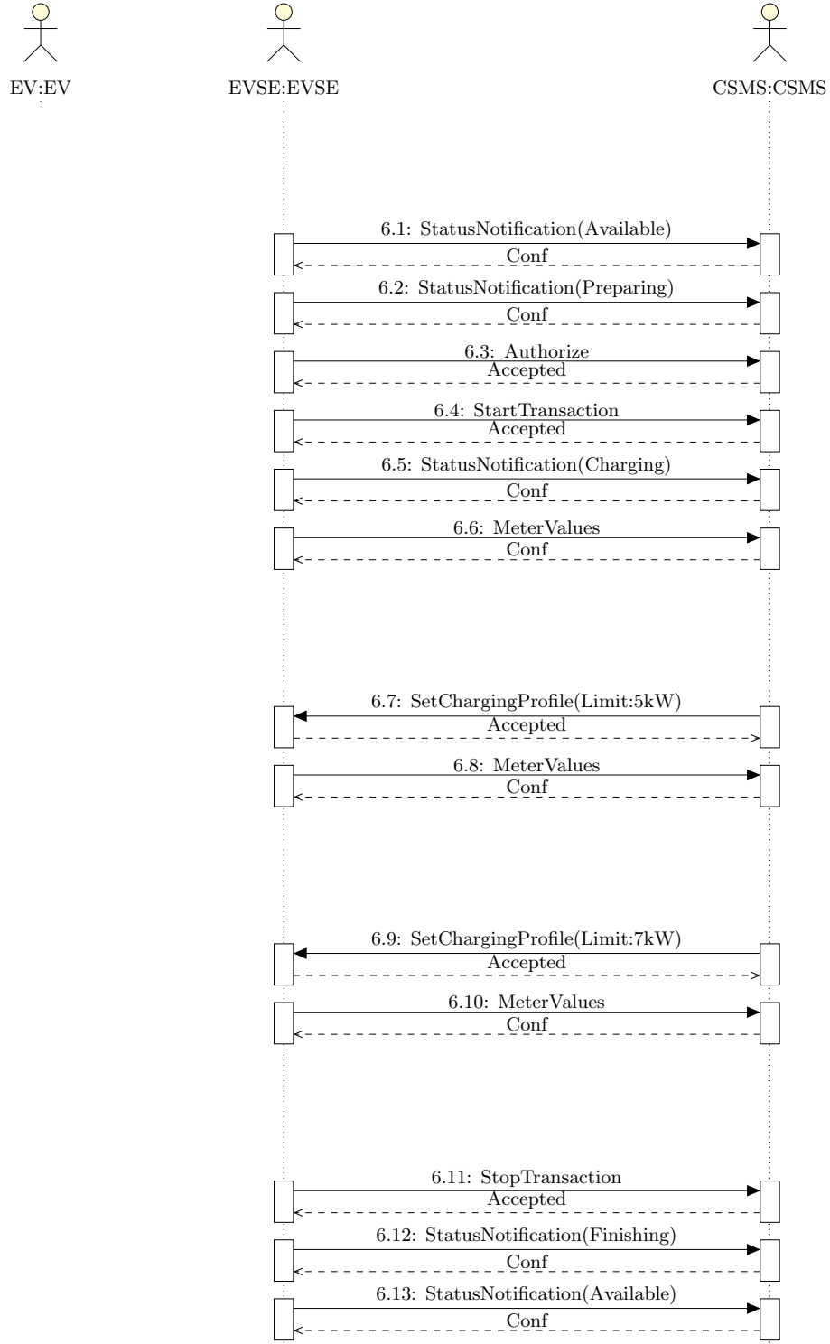
Figure 6.11: Charging Profile Verification (Part 1)
