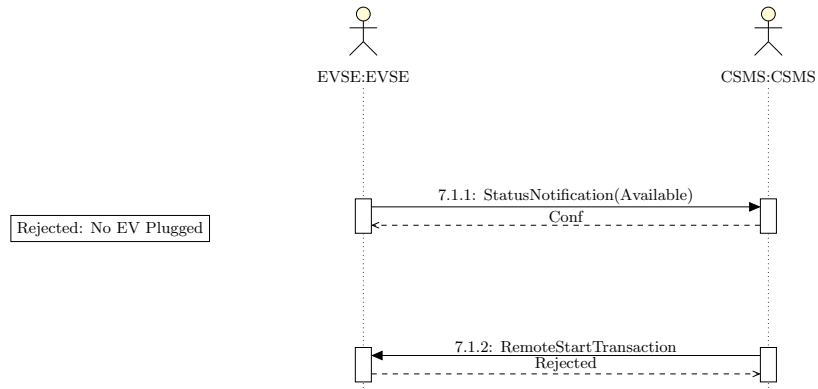
Figure 6.13: Remote Start (Unplugged) Sequence
