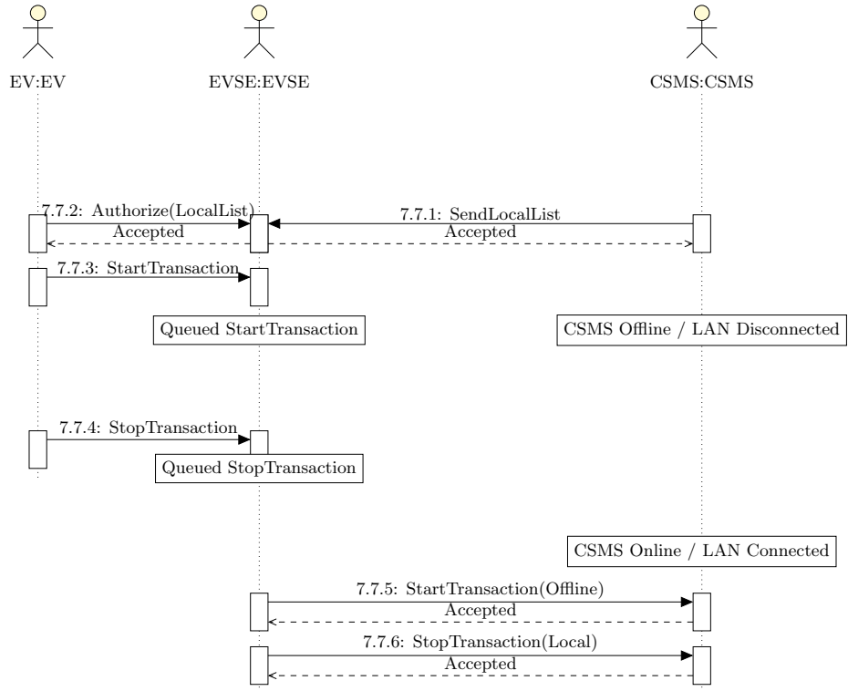
Figure 6.19: Local List (Offline) Sequence
