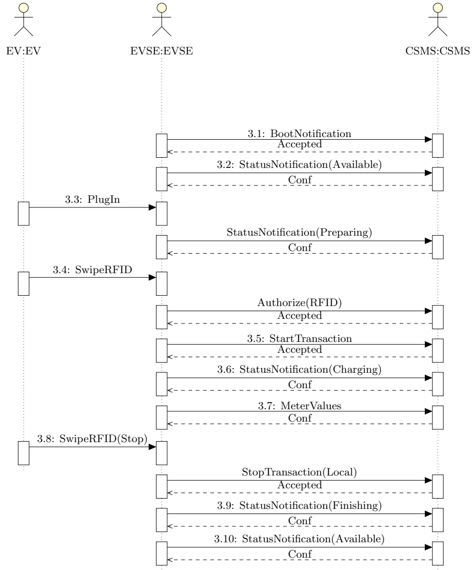
Figure 6.5: Normal Operation Verification (Part 1)
