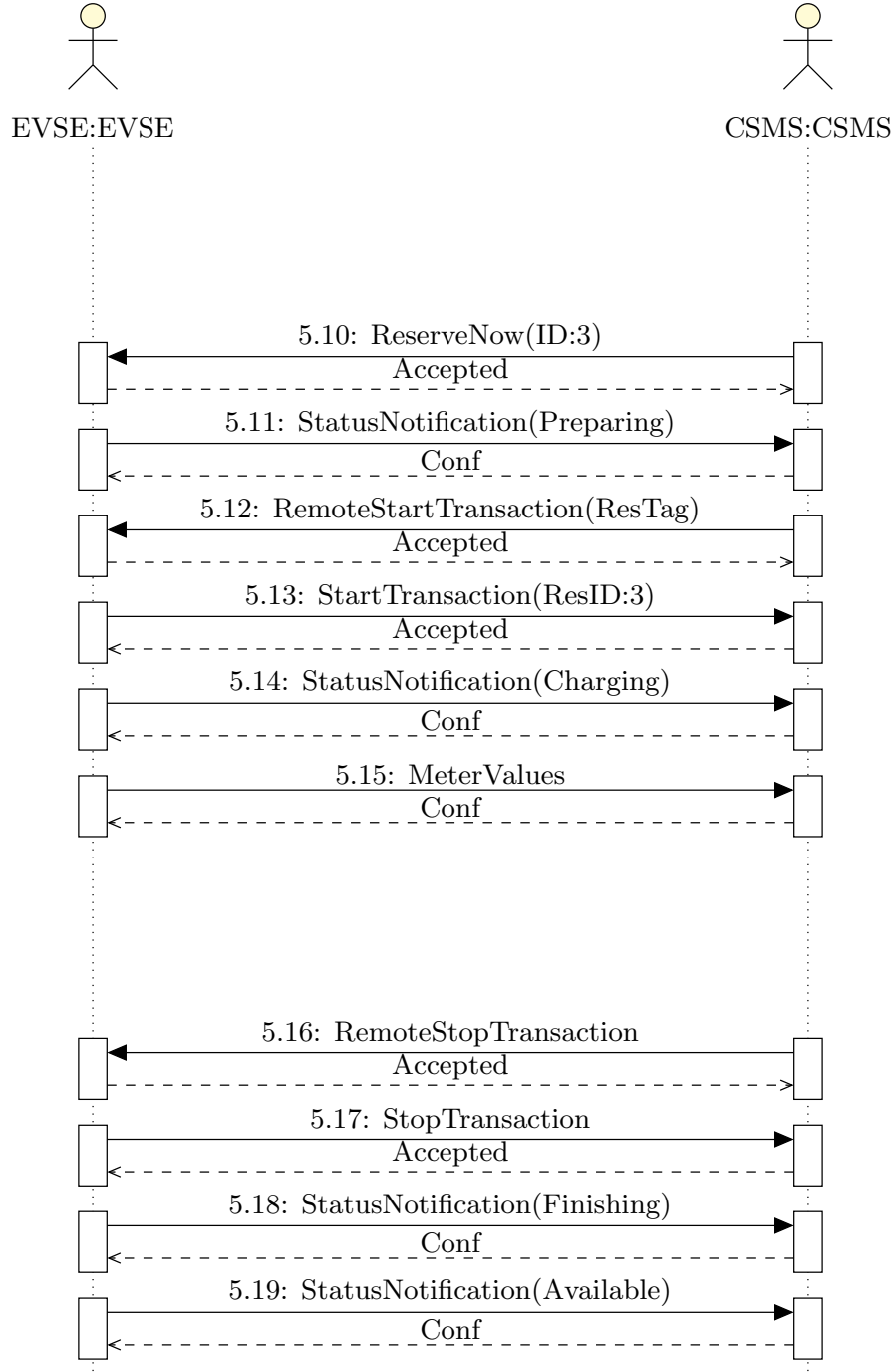
Figure 6.10: Reservation Verification (Part 2)
