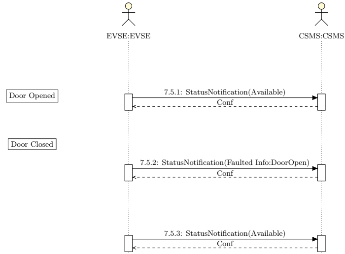
Figure 6.17: Open Door Fault Sequence
