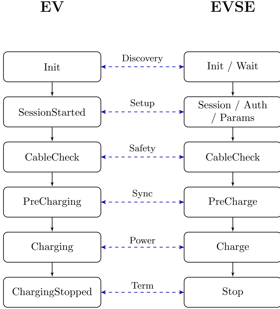
Figure 3.4: EV-EVSE State Synchronization
