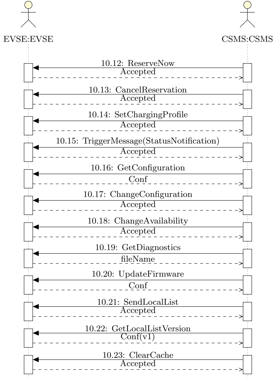
Figure 6.30: Summary Verification (Part 2)
