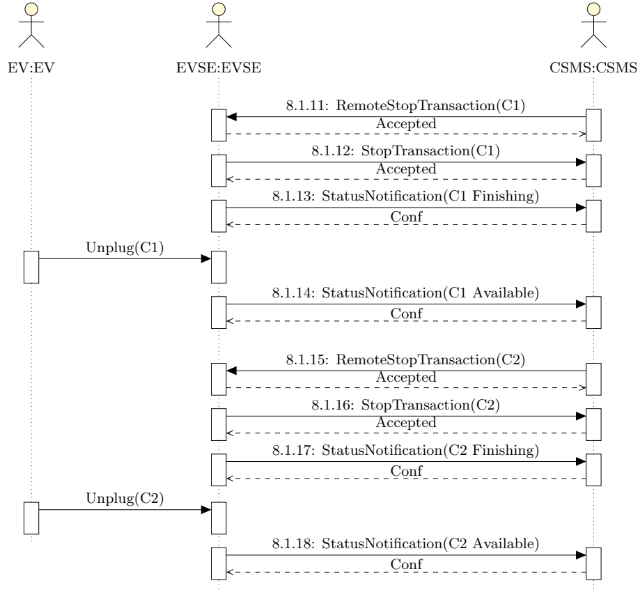
Figure 6.22: Dual Concurrent Sequence (Part 2)
