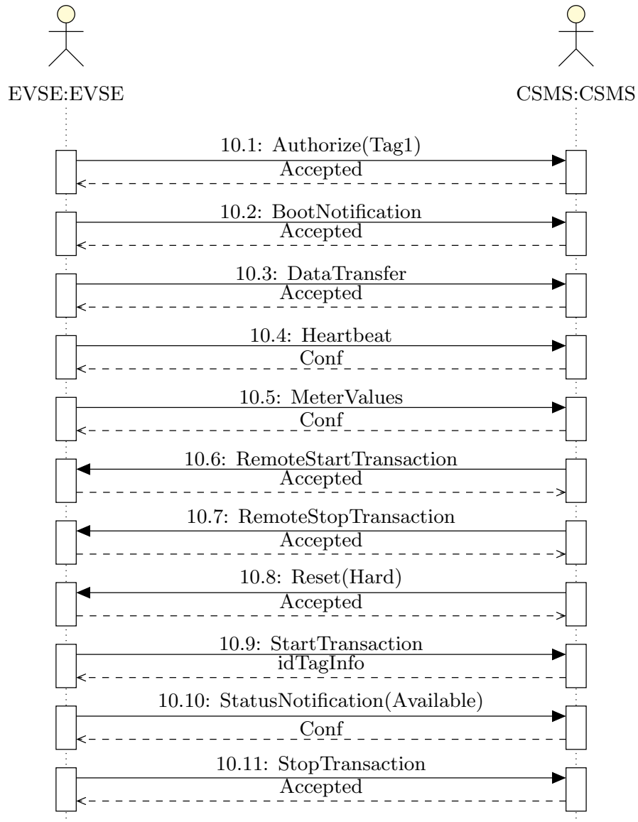
Figure 6.29: Summary Verification (Part 1)
