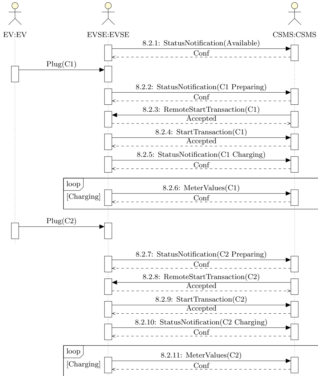
Figure 6.23: Dual Connector Emergency Stop Sequence Part 1
