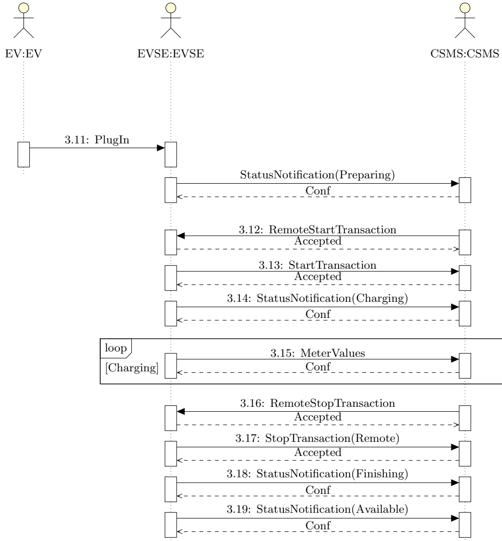
Figure 6.7: Normal Operation Verification (Part 2)
