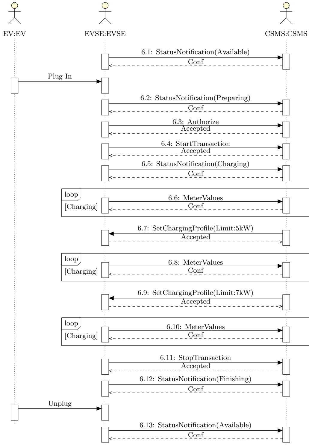
Figure 6.12: Charging Profile Verification (Part 1)
