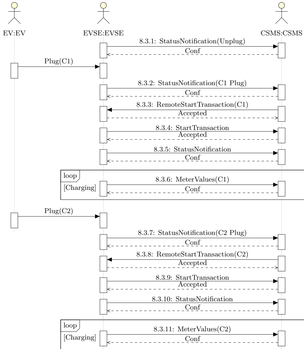
Figure 6.25: Dual Power Loss Sequence Part 1
