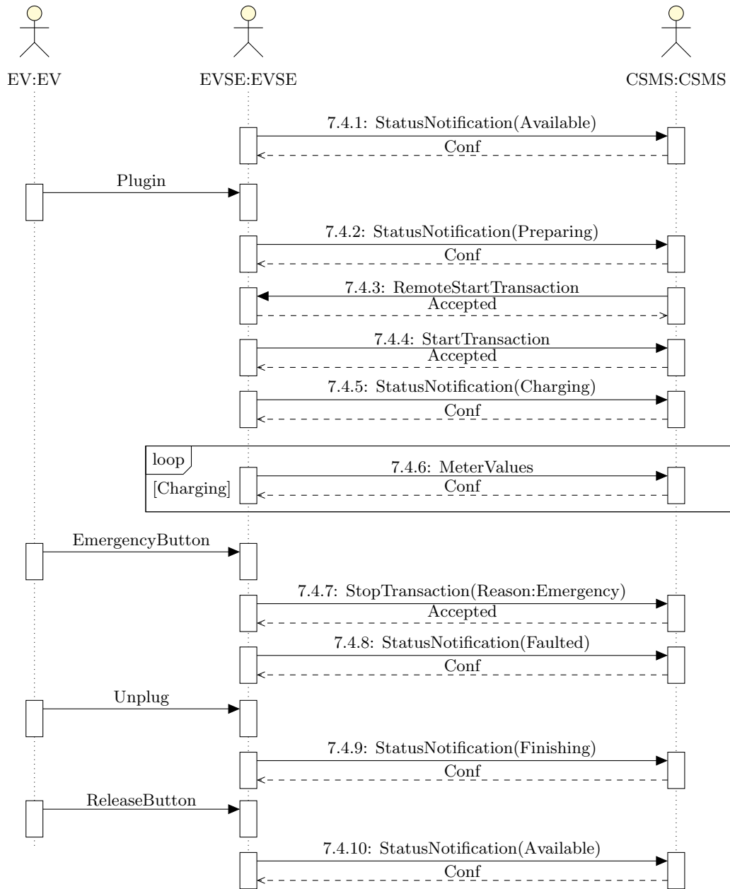
Figure 6.17: Emergency Stop Sequence
