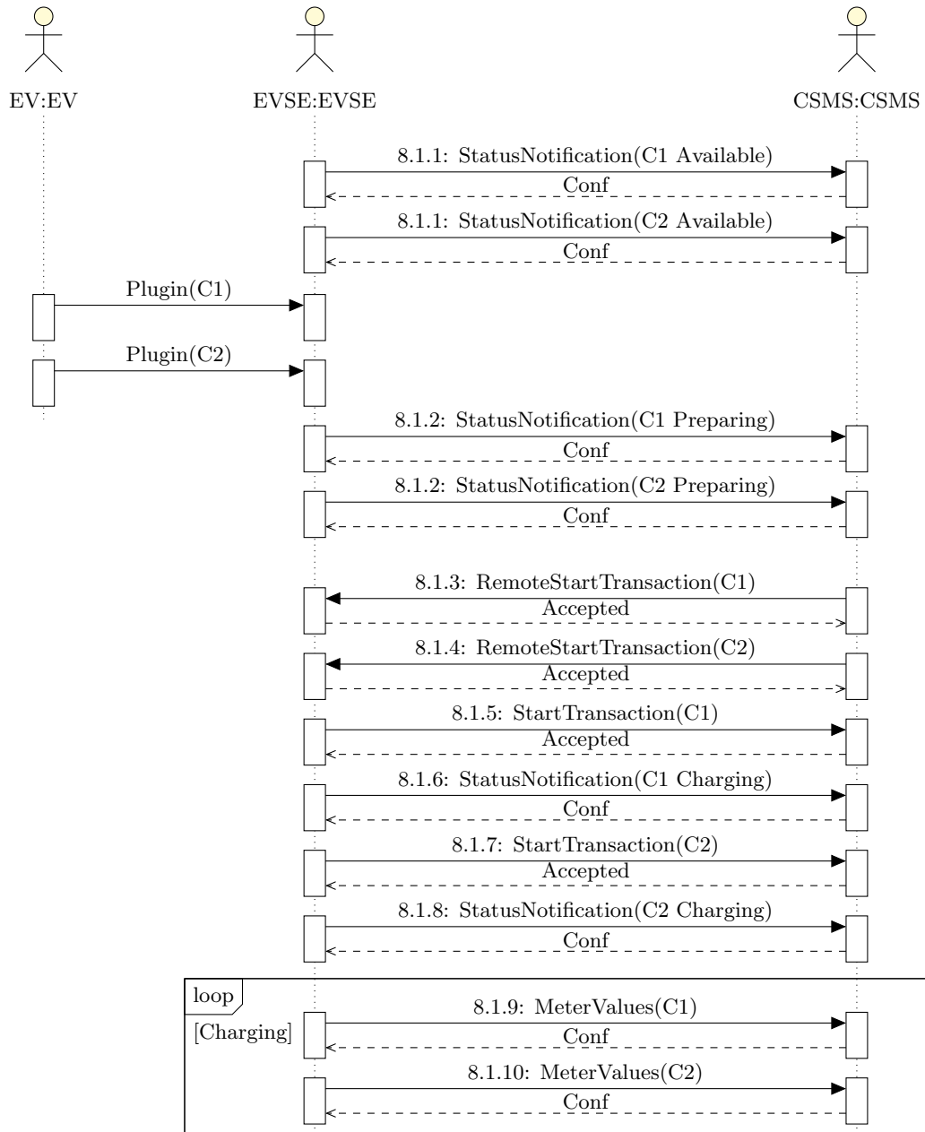
Figure 6.21: Dual Concurrent Sequence (Part 1)
