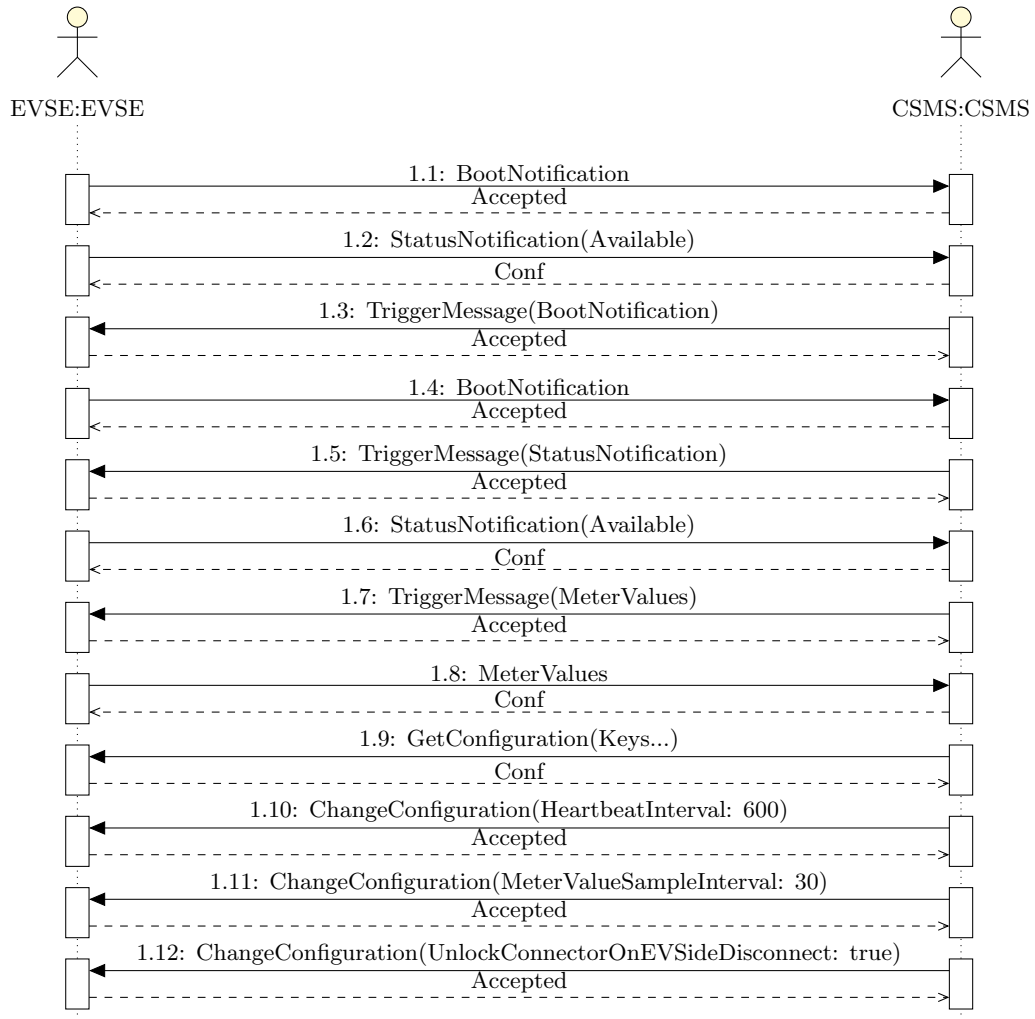
Figure 6.2: Configuration Verification (Part 1)
