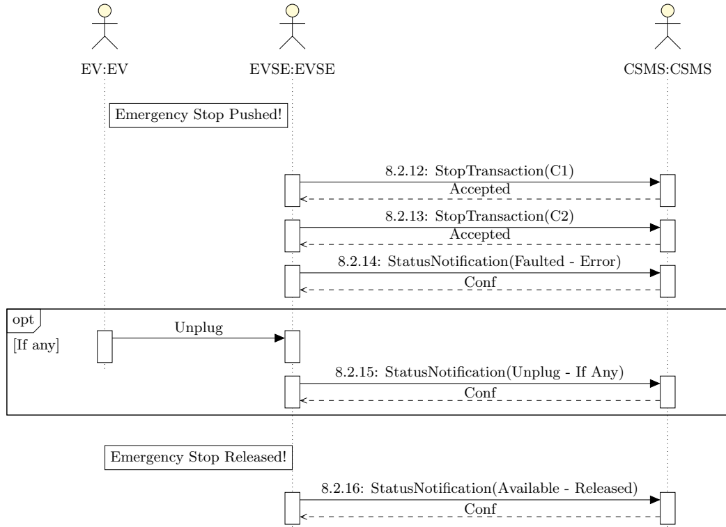
Figure 6.24: Dual Emergency Stop Sequence
