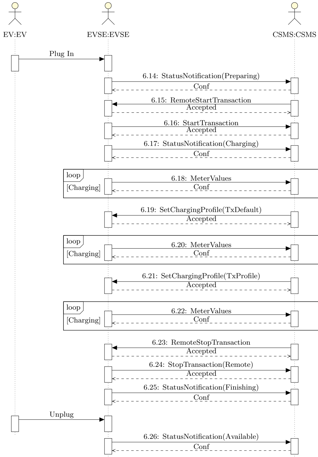
Figure 6.13: Charging Profile Verification (Part 2)
