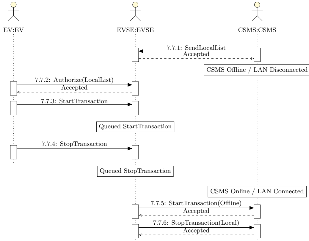
Figure 6.20: Local List (Offline) Sequence
