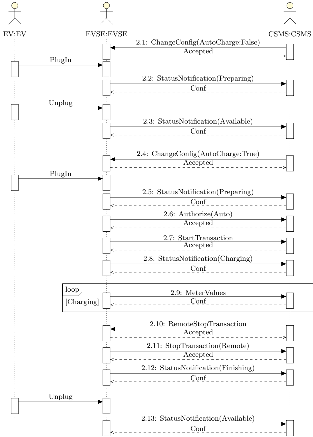
Figure 6.4: Auto Charge Verification (Part 1)
