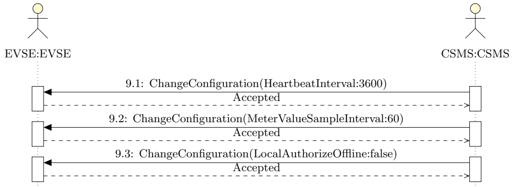
Figure 6.27: MEA General Configuration Sequence
