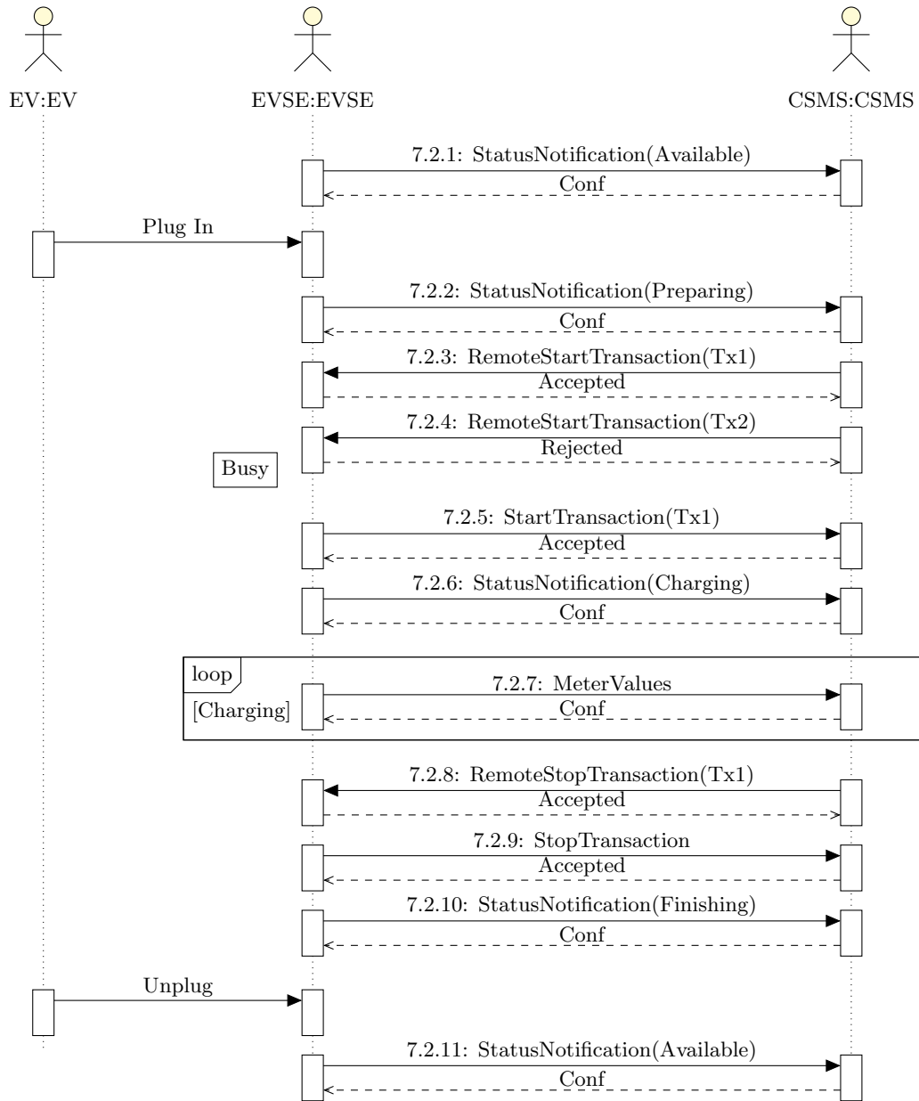
Figure 6.15: Concurrent Remote Start Sequence
