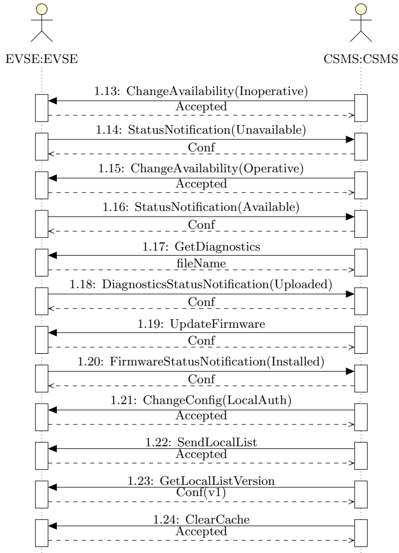
Figure 6.3: Configuration Verification (Part 2)
