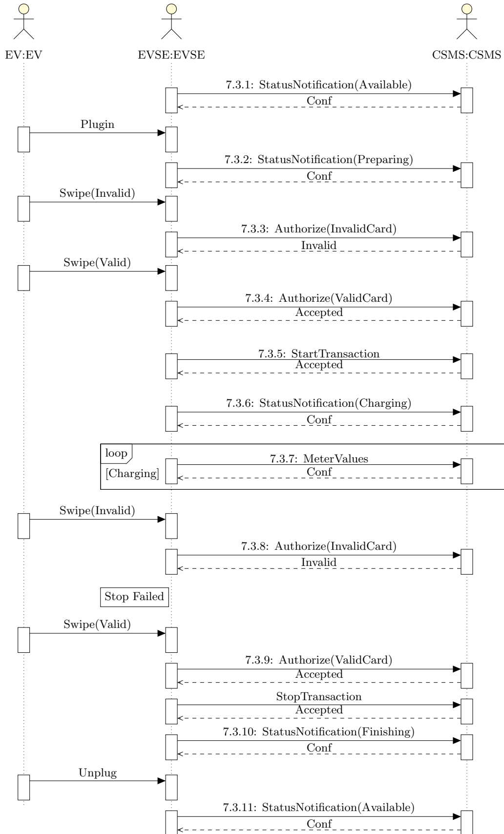
Figure 6.16: Swap Card Sequence
