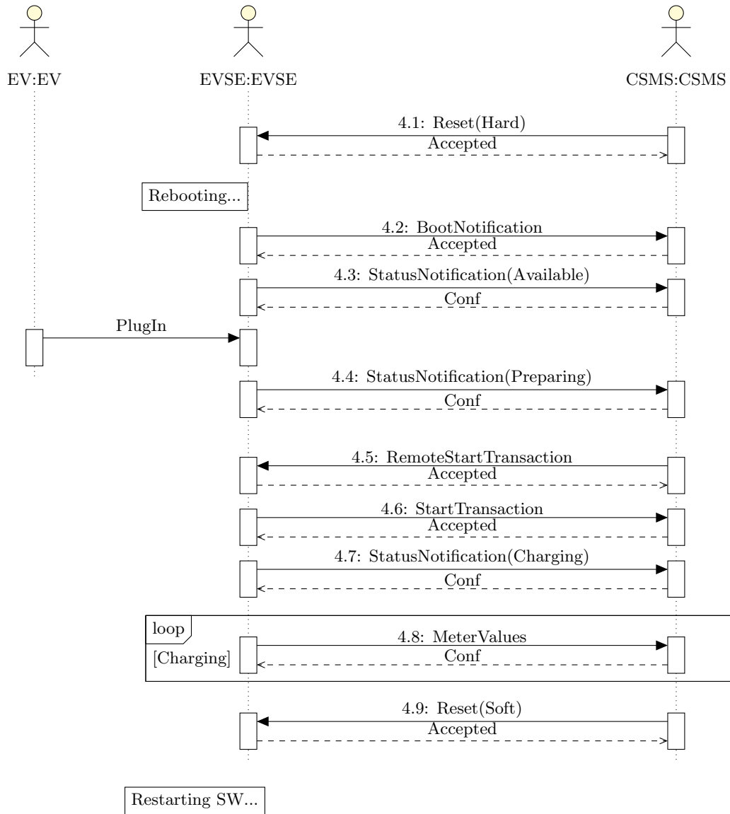
Figure 6.8: Reset Verification (Part 1)
