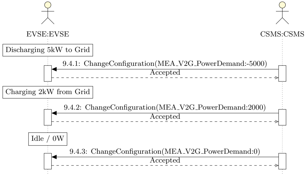
Figure 6.28: Power Demand Verification Sequence
