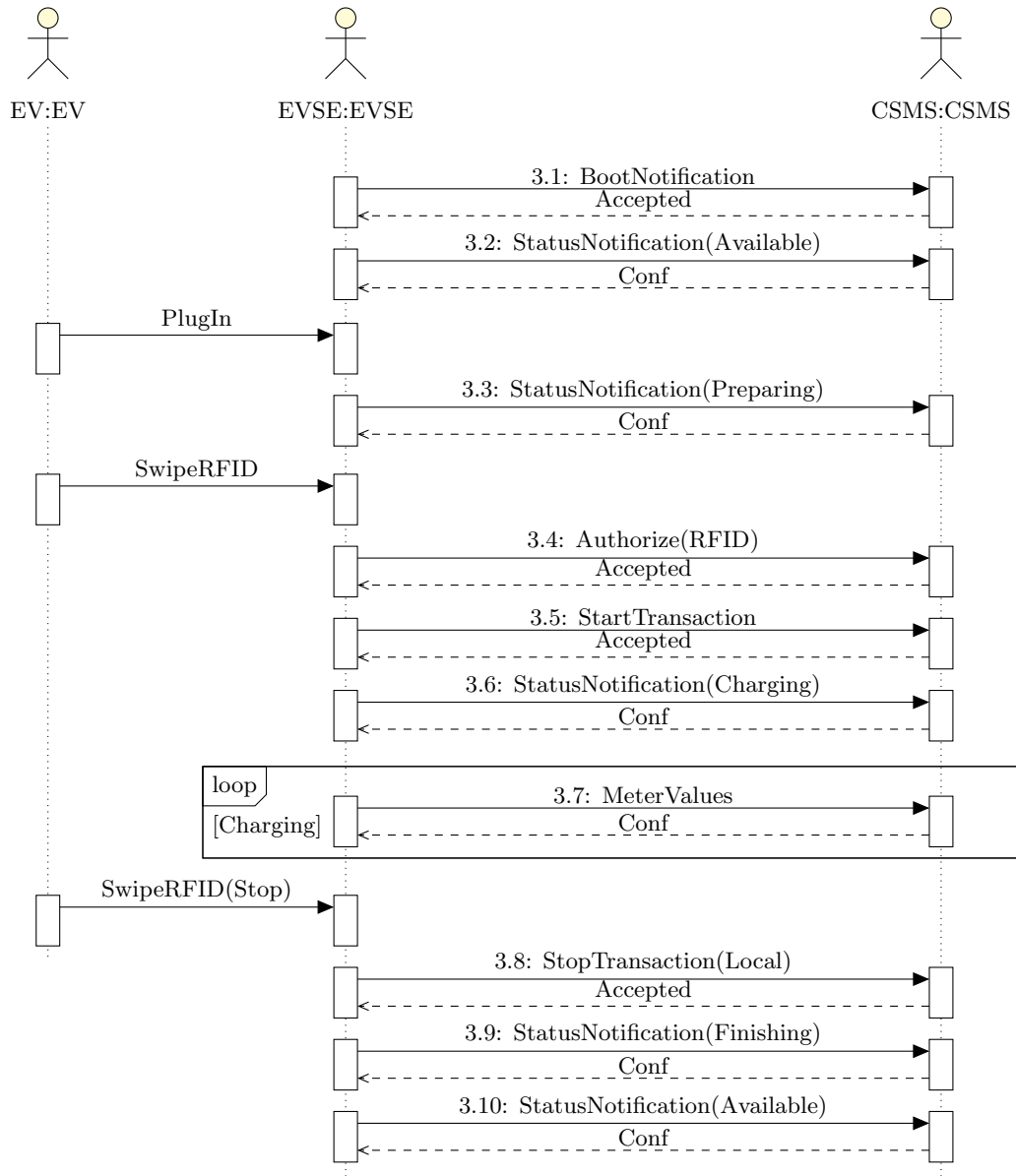
Figure 6.6: Normal Operation Verification (Part 1)
