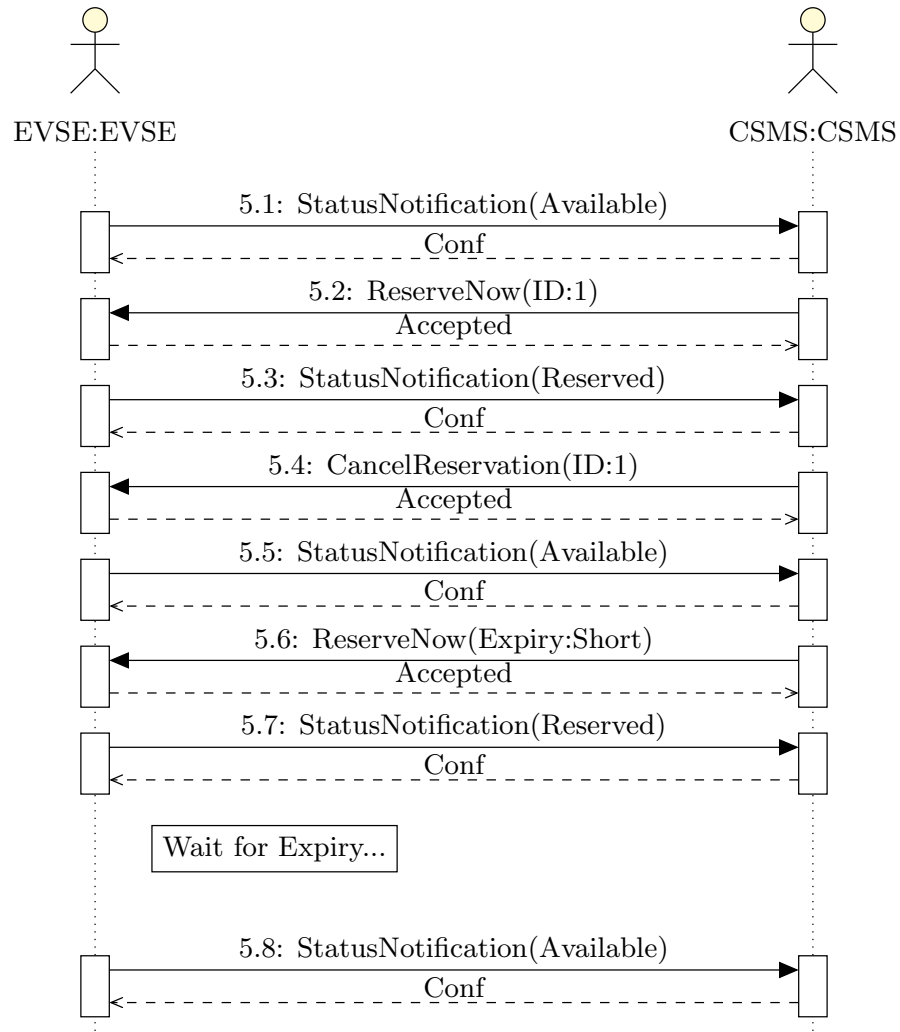
Figure 6.10: Reservation Verification (Part 1)
