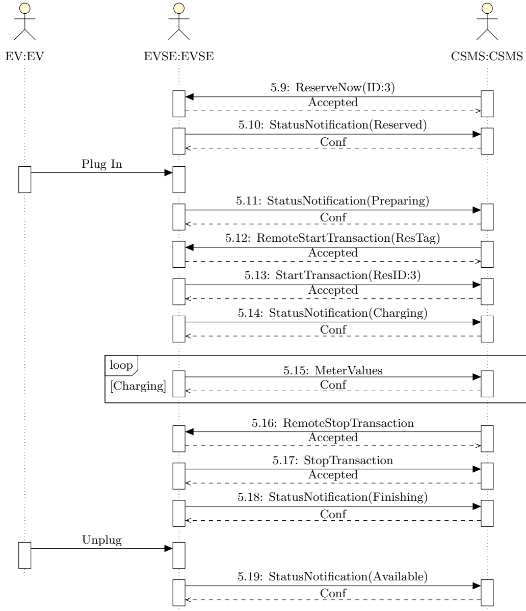
Figure 6.11: Reservation Verification (Part 2)
