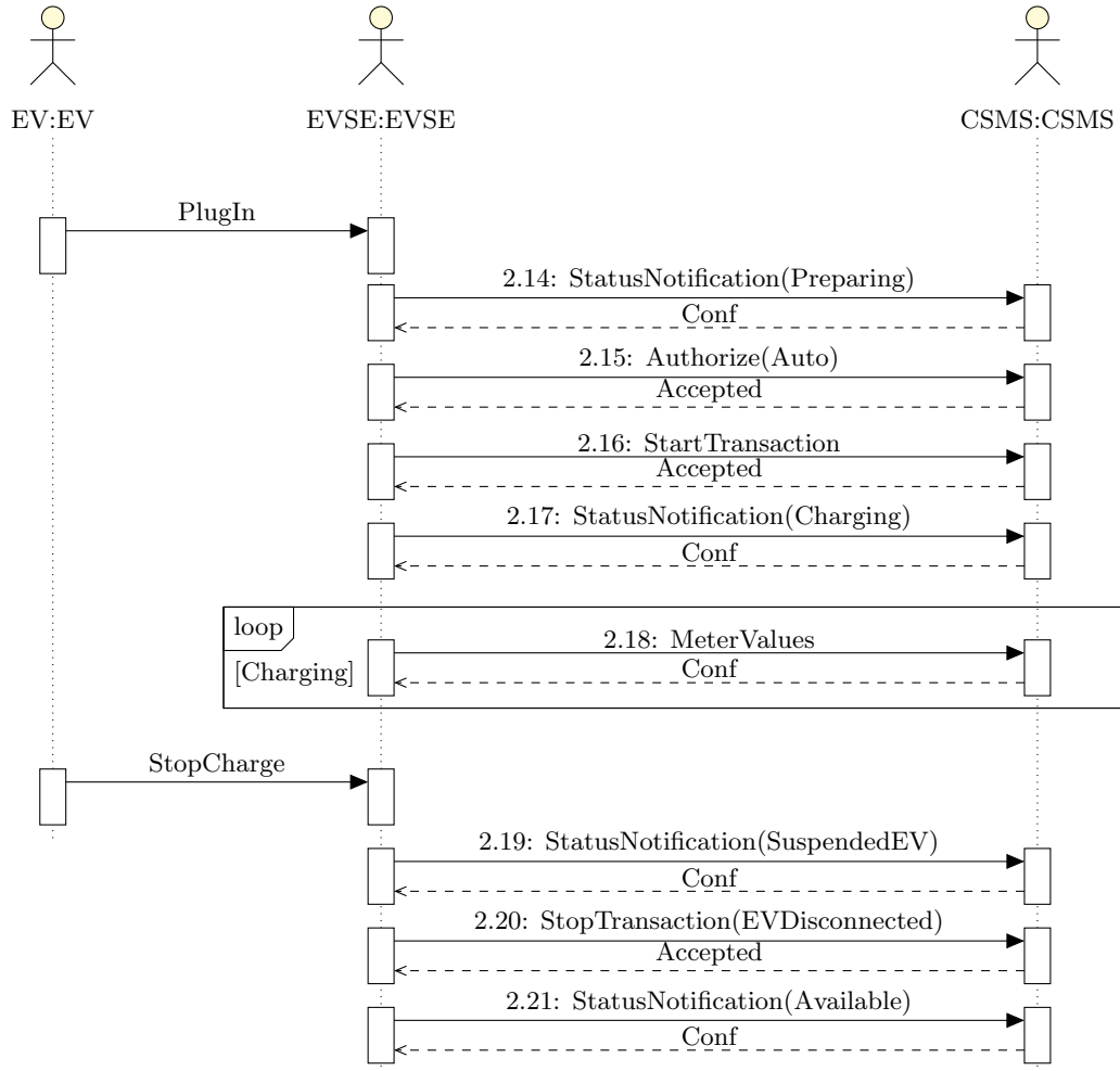
Figure 6.5: Auto Charge Verification (Part 2)
