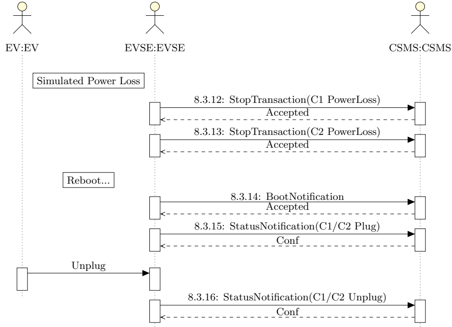
Figure 6.26: Dual Power Loss Sequence Part 2
