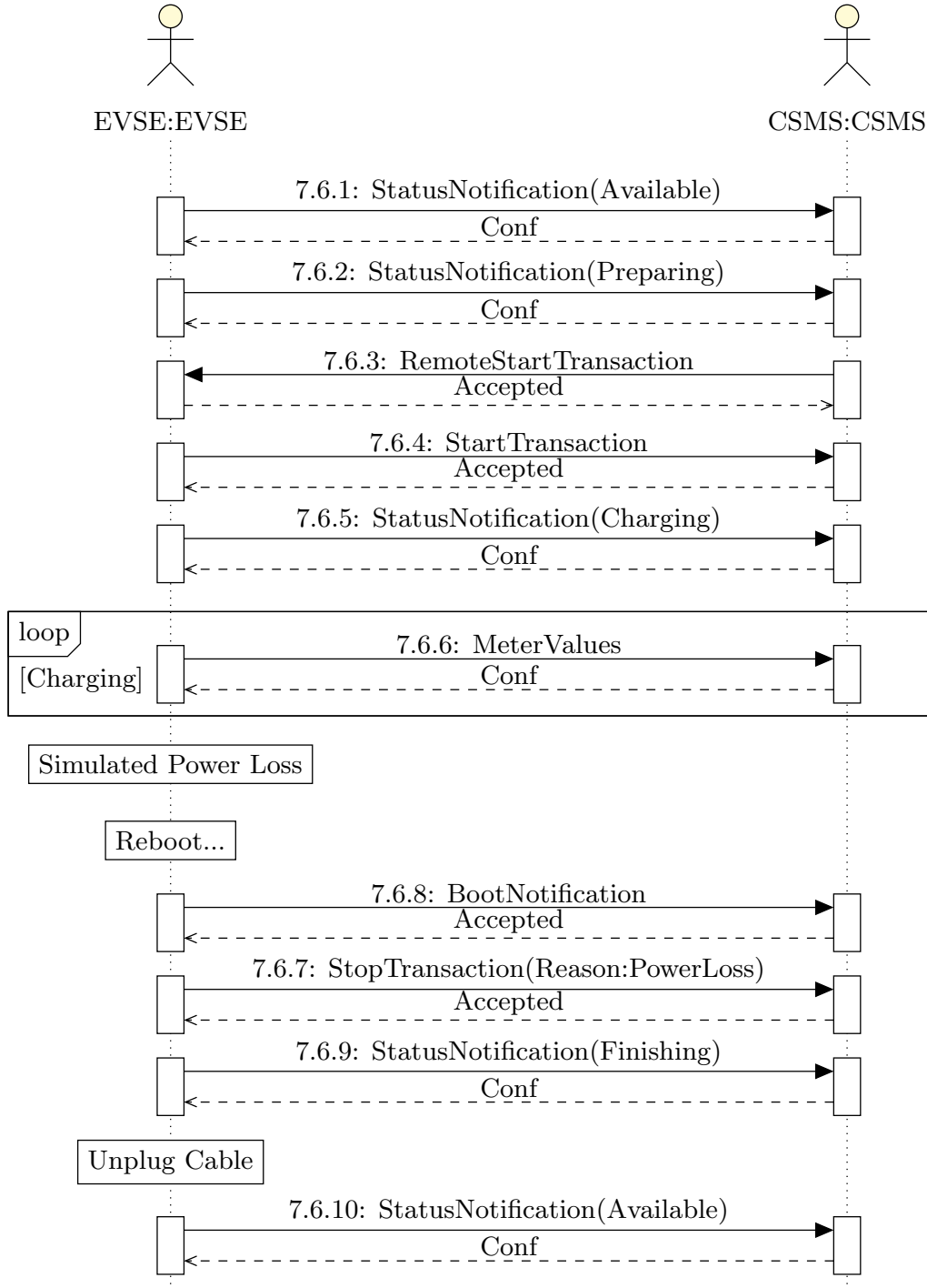
Figure 6.19: Power Loss Recovery Sequence
