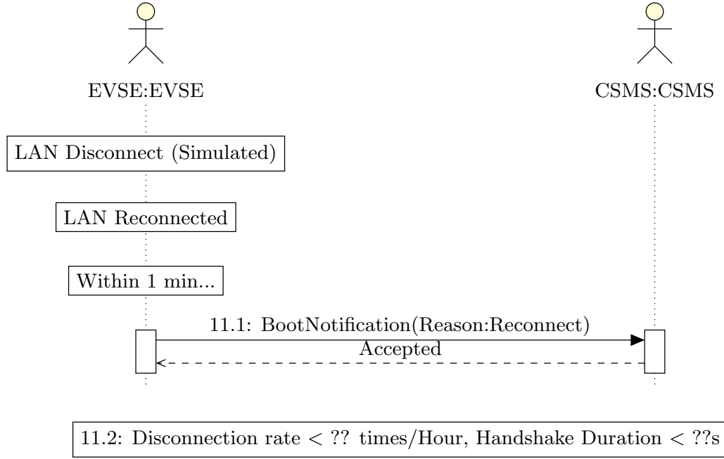
Figure 6.31: LAN Disconnect/Reconnect Sequence
