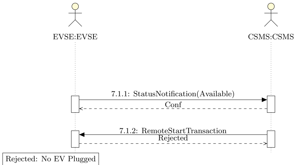
Figure 6.14: Remote Start (Unplugged) Sequence
