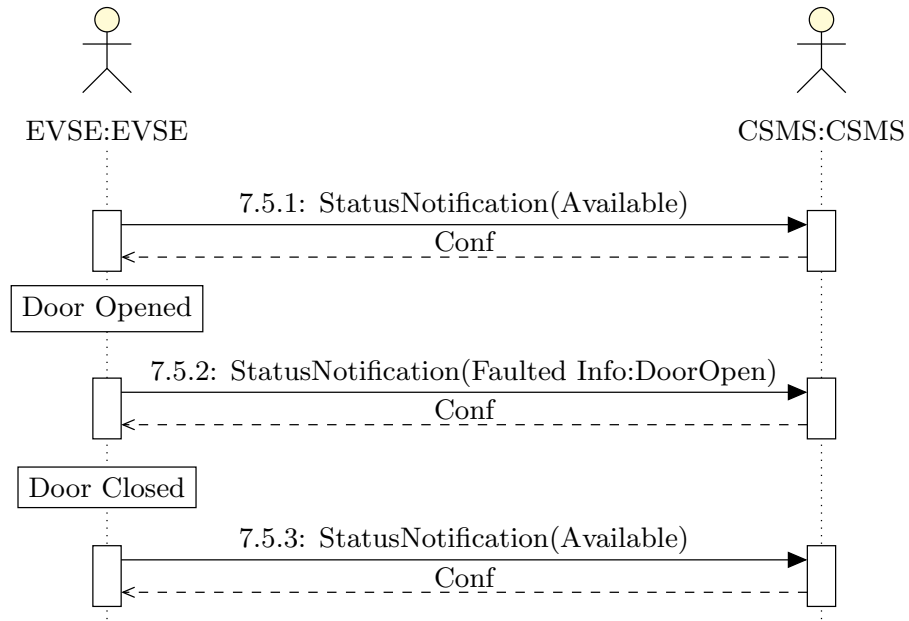
Figure 6.18: Open Door Fault Sequence
