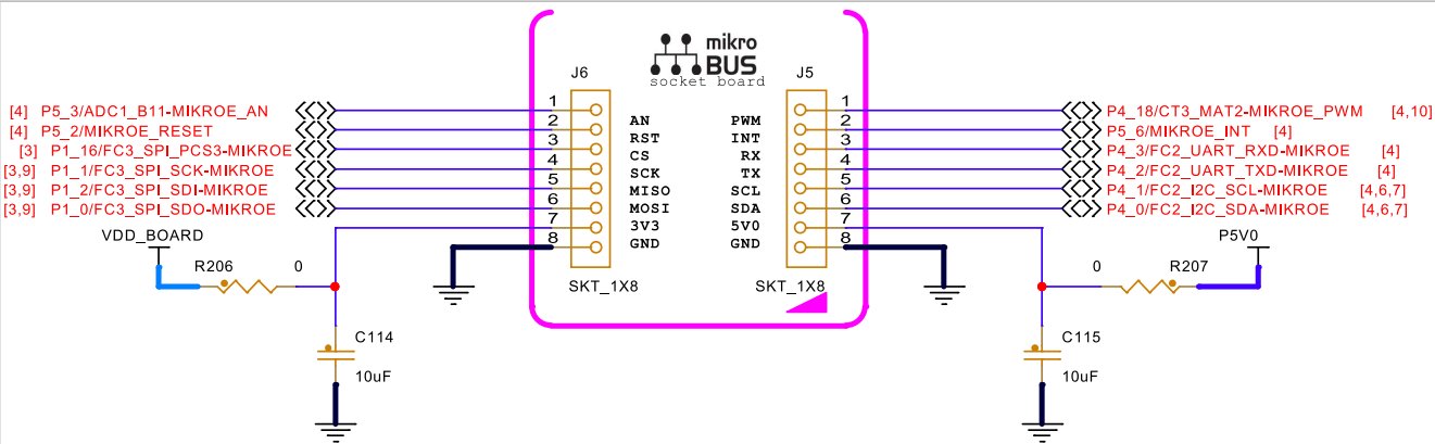
Figure 18. mikroBUS header pinout
