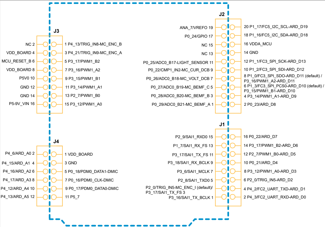
Figure 17. Arduino socket connector pinout
