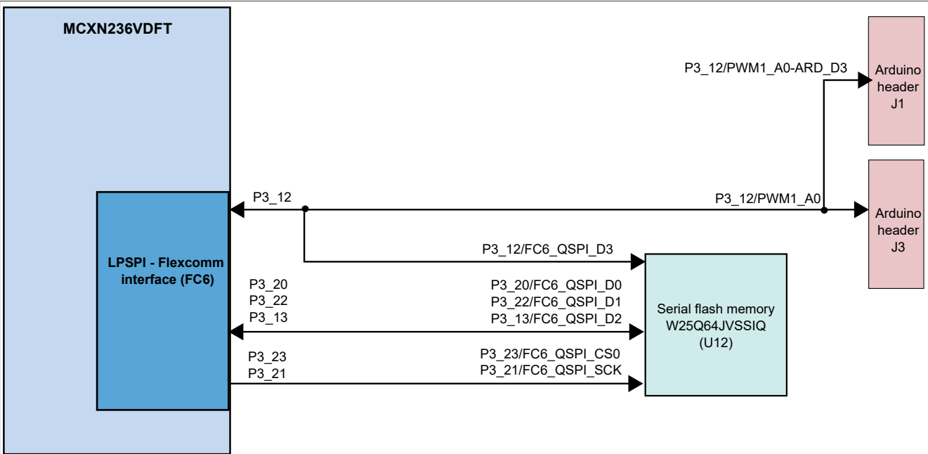
Figure 13. Flash memory circuit diagram
