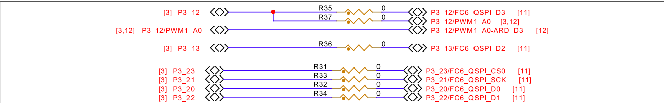
Figure 14. Isolation resistors for flash memory
