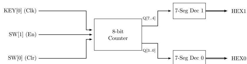
Figure 2: Top-level block diagram of the 8-bit counter.
