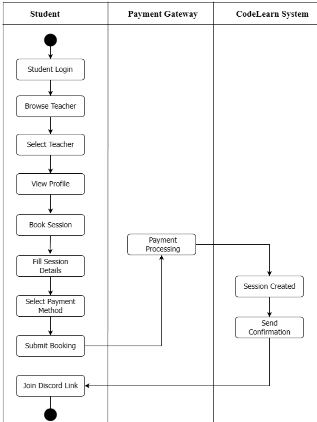
CODELEARN : USER ACTIVITY DIAGRAM
