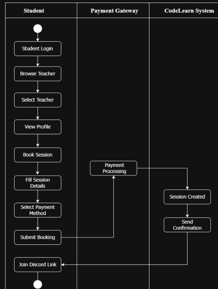
CODELEARN : USER ACTIVITY DIAGRAM
