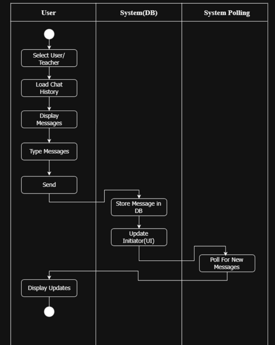
CODELEARN : CHAT ACTIVITY DIAGRAM
