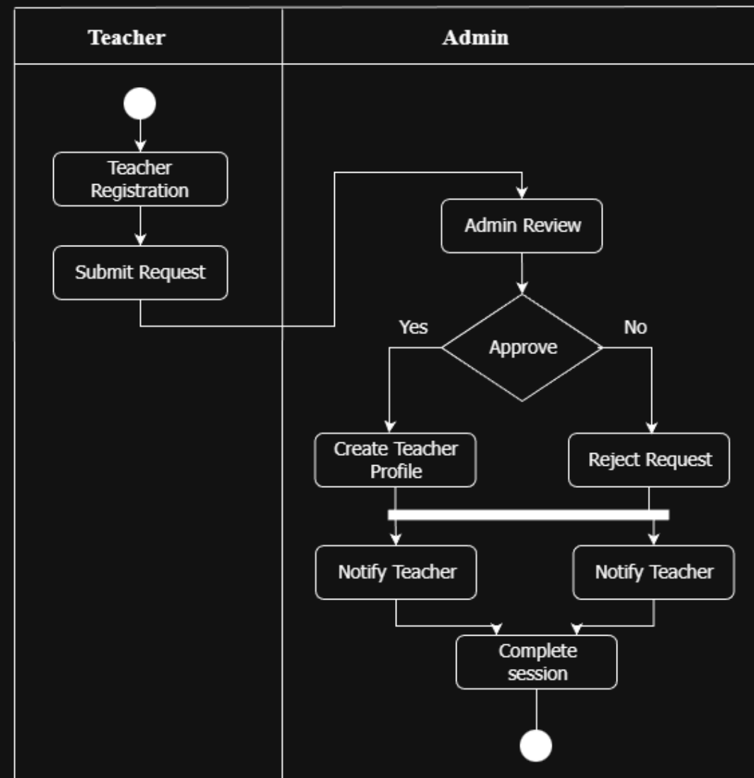
CODELEARN : TEACHER ACTIVITY DIAGRAM
