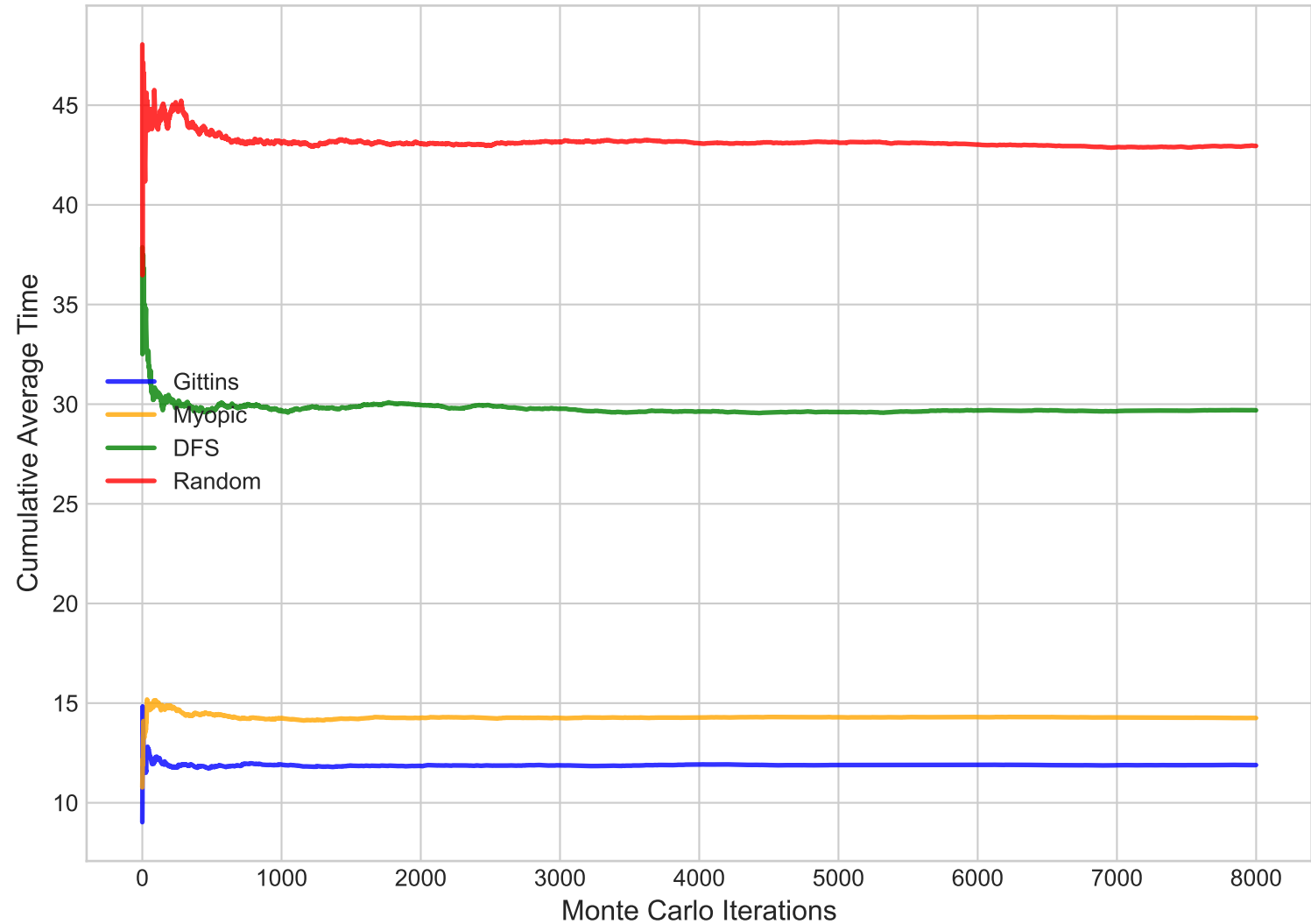
Expected Time-to-Compromise (Convergence)
