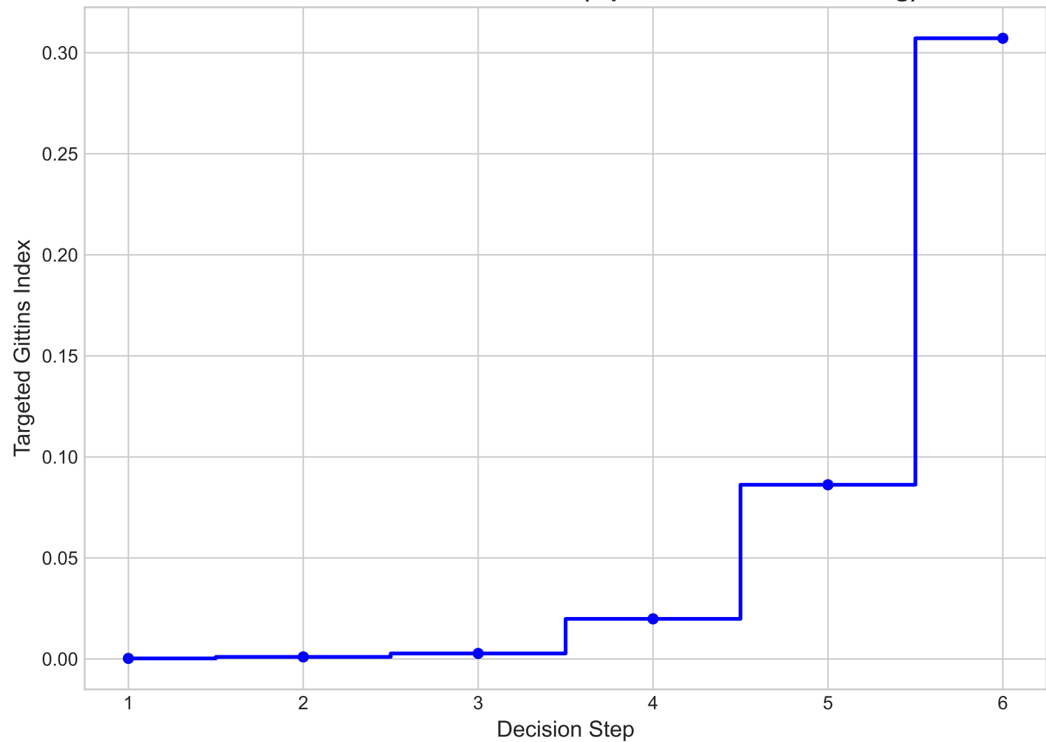
The Abandonment Threshold (Optimal Lateral Switching)
