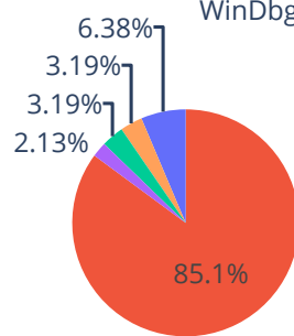
WinDbg
