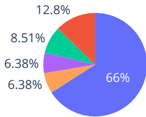
BugStalker
