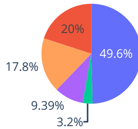
WinDbg
