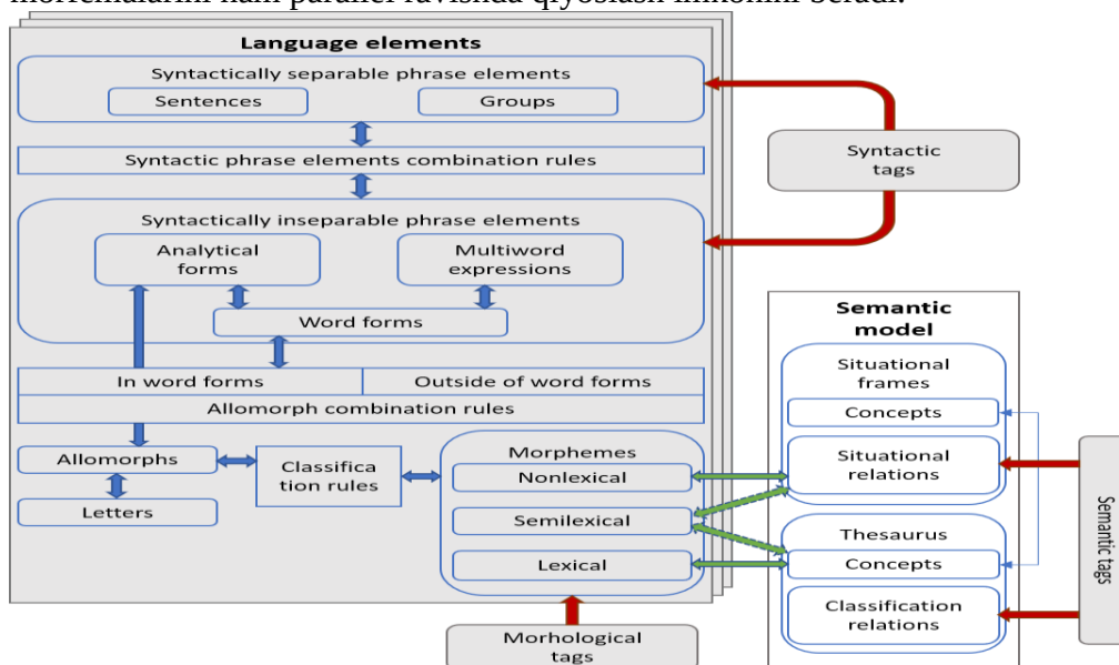
3-rasm. Turkiy morfemaning model tuzilishi.
