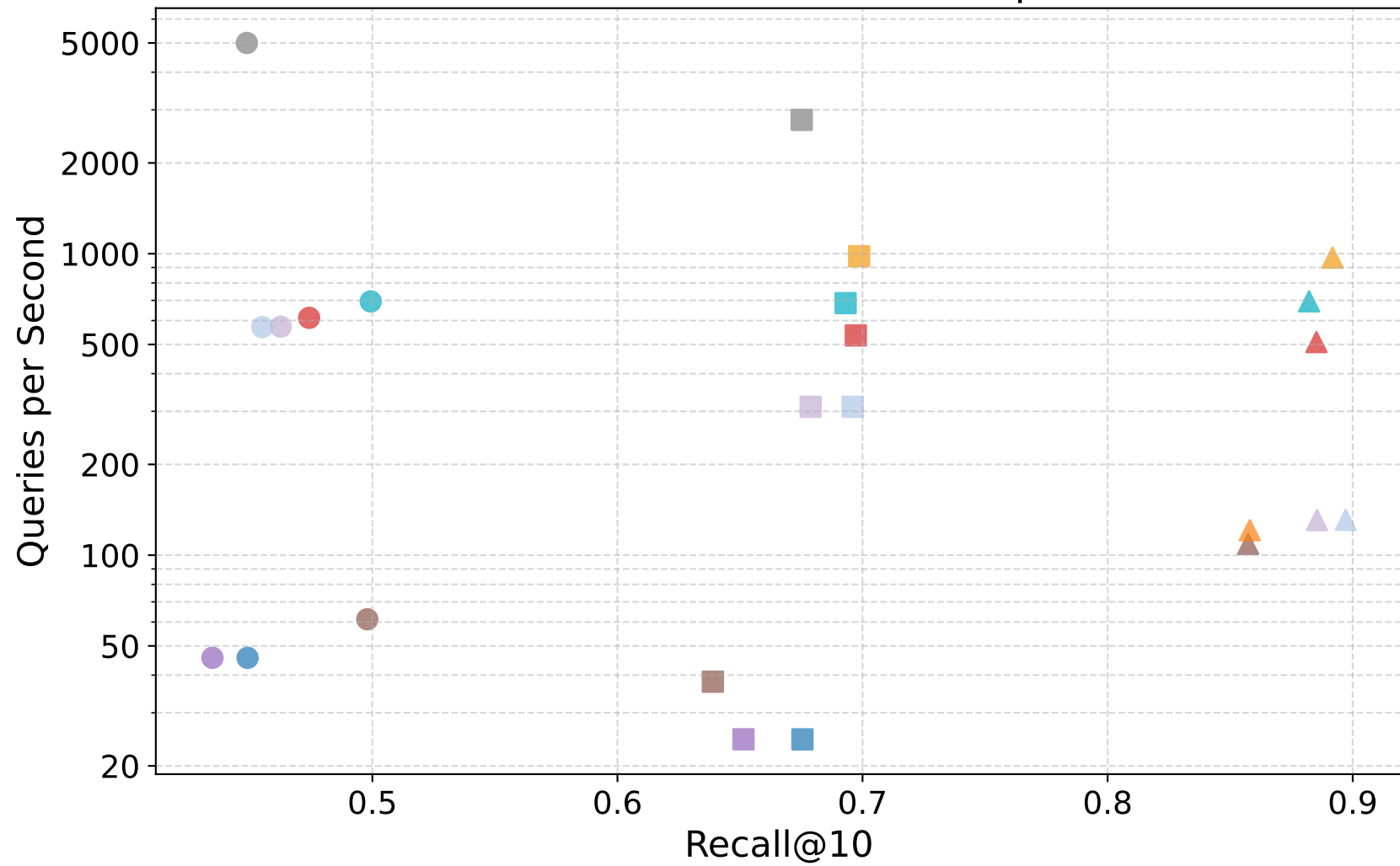
audio-128-euclidean — top10
