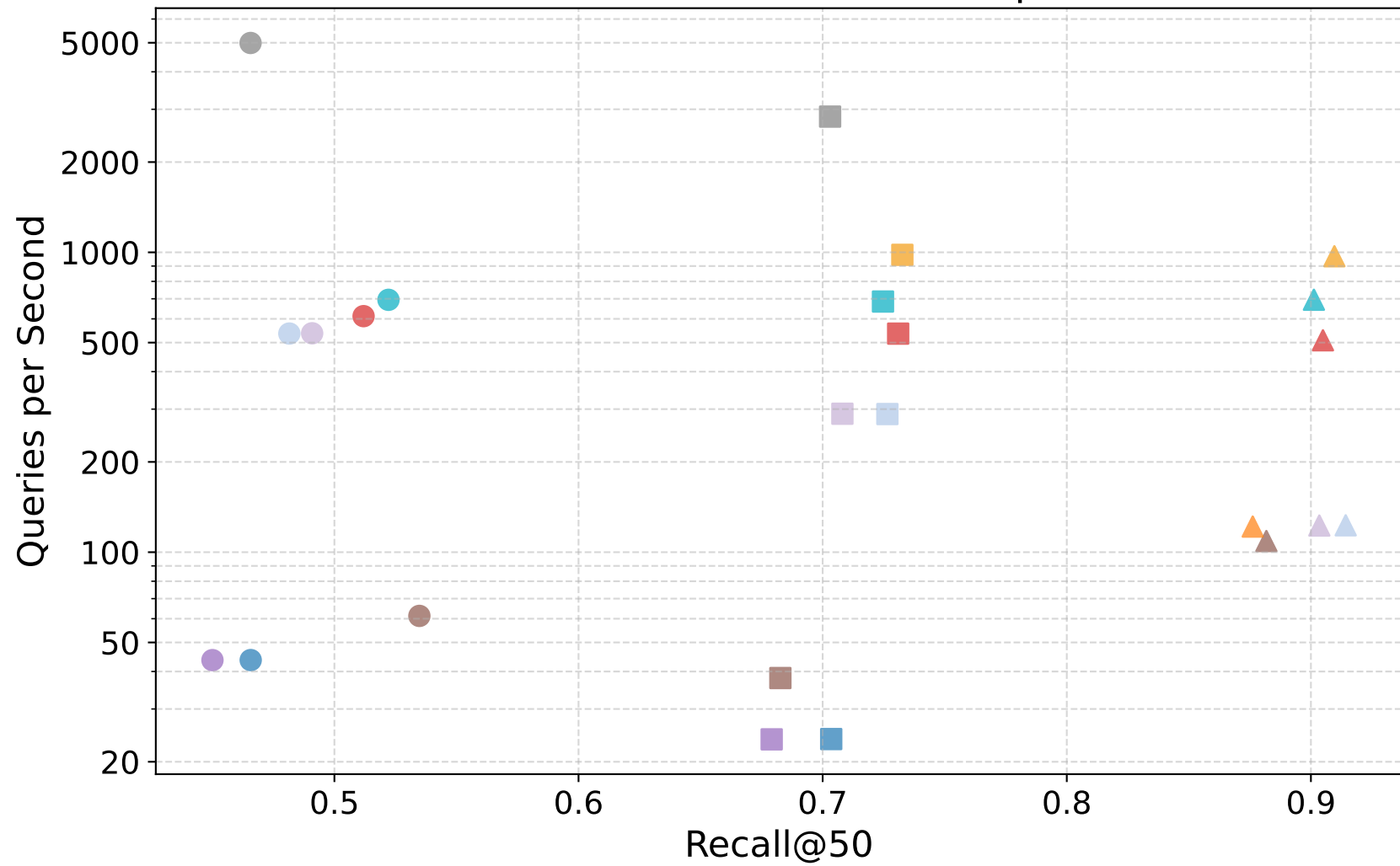
audio-128-euclidean — top50
