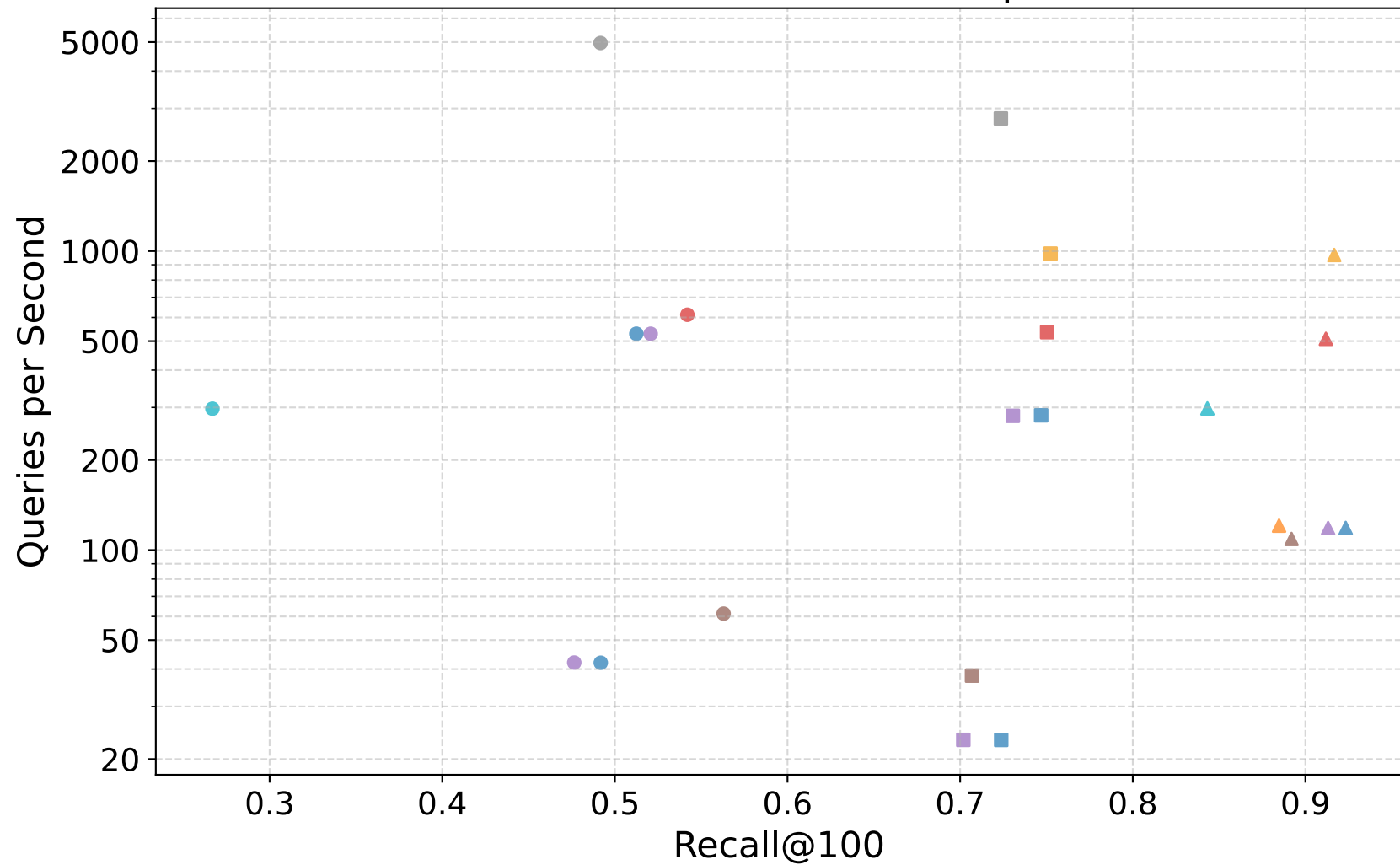
audio-128-euclidean — top100
