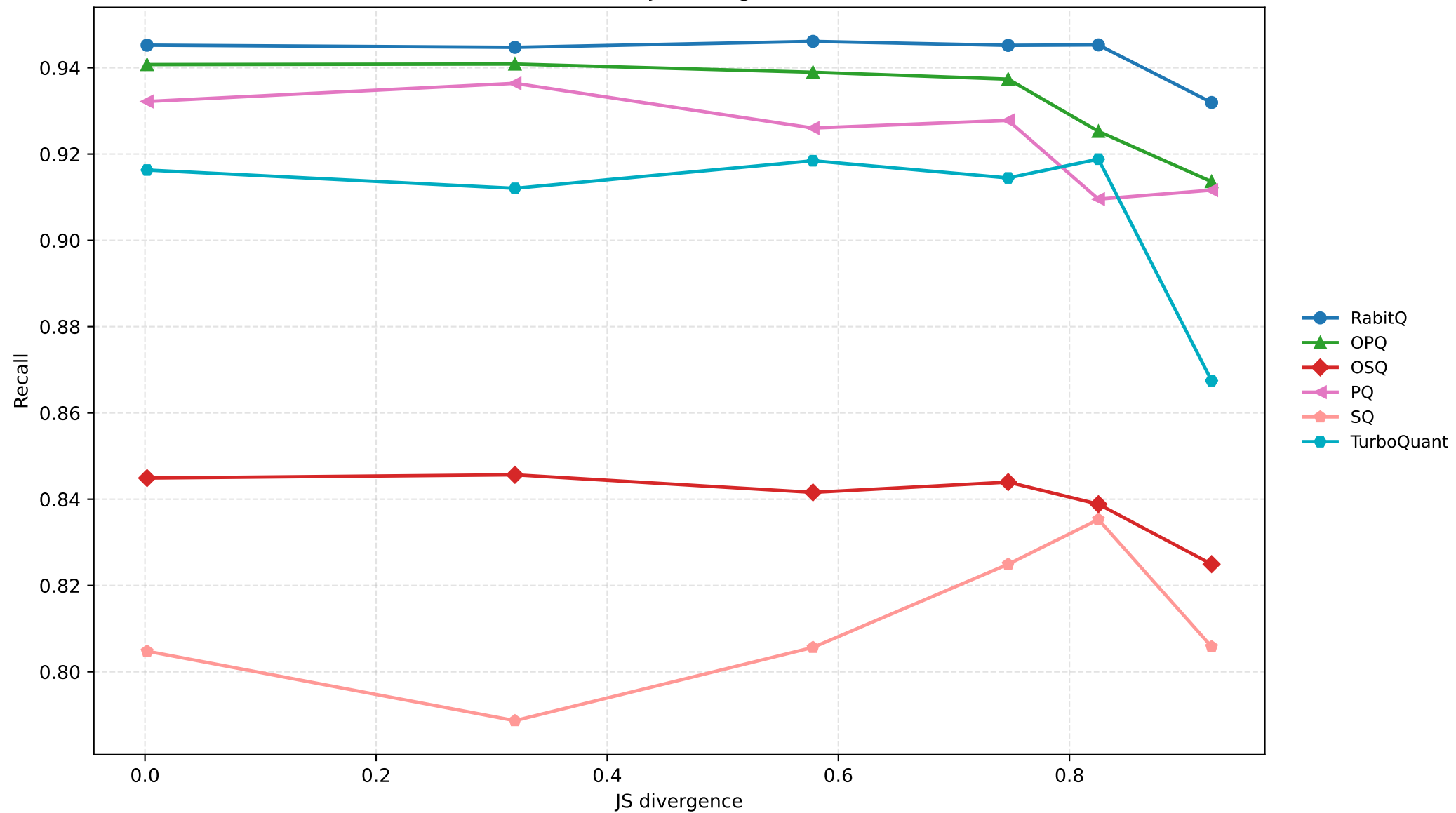
Distribution Shift: JS Divergence vs Recall
