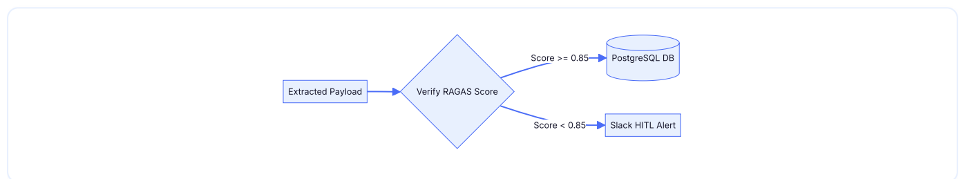
Figure 9.1: Proposed Confidence Gate Workflow. This diagram highlights how extracted payloads are routed depending on the composite RAGAS confidence score.
