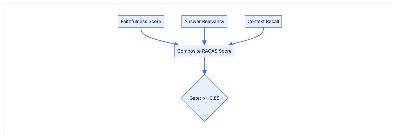
Figure 10.1: Proposed RAGAS Evaluation Pipeline. This diagram shows the three metrics combined into a single composite score to gate database writes.
