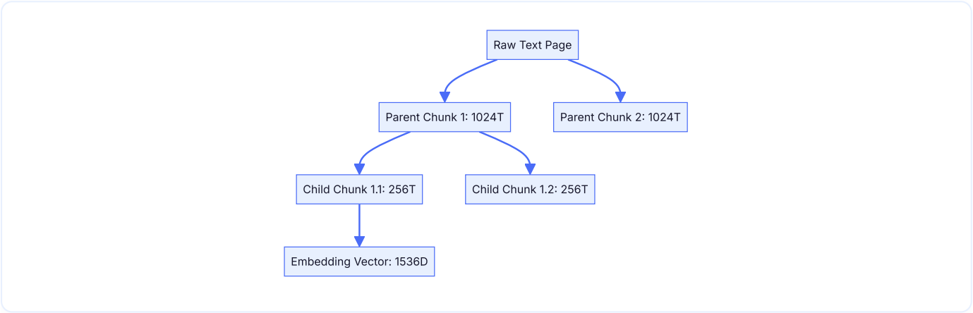
Figure 7.1: Parent-Child Chunking Layout. This diagram shows the relationship between parent chunks used for synthesis and child chunks embedded for vector similarity matching.
