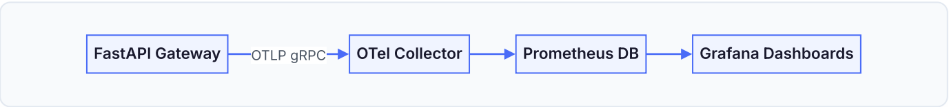
Figure 13.1: Proposed Telemetry Stack. This diagram shows the routing of API metrics through OTel collectors to dashboards.
