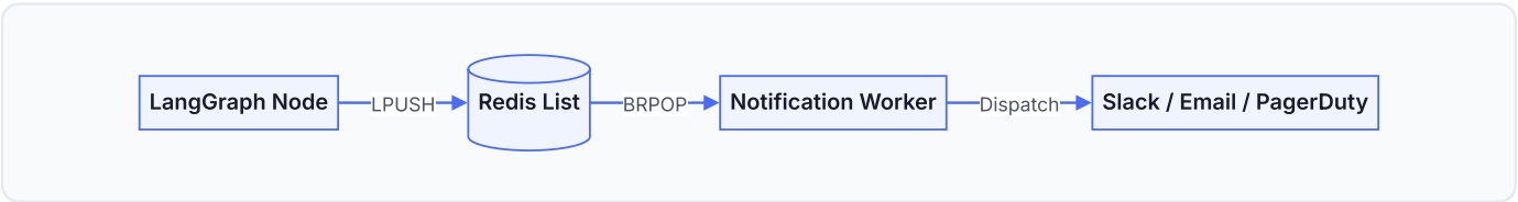
Figure 11.2: Proposed Redis Queue Workflow. This diagram illustrates the asynchronous dispatch flow utilizing Redis LPUSH/BRPOP operations.
