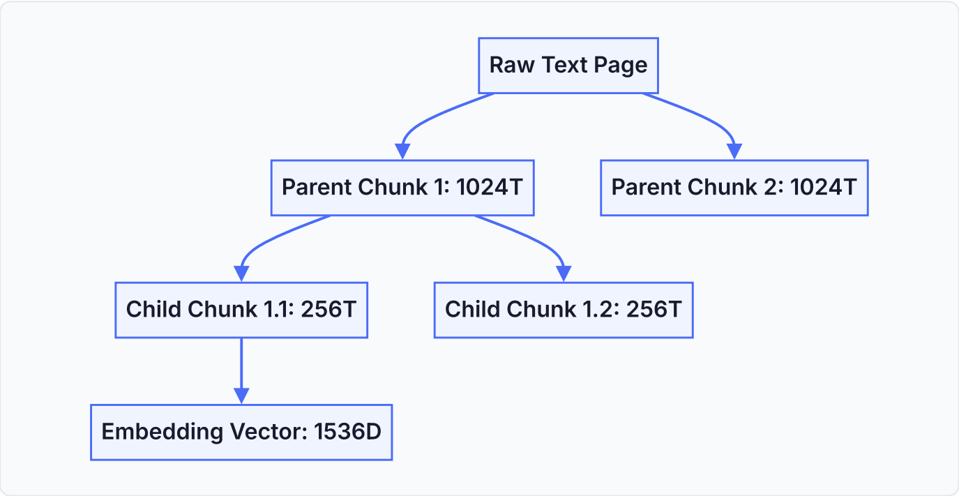
Figure 7.1: Parent-Child Chunking Layout. This diagram shows the relationship between parent chunks used for synthesis and child chunks embedded for vector similarity matching.
